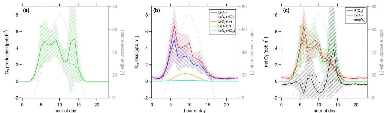
Figure 8. Diurnal profiles of (a) ozone production P(\text{O}_3) , (b) ozone loss L(\text{O}_3) and (c) ozone net terms during the CYPHEX campaign 2014. Solid lines show the hourly averaged \text{O}_3 production and loss terms based on the point-by-point calculation of simultaneous parameter measurements. The uncertainty from the atmospheric variability is represented by the 1\sigma error shades. For the dashed lines, all measurement parameters were averaged first, followed by the calculation of hourly \text{O}_3 production and loss terms. The uncertainty is mostly dominated by the atmospheric variability of all parameters and exemplarily shown by the error bar for one point for each production and loss term. Please find the temporal development of production and loss terms throughout the campaign in Figure S8 of the Supplement.
