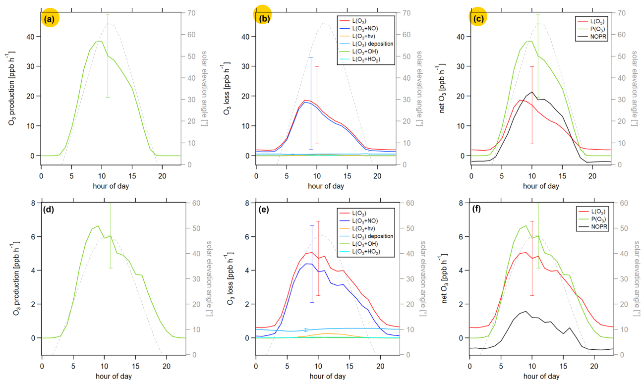
Figure 10. Diurnal profiles of O_3 production P(O_3) and loss L(O_3) terms during the HOPE campaign 2012 (top row: (a) P(O_3) , (b) L(O_3) and (c) net O_3 ) and the HUMPPA campaign 2010 (bottom row: (d) P(O_3) , (e) L(O_3) and (f) net O_3 ).
