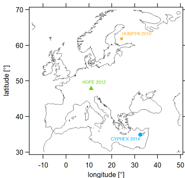
Figure 3. Geographic locations of the measurement sites included in this analysis. CYPHEX: 34.96 °N, 32.38 °E, 650 m a.s.l. (above sea level), UTC + 128 min (mean local time); HOPE: 47.80 °N, 11.01 °E, 980 m a.s.l., UTC + 44 min; HUMPPA: 61.85°N, 24.28°E, 181 m a.s.l., UTC + 96 min.
