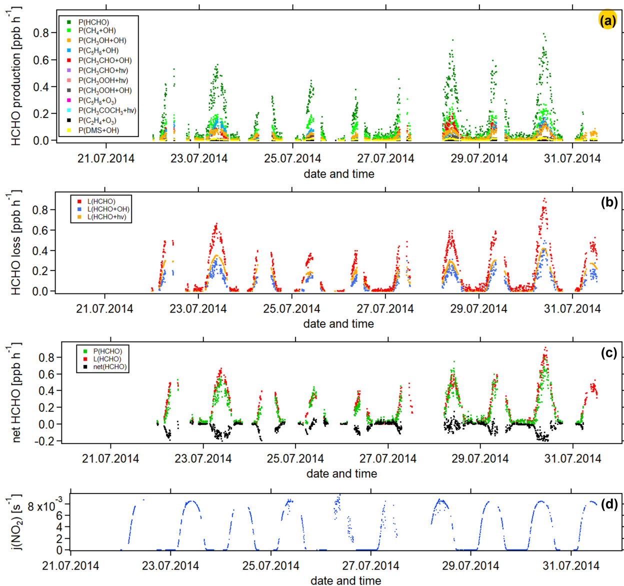
Figure 5. Temporal development of (a) HCHO production terms, (b) HCHO loss terms and (c) net HCHO from July 22 to July 31, 2014 during the research campaign CYPHEX in Cyprus. The \text{NO}_2 photolysis frequency j(\text{NO}_2) is shown in (d) as illustration of the diurnal cycle. All times are in UTC.
