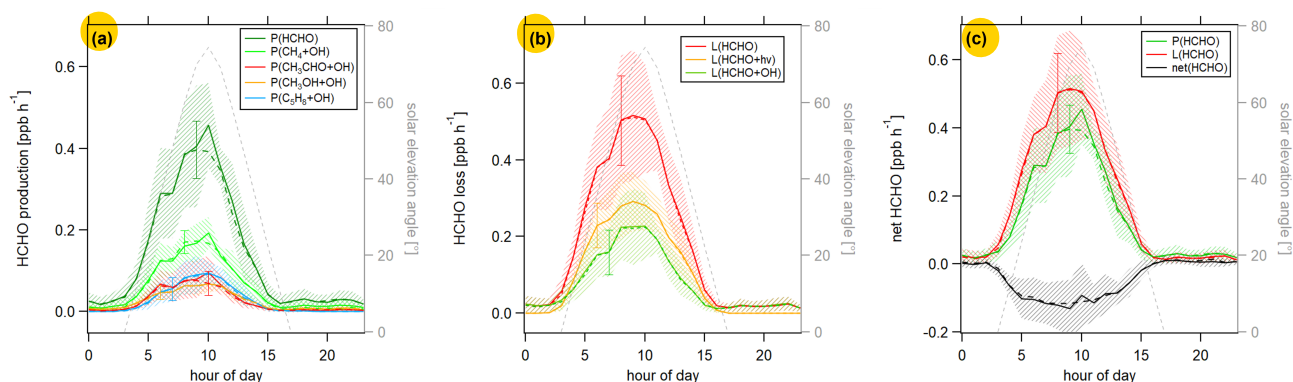
Figure 7. Diurnal profiles of (a) HCHO production P(\text{HCHO}) , (b) HCHO loss L(\text{HCHO}) and (c) HCHO net terms during the CYPHEX campaign 2014. Solid lines show the hourly averaged HCHO production and loss terms based on the point-by-point calculation of simultaneous parameter measurements. The uncertainty from the atmospheric variability is represented by the 1\sigma error shades. For the dashed lines, all measurement parameters were averaged first, followed by the calculation of hourly HCHO production and loss terms. The uncertainty is based on the atmospheric variability of all parameters and exemplarily shown by the error bar for one point for each production and loss term. The gray dashed line represents the diurnal solar elevation angle at the measurement site as determined by help of the NOAA Solar Calculator (2021).
