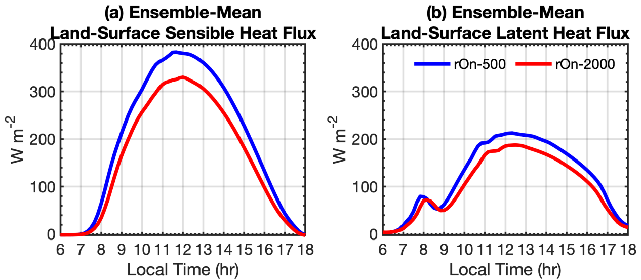
Figure 4. Time series of the ensemble-mean land surface (a) sensible heat flux and (b) latent heat flux, spatially averaged from western domain edge to the 50 km ahead of the algorithm-identified sea breeze front, for the rOn-500 (blue) and rOn-2000 ensembles (red).
