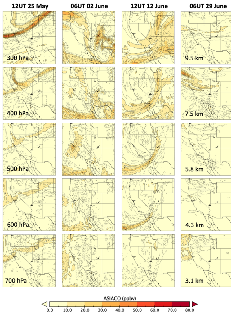
540 Figure 10: Same as Fig. 9, but for the ASIACO tracer.
