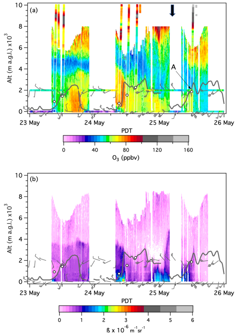
555 Figure 11: Time-height curtain plots similar to those in Figures 4 and 5, but expanded to better show the TOPAZ (a) ozone and (b) backscatter measurements during IOP1. The dark gray curves represent the boundary layer heights derived from the co-located Doppler lidar measurements. The superimposed horizontal bands in (a) show the AP and NLVA in-situ O_3 measurements and the near-vertical colored bands show the Joe Neal ozonesonde profiles. The bars in both panels show the AP and NLVA surface winds and the open circles the mixing heights inferred from the ozonesondes. The heavy black arrow above (a) corresponds to the 12UT 25 May PV plot from Figure 3b. The 300 hPa surface lies at approximately 9 km a.g.l. The label “A” is the same as in Figure 6.
