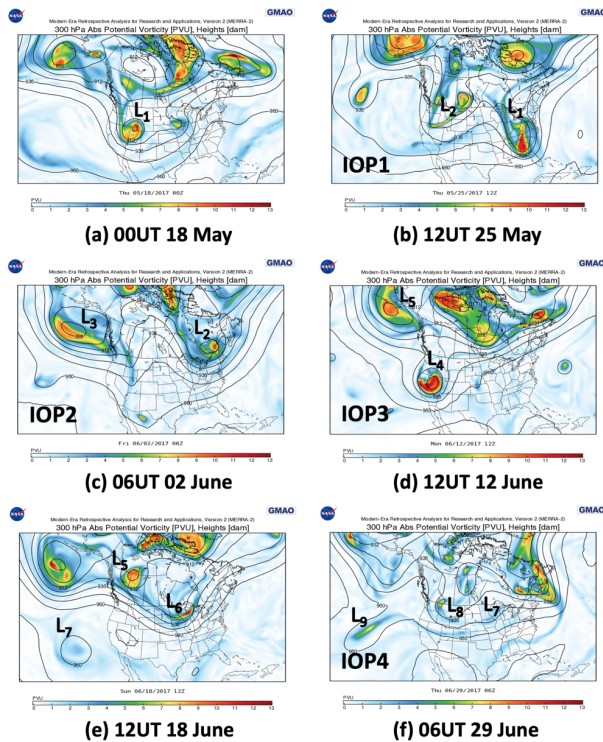
635 Figure 3: MERRA-2 300 hPa Absolute potential vorticity and geopotential heights (dam) at (a) 00UT 18 May, (b) 12UT 25 May, (c) 06UT 02 June, (d) 12UT 12 June, (e) 12UT 18 June, and (f) 06UT 29 June.
