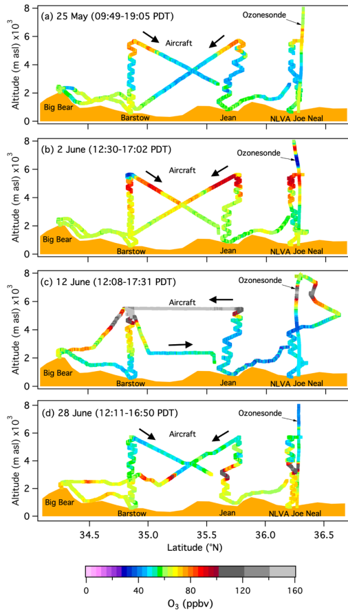
1055 Figure 16: Ozone mixing ratios measured by the ozonesonde and aircraft on the flights to and from Big Bear on: (a) 25 May, (b) 2 June, (c) 12 June, and (d) 28 June. The TOPAZ measurements and \Delta P aircraft profiles are omitted for clarity, as are the Jean and NLVA aircraft profiles from the return legs. The terrain profile is approximate.
