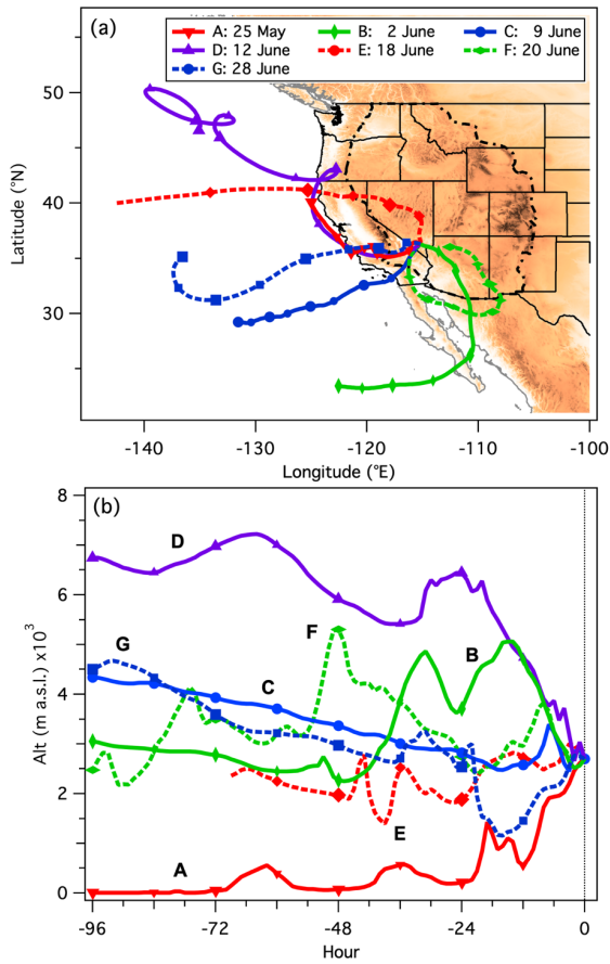
1065 Figure 18: NOAA HYSPLIT 96-h back trajectories launched 2 km above North Las Vegas during episodes A-G. The small and large filled symbols are spaced at 12 and 24 hours apart, respectively. The trajectories were calculated using the 40 km NCEP Eta Data Assimilation System (EDAS) meteorology.
