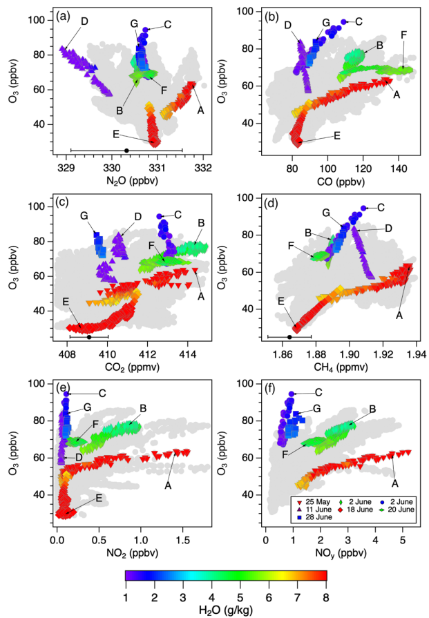
1060 | Figure 17: Scatter plots showing the relationships between O 3 and the (a) N 2 O, (b) CO, (c) CO 2 , (d) CH 4 , (e) NO 2 , and (f) NO y tracers on AP during episodes A-G. The grey points show all of the F457-LVOS measurements. The black points with error bars in (a), (c), and (d) represent the mean (±1σ) June 2017 concentrations from the NOAA GML Mauna Loa Observatory.
