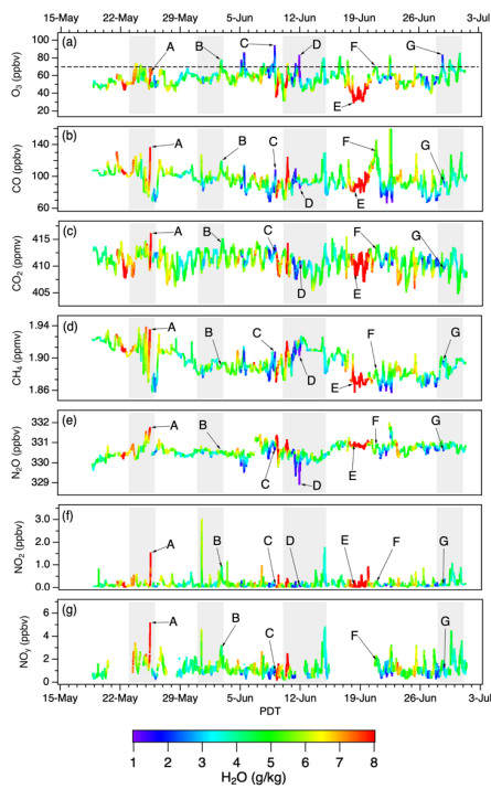
700 Figure 6: Time series of the AP 1-min in-situ measurements color-coded by the co-measured H 2 O. The dashed black line in (a) shows the 2015 NAAQS of 70 ppbv. The gray regions bracket the four IOPs. The measurements labelled A-G are discussed in the text.
