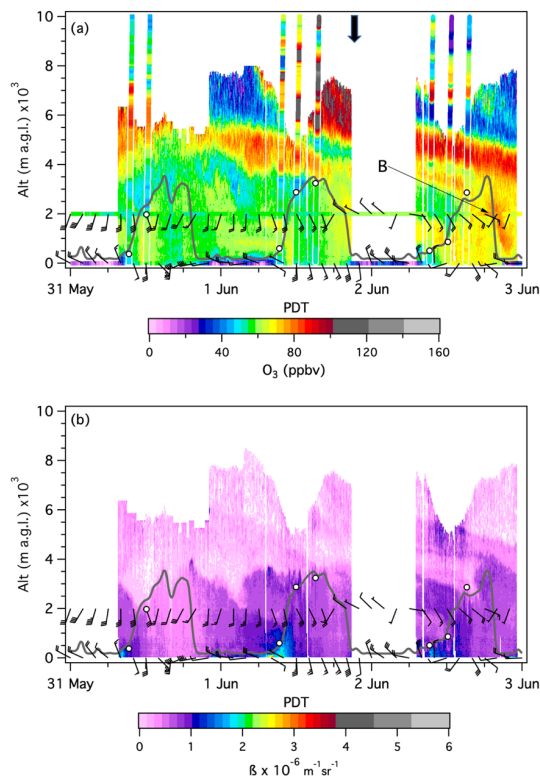
930 Figure 12: Same as Figure 11, but for IOP2. The heavy black arrow corresponds to the 06UT 2 June 300 hPa plot in Figure 3c.
