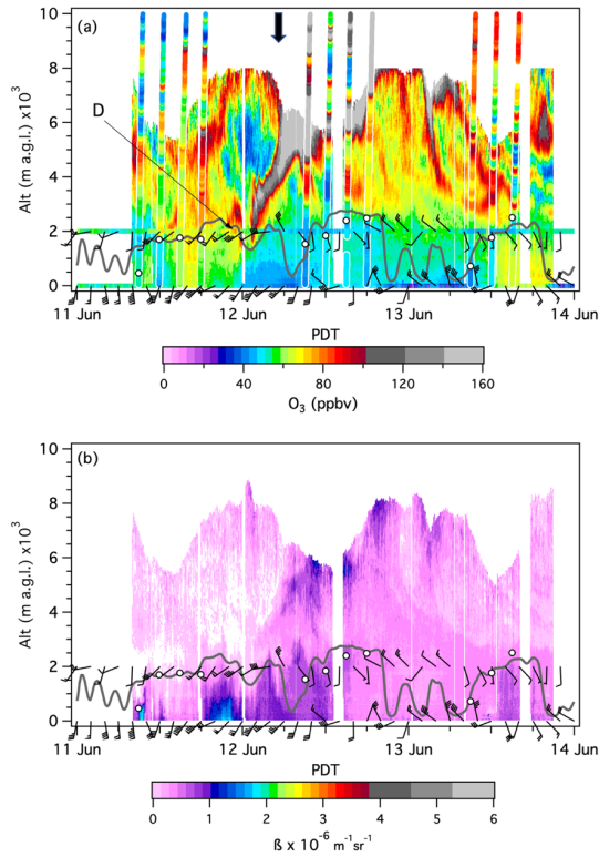
980 Figure 13: Same as Figure 11, but for IOP3. The heavy black arrow corresponds to the 12UT 12 June 300 hPa plot in Figure 3d.
