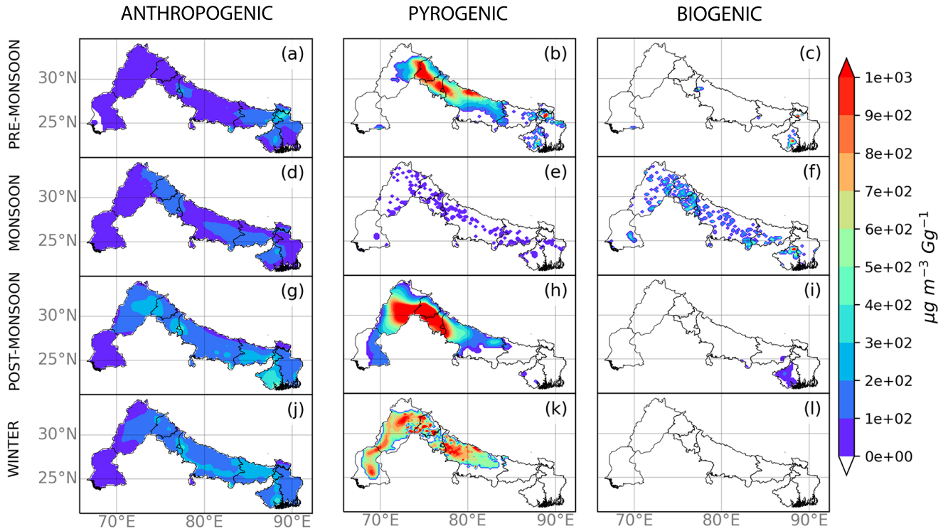
Figure 4. Seasonal sensitivity of \text{PM}_{2.5} concentrations to changes in (left column) anthropogenic, (middle column) pyrogenic, and (right column) biogenic emissions ( \mu\text{g m}^{-3}\text{Gg}^{-1} ). The calculation is described in the main text. Regions marked as white denote where sensitivity corresponds to \text{PM}_{2.5} concentrations below the set threshold of 4 \mu\text{g m}^{-3} .
