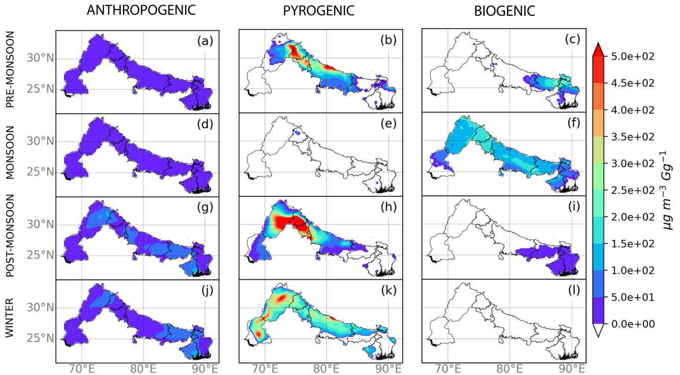
Figure 7. Seasonal sensitivity of total OA to changes in (left column) anthropogenic, (middle column) pyrogenic, and (right column) biogenic emissions ( \mu \text{ g m}^{-3} \text{ Gg}^{-1} ). The sensitivity calculation is described in the main text. Regions marked as white shows where sensitivity corresponds to OA concentrations below the set threshold of 1 \mu \text{ g m}^{-3} .
