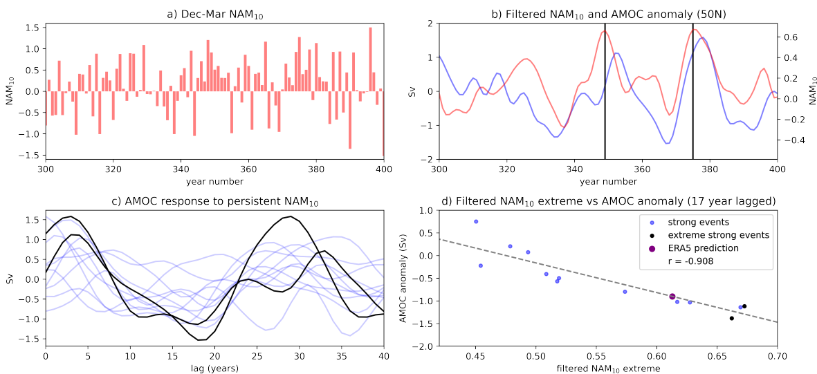
Figure 11. a: Dec-Mar NAM_{10} index (red bars) from the UKESM simulation between year numbers 300 and 400. b: AMOC (blue) and NAM_{10} (red) indices smoothed with the Gaussian filter ( \sigma = 2 years) between year numbers 300 and 400 of the UKESM simulation. Black vertical lines show the location of the largest smoothed NAM_{10} . c: AMOC response to persistent strong NAM_{10} intervals. Light blue lines denote lagged AMOC responses of the AMOC from the whole UKESM simulation, black lines show AMOC responses to NAM_{10} intervals marked in b by vertical black lines. d: Scatter plot of filtered NAM_{10} index values occurring at persistent strong NAM_{10} intervals throughout the whole UKESM simulation ( y -axis) against AMOC anomalies at 50N lagged 17 years after persistent intervals' central year ( x -axis). Blue points indicate persistent intervals and black dots represent the 2 intervals displayed in b . The dotted line represents the linear line of best fit for the points in black and blue. Also included is the 17-year lag AMOC anomaly predicted by projecting the regression coefficients used to construct the linear fit onto the maximum smoothed NAM_{10} index in the ERA5 dataset (purple point).
