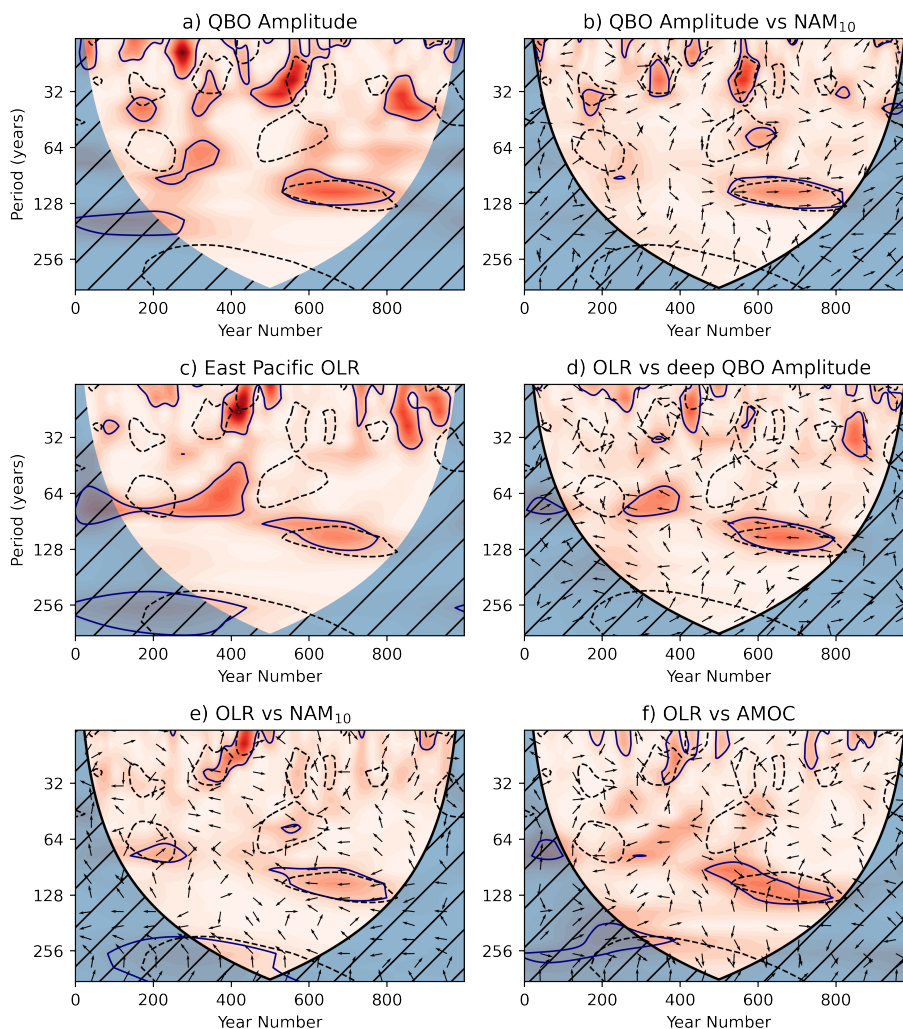
Figure 9. (a): Wavelet power spectrum for the Sep-Nov deep QBO amplitude (see section 2.4). (b) cross power spectra between deep QBO Amplitude (Sep-Nov) and smoothed NAM 10 (Dec-Mar). (c): Wavelet power spectrum for the Sep-Nov Area weighted average equatorial East Pacific OLR (see section 2.4). d-f : cross power spectra between combinations of East Pacific OLR, deep QBO Amplitude (both Sep-Nov means), AMOC at 50N (annual mean, all months) and NAM 10 (Dec-Mar) indices all smoothed with the same Gaussian filter as is used throughout ( \sigma = 2years ). Indices involved are indicated by the sub-figure titles. Shading indicates the cross power, using the same colour scale as in figures 6-8. Solid contours indicate the 95% confidence interval for the power spectrum and dashed contours show the 95% confidence interval for the NAM 10 spectrum, for ease of comparison. Arrows indicate the relative phase angle between the signals in the indices.
