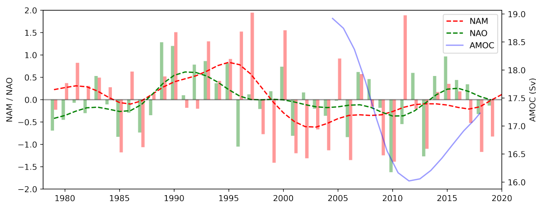
Figure 10. Time series of the Dec-Mar NAO index (green bars), NAM 10 index (red bars) from the ERA5 dataset. Dashed lines correspond to indices shown by bars smoothed with a Gaussian filter ( \sigma = 2 years). Also included is the annual AMOC time series at 26N from the rapid array dataset (blue).
