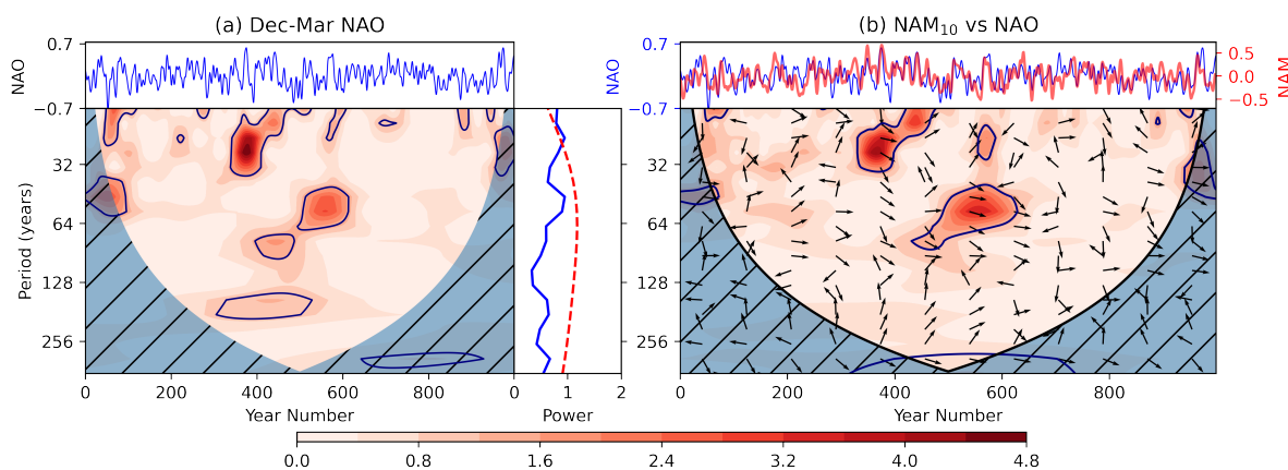
Figure 8. like figure 7 for the Dec-Mar NAO index. (a) shows the wavelet power spectrum of the NAO and (b) the cross power spectrum between the NAO and the NAM 10 index.
