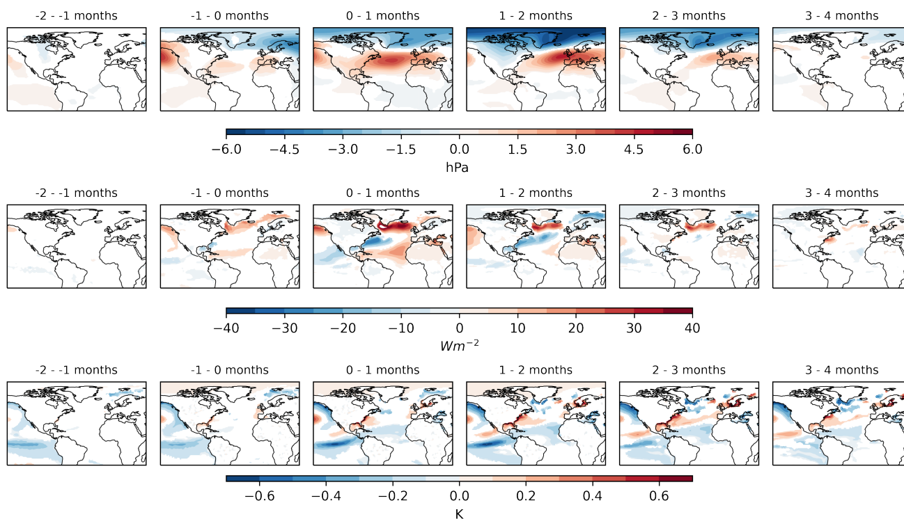
Figure 1. Surface patterns associated with anomalous winter stratospheric NAM 10 events. Top row: Monthly mean sea level pressure anomaly (hPa), middle row: Ocean-Atmosphere heat flux defined as the sum of latent and sensible heat fluxes ( wm^{-2} ) and bottom row: SSTs (K). Coloured shading shows where the composite differences between strong and weak NAM 10 events are statistically significant at the 95% level under a 2 tailed students t-test. The title of each sub-figure indicates the month range relative to the central date of each NAM 10 anomaly. Signals at negative times indicate that the surface anomaly leads the stratospheric NAM 10 anomaly. Signals at positive times indicate that the stratospheric NAM 10 anomaly leads the surface response.
