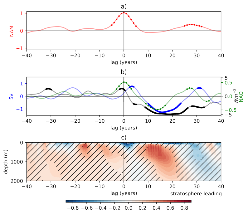
Figure 4. a: Composite differences of the smoothed NAM_{10} index around extreme NAM_{10} intervals (positive - negative intervals). b: Like figure 3f for the AMOC at 50N (blue), the Dec-Mar mean NAO index and the ocean-atmosphere heat flux (sum of latent and sensible fluxes) averaged over an Atlantic box defined by 45^{\circ} – 65^{\circ} N, 15^{\circ} – 60^{\circ} W. All indices are smoothed with a Gaussian filter ( \sigma = 2 years). c: lagged responses of ocean temperature anomaly depth profiles to persistent NAM_{10} intervals. Composite differences between strong and weak intervals are shown for the same Atlantic box as the heat flux index. Hatching indicates composite differences that are not significant at the 95% level under a 2-tailed student's t-test.
