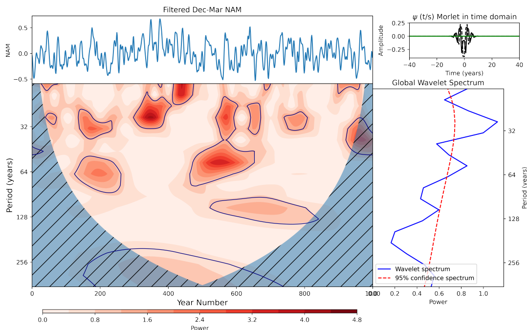
Figure 6. Top left: Dec-Mar NAM 10 values smoothed with a Gaussian filter ( \sigma = 2 years). Bottom left: Wavelet power spectrum of time series in the top left sub-figure. Hatching represents areas outside the cone of influence in which edge effects are significant and power should not be considered. blue contours represent the 95% confidence level assuming mean background AR1 red noise. Top Right: Morlet wavelet used for the wavelet transform in the time domain. Bottom right: Global power spectrum, the wavelet power averaged over the whole simulation (blue line), and global 95% confidence spectrum (red dashed line).
