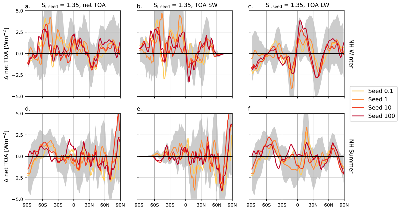
Figure 11. Five-year annual global 1.35-seeding zonal mean radiative balance anomalies in \text{Wm}^{-2} for all seeding particle concentrations for the net TOA (a,d) and the TOA SW (b,e) anomaly profiles in \text{mg/m}^3 as in, but and TOA LW (c,f). The top row shows the four-year zonal mean for NH winter (December - February) and the bottom row is the five-year zonal mean for NH summer (June - August). The grey shaded area is the 95% confidence interval around the mean Seed1 anomaly, representing the two-times standard deviation interval, based on the variance of the annual data.
