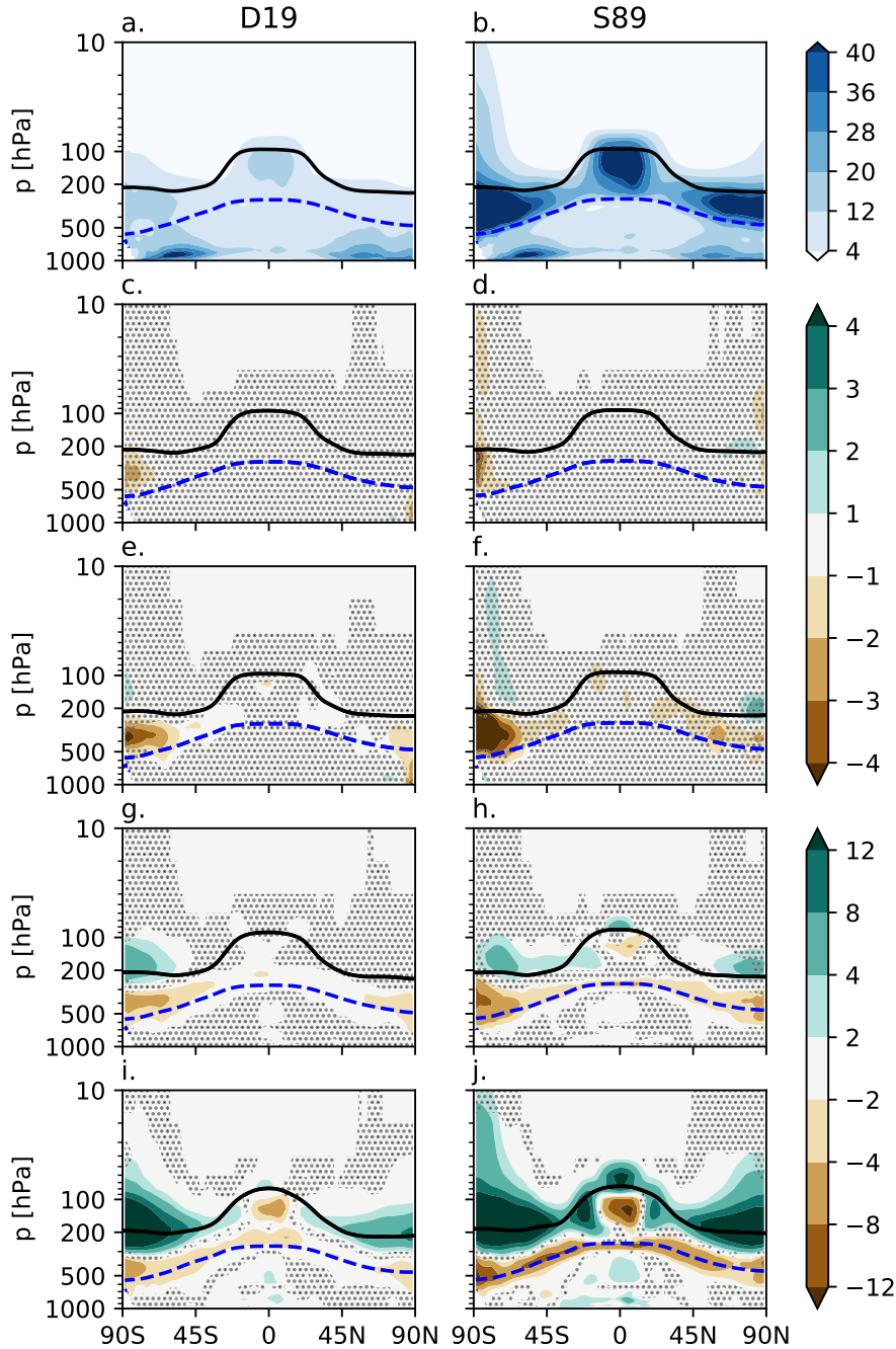
Figure 4. Five-year zonal mean cloud fractions [0-1%] on pressure levels [hPa] for D19 and S89 ice-cloud fraction approaches for the unseeded reference cases (a-b). The cloud fraction anomalies respective to the unseeded reference cases are plotted in the subsequent rows for S_{i,seed} = 1.05 : Seed0.1 (c-d), Seed1 (e-f), Seed10 (g-h), and Seed100 (i-j). The black line is the five-year mean zonal mean WMO-defined tropopause height on pressure levels, and the blue dashed line is the 238 K isotherm. The stippling in the difference plots shows insignificant data points on the 95% confidence level according to the independent t-test controlled by the "false discovery rate" method.
