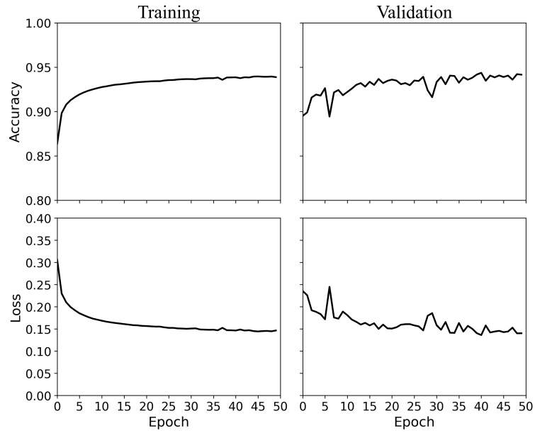
Figure 3. Training (left panels) and validation (right panels) accuracy and loss trajectories.
