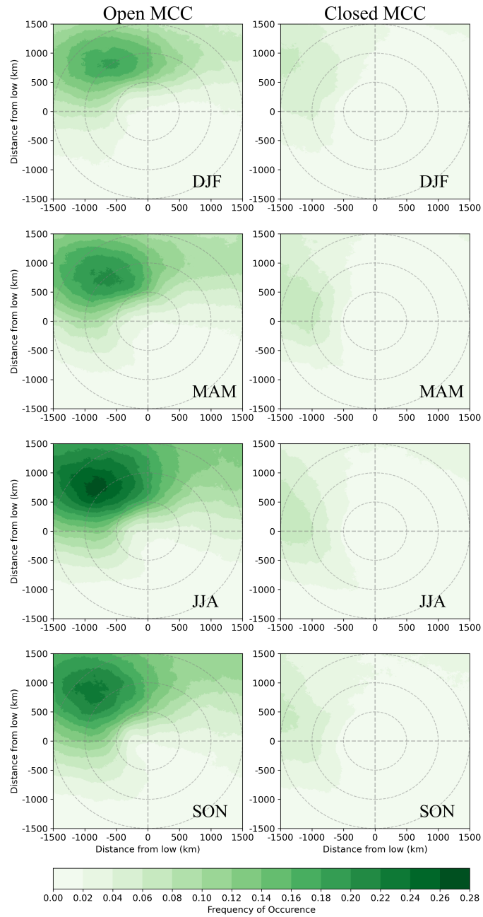
Figure 10. Seasonal distribution of open and closed MCC in the context of the composite extra-tropical cyclones. Shown are open MCC (left) and closed MCC (right). Seasonal means are shown for winter (DJF), spring (MAM), summer (JJA) and fall (SON). Concentric circles indicate distances of 500, 1000, and 1500 km from cyclone center.
