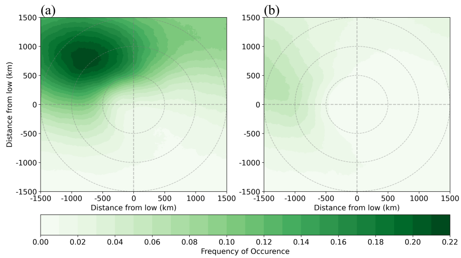
Figure 9. Distribution of open and closed MCC in the context of the composite extra-tropical cyclones. Concentric circles indicate distances of 500, 1000, and 1500 km from cyclone center.
