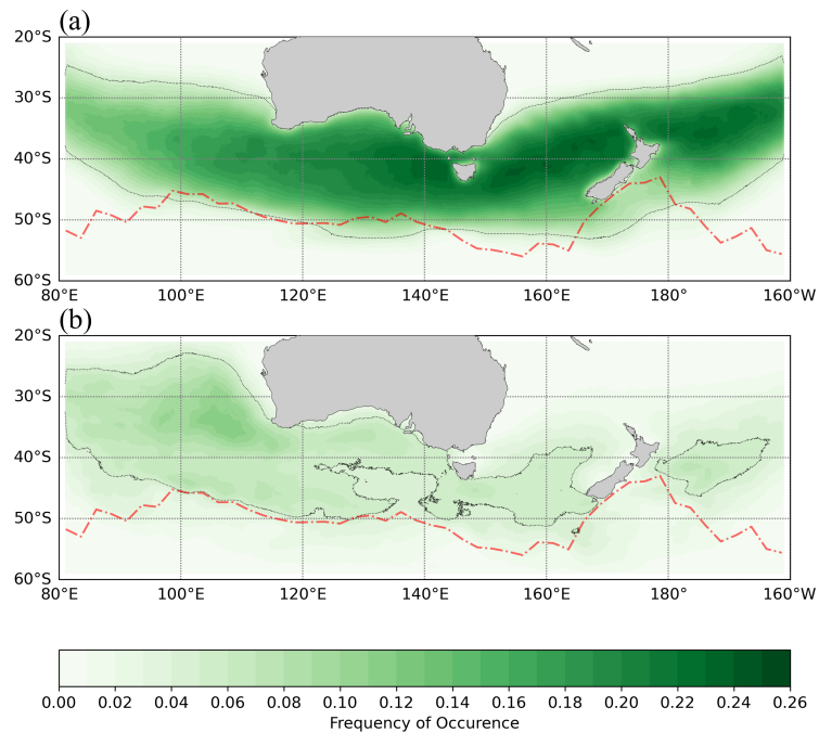
Figure 6. Distribution of the frequency of occurrence of MCC cloud type for the period 2016-2018. (a) Open MCC and (b) closed MCC. Red lines indicate the position of the polar front derived from ERA5 SST gradients. Dotted black lines shows the contour level 0.05%.
