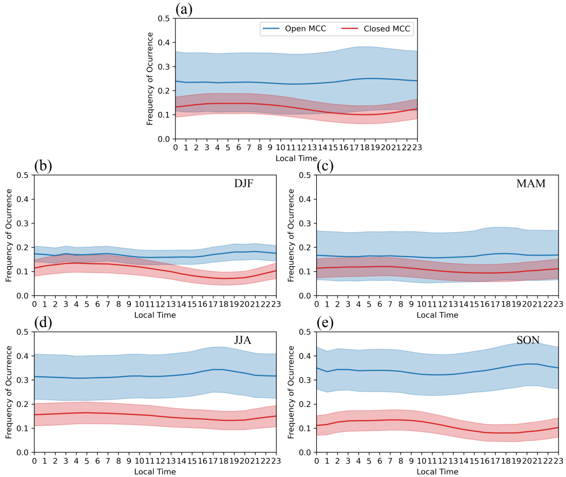
Figure 8. Diurnal cycle of the frequency of occurrence of MCC types for the period 2016-2018. Shown are open MCC (blue) and closed MCC (red). Seasonal means are shown for summer (DJF), autumn (MAM), winter (JJA) and spring (SON). Shadings represent one standard deviation. Frequencies are calculated for the latitudinal band between 40^{\circ} and 50^{\circ} .
