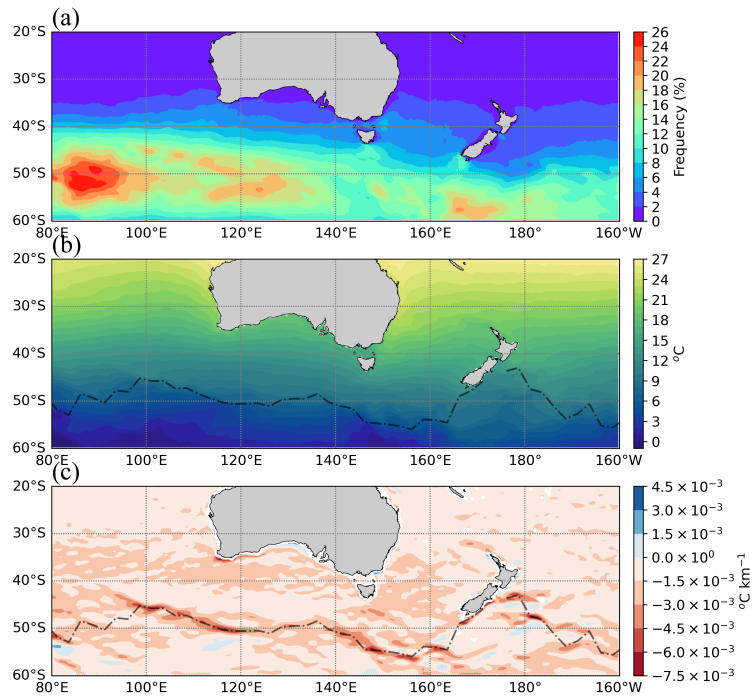
Figure 4. (a) Frequency (%) of 10-m winds exceeding 15 \text{ m s}^{-1} from ERA5, (b) mean SST from ERA5 reanalysis and the corresponding (c) SST gradient. Period between 2016 and 2018. Black lines indicate the position of the polar front derived from ERA5 SST gradients.
