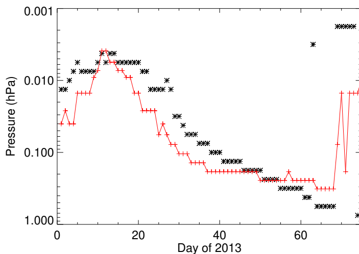
Figure 2. The pressure level of the nitric oxide 50 ppbv value (bottom side of the layer). The pluses connected by a red line are daily values of the WACCMX results shown in Figure 1. The black stars are the SOFIE data from Figure 1.
