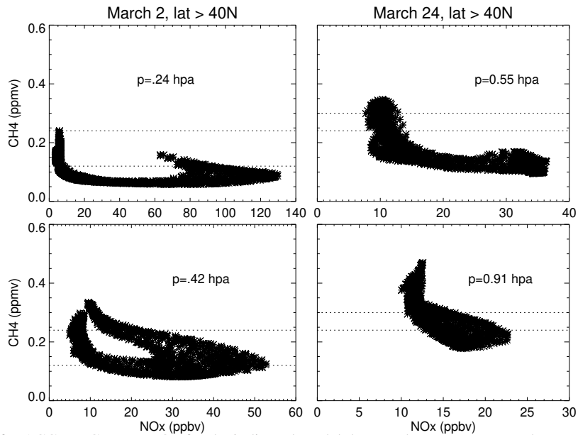
Figure 12. Scatter plot of WACCMX CH 4 vs. NO x for the indicated model dates and pressures. Note, the vertical range for CH 4 is the same for all 4 panels, but the horizontal ranges for NO x differ and are labeled separately for each panel. The horizontal dotted lines in each panel are CH 4 thresholds that are used to identify MLT NO x ; see text for discussion.
