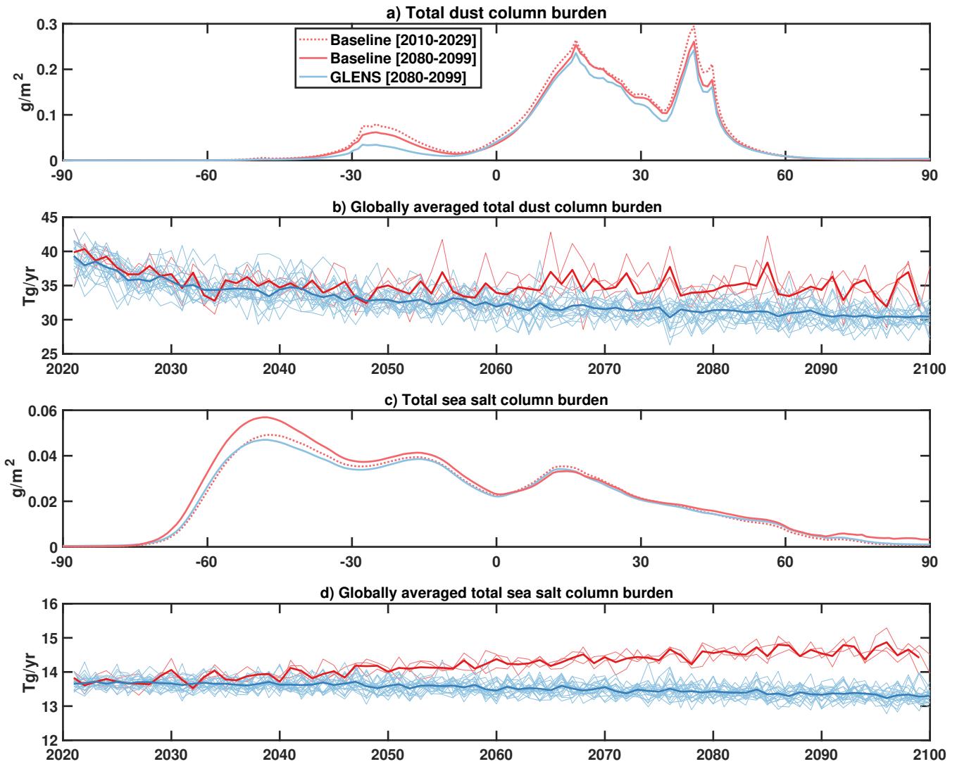
Figure 2. Zonally averaged total column burden of dust (a) and sea salt (c) (considering all modes) in 2010-2029 (red, dashed line), 2080-2099 in Baseline (red line) and 2080-2099 in GLENS (blue line). Evolution of the globally integrated dust (b) and sea salt (d) burden ( Tg/yr ). Lighter lines show the single ensemble realizations, while the thicker lines show the ensemble mean.
