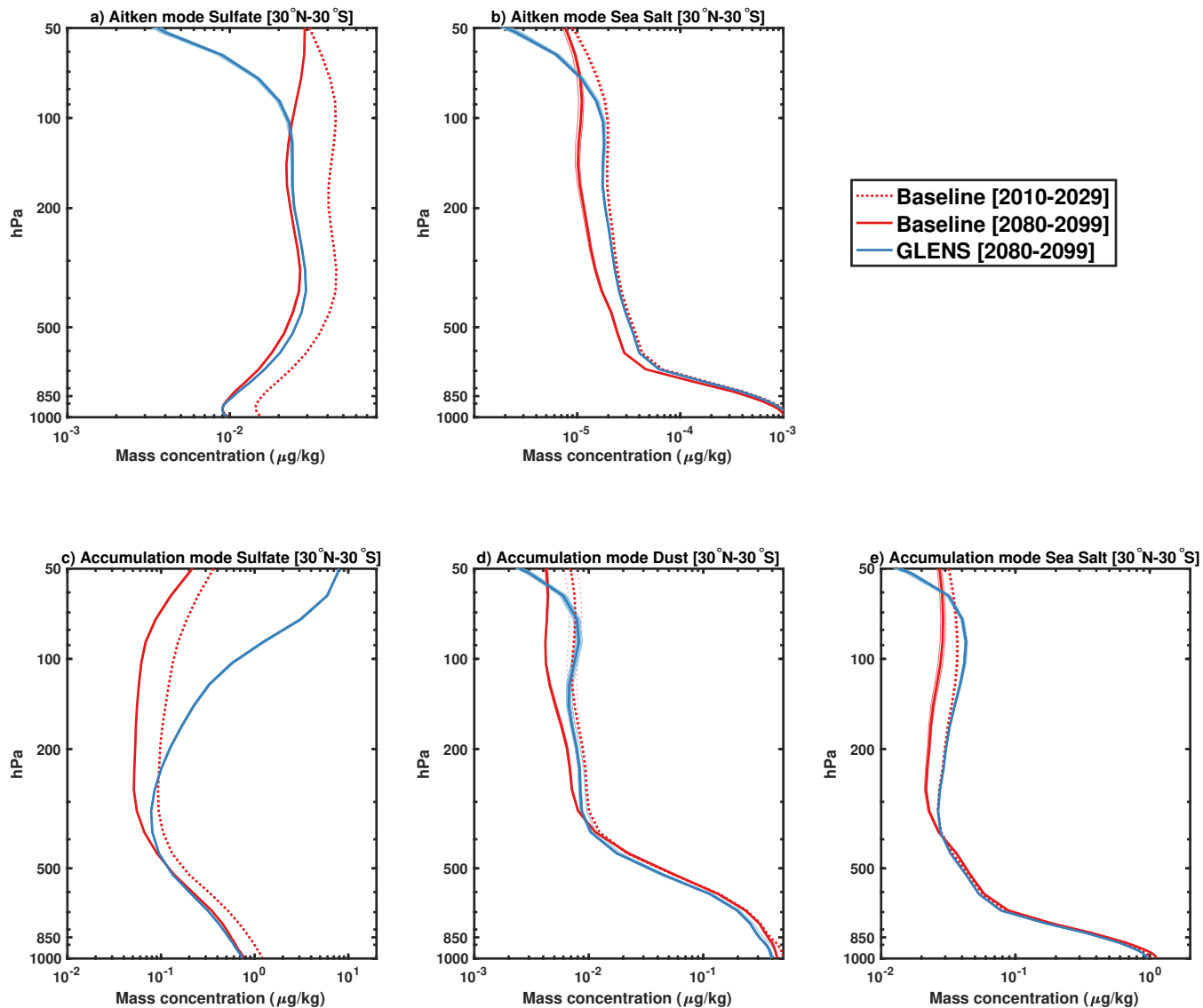
Figure 3. Mass concentration (in \mu\text{g} per kg of air) of Sulfate, Dust and Sea Salt in the Aitken (smallest) and Accumulation (intermediate) mode, between 30°N and 30°S. Lighter lines show the single ensemble realizations, while the thicker lines show the ensemble mean.
