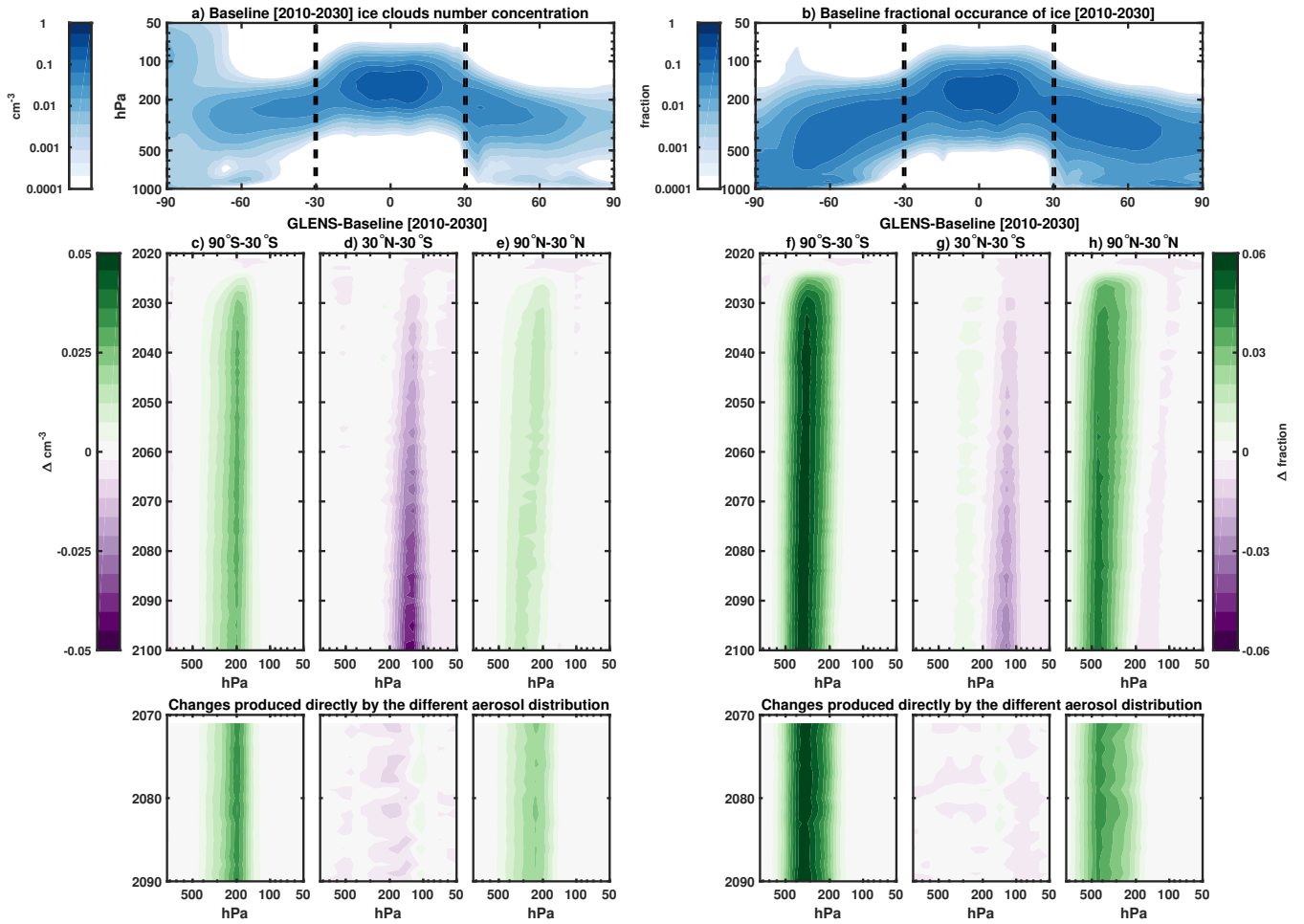
Figure 5. Baseline concentration of cloud ice number concentration (a, number of particles per \text{cm}^{-3} ) and fractional occurrence (b) in the period 2010-2030. In the panels c-e) and f-h), the yearly evolution of the differences between GLENS and Baseline (in the 2010-2030 period, as for the panels above) are shown for the three latitudinal boxes separately. In the small panels below, the effect of the changes produced by the aerosols are isolated by plotting the difference between GLENS and the simulations with surface cooling and stratospheric heating but no aerosols.
