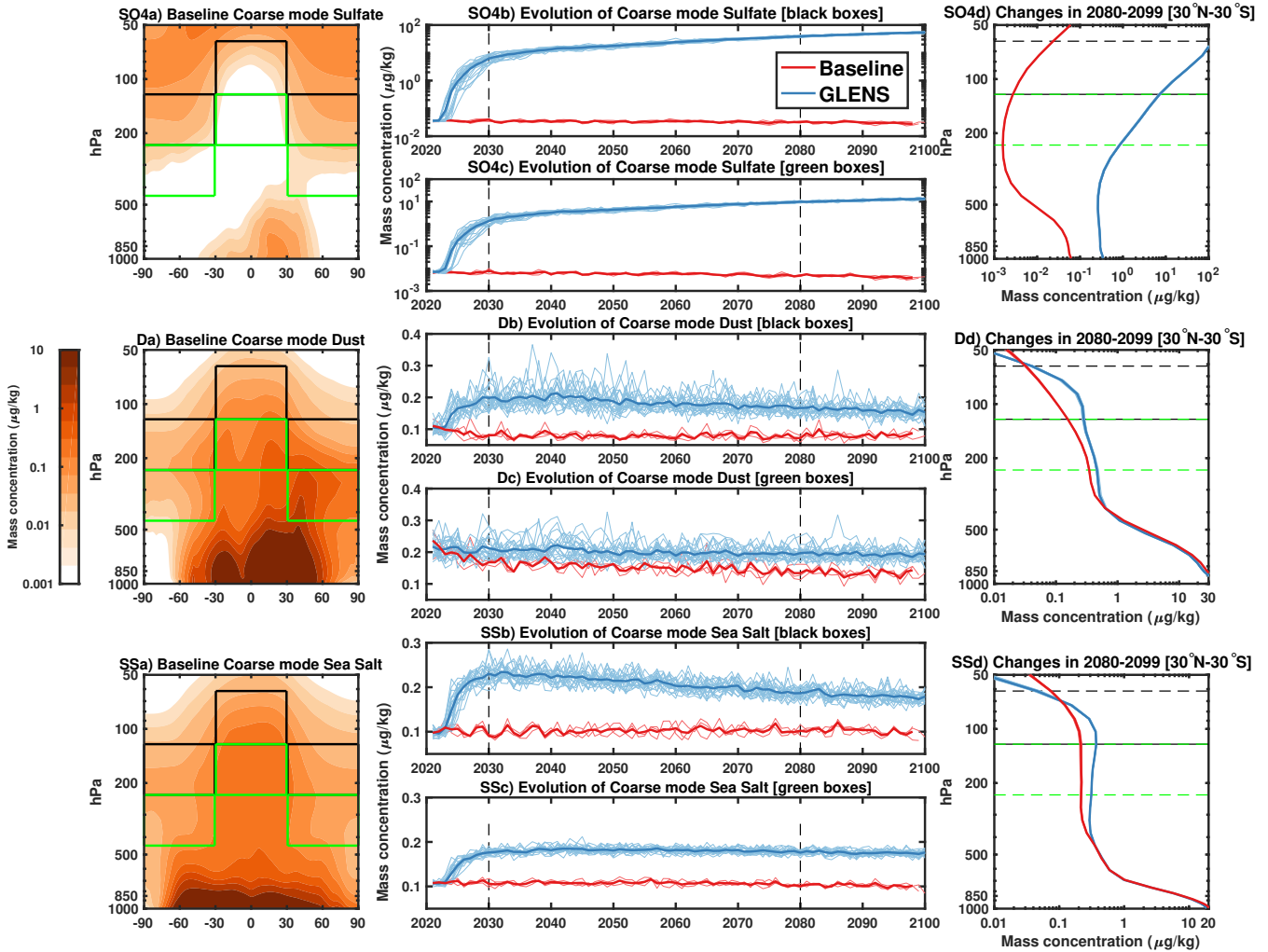
Figure 1. Mass concentration (in \mu\text{g} per kg of air) of Coarse mode species (Sulfate (SO4), Dust (D) and Sea Salt (SS), from top to bottom). On the left, panels a) indicate the Baseline (2020-2029) zonal mean concentration for the respective species, with the black box and green boxes indicating the area-areas considered in the average-averages for the central panels -, where (panels b and c). The uppermost limit of the green boxes and the lowermost limit of the black boxes coincide. Panels b) and c) for each species show the annual mean-evolution for both cases is shown. Lighter of the concentration in the black (panels b) and green (panels c) boxes, with lighter lines show showing the single ensemble realizations, while and the thicker lines show the ensemble mean; red lines indicate the Baseline simulations, while blue lines indicate the GLENS simulations. On the right, panels c) show the vertical profile-profiles in both cases (Baseline, in red, and GLENS, in blue) for the same latitudinal band is shown period 2080-2099. Black dashed lines in the central-c) and d) panels indicate the periods of analyses for the left-a) and right-d) panels, respectively; the same lines in the right-d) panels indicate the altitude of analyses in the central-b) and c) panels.
