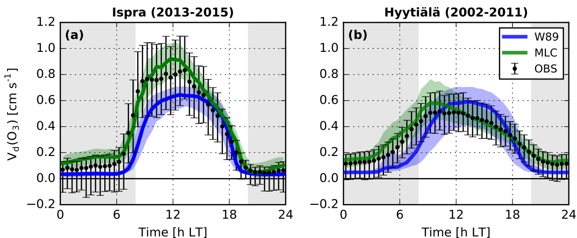
Figure 4. Diurnal cycles of April-September ozone dry deposition velocity at Ispra (panel a) and Hyttiälä (b), derived from observations (black), and simulations with the W89 parameterization (blue) and MLC-CHEM (green). Lines and points show median values, and shaded areas and whiskers display the inter-quartile range.
