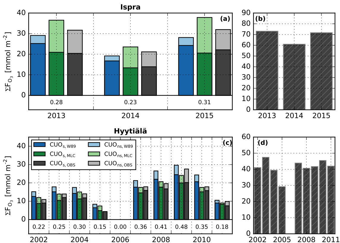
Figure 8. Panels a,c: growing season-integrated daytime (8–20 h LT) stomatal (CUO st ; dark colours) and non-stomatal (CUO ns ; light colours) ozone fluxes for the different years in the study period, for Ispra (panel a) and Hyttiälä (panel c). Results from the W89 parameterization are shown in blue, from MLC-CHEM in green and from observations in grey. Only the data points with valid observation-inferred stomatal conductance estimates are selected for this comparison, the fraction of valid data points per growing season that remains is shown in the bottom of the figure. Panels b,d: inferred cumulative stomatal ozone uptake (CUO) estimate at both sites (hatched bars) after dividing the season-integrated daytime stomatal ozone flux (dark grey bars) by the fraction of valid data points. Note the different y axis ranges in the four panels.
