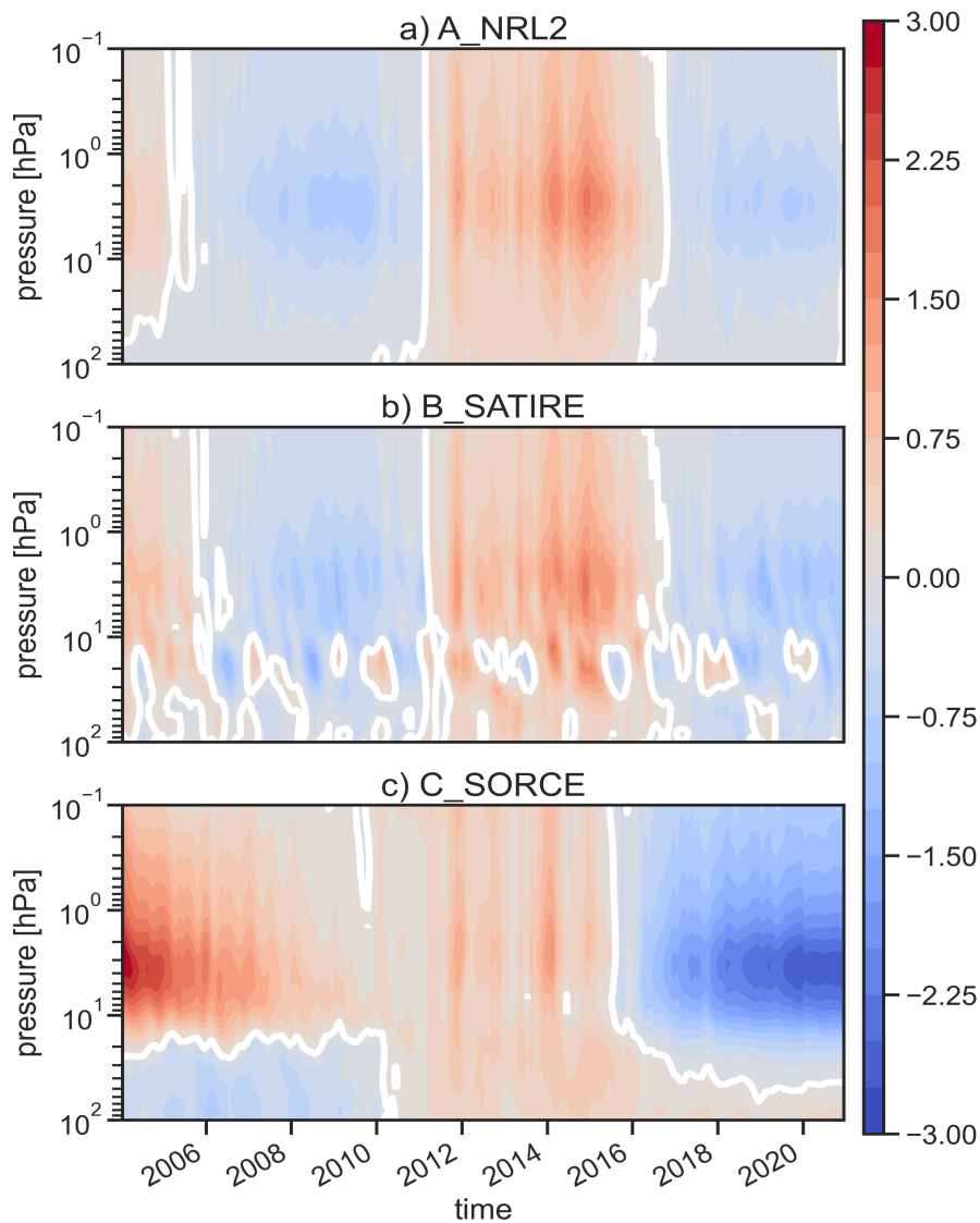
Figure 7. Percentage difference in tropical ozone (20°N–20°S) between a model simulation with time-varying solar flux and a simulation with fixed solar flux for (a) NRL2, (b) SATIRE and (c) SORCE. White-coloured lines show zero contours.
