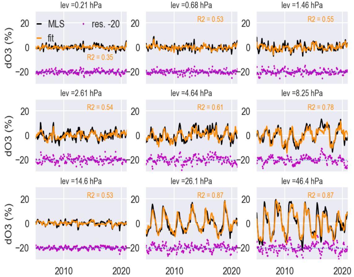
Figure 1. Monthly mean ozone anomalies from MLS V5 (black line) for 2005-2020 and corresponding regression fits (orange line) for nine different pressure levels at 1.5°N. Corresponding Goodness of fit ( R^2 ) values are also shown with dark-orange-coloured text and residuals are shown at the bottom of each panel (as pink dots). For clarity the residuals are shifted by -20%.
