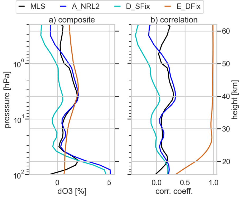
Figure 4. (a) MLS ozone profile composite for solar maxima ( n=40 ) and solar minima ( n=51 ) months (black line). Percentage ozone differences for the tropics ( 20^\circ\text{N} – 20^\circ\text{S} ) between a model simulation with time-varying NRL2 solar flux (A_NRL), fixed solar flux (D_SFfix) and fixed dynamics (E_DFfix) simulations are shown with blue, cyan and orange lines, respectively. (b) Correlation coefficient between Mg-ii index and monthly mean ozone anomalies from MLS and simulations A_NRL, D_SFfix and E_DFfix.
