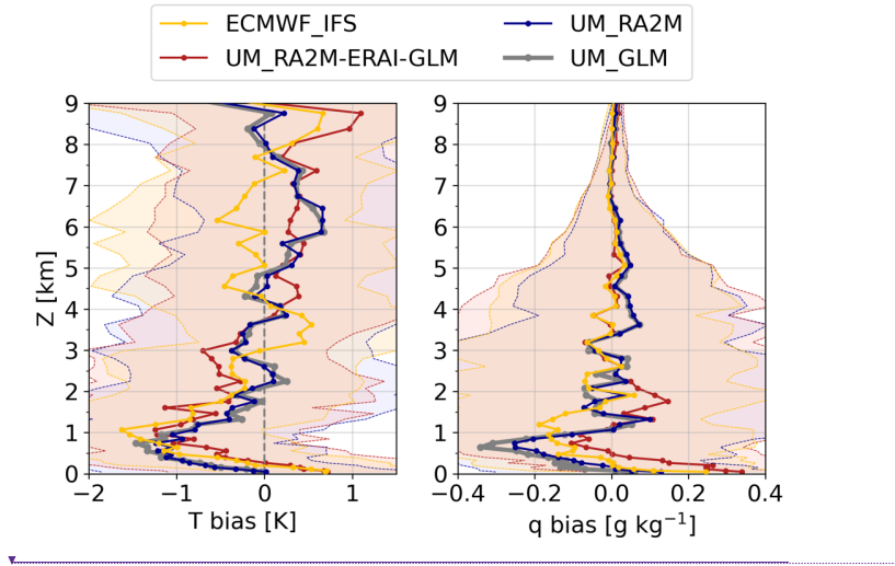
Figure 11: Median T (left) and q (right) biases from a subset of the drift (31 Aug to 5 Sep) for ECMWF IFS (yellow), UM_RA2M-ERA1-GLM (red), UM_RA2M (dark blue), and UM_GLM (grey). UM_RA2M-ERA1-GLM biases follow ECMWF_IFS biases up to approximately 1 km, above which they largely behave more like the other UM cases. \pm one standard deviation shown in shading to illustrate variability.
