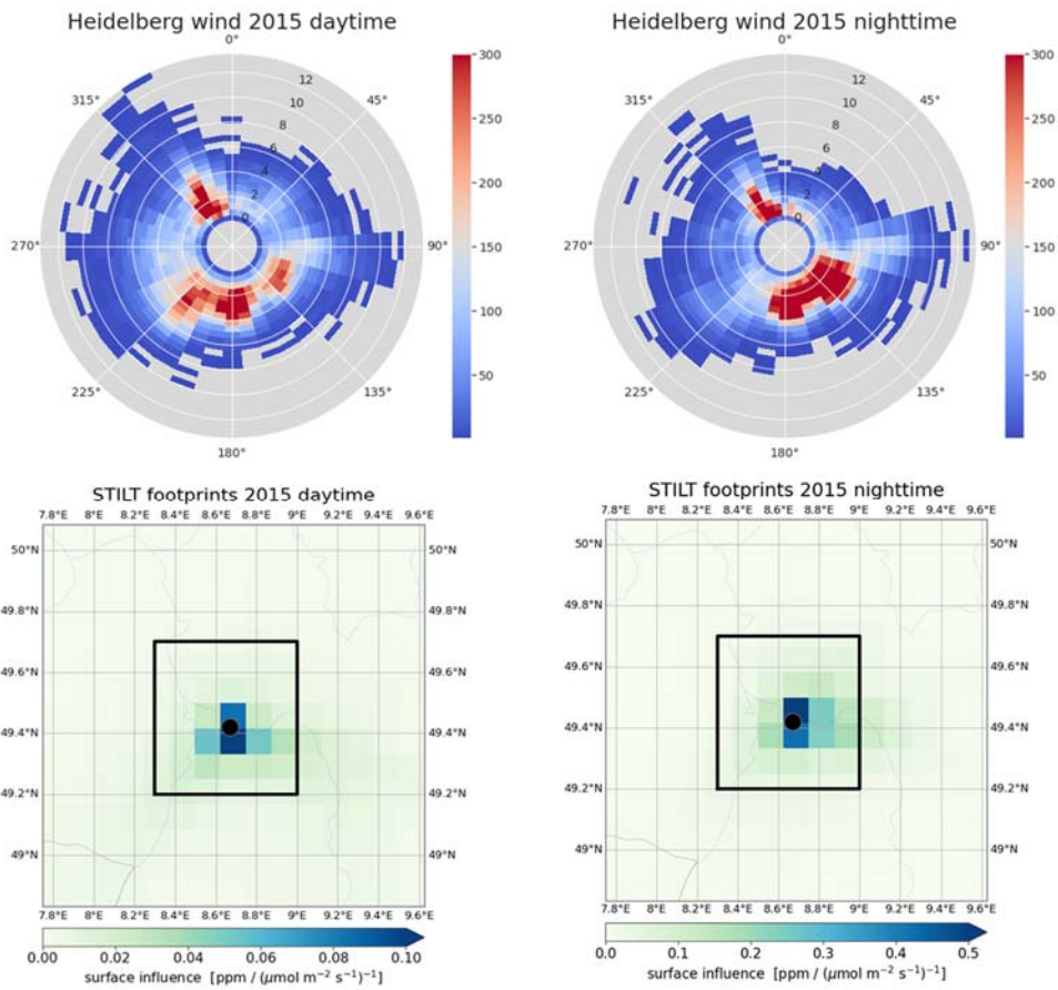
840 Figure 2: The upper two panels show the wind distributions (5-minute mean values, wind velocity in \text{m s}^{-1} displayed on the radius) in 2015 measured on the roof of the Institute for Environmental Physics building at a height of 37 m a.g.l. Daytime (left panel) and nighttime (right panel) wind distributions are similar. The lower two panels show the annually aggregated surface influences of potential emissions for 2015 (left: daytime and right: nighttime). Note the different scales for day and night, indicating an appr. 5-fold sensitivity of emissions on concentrations observed at 30 m a.g.l. during nighttime compared to daytime. The black rectangle 845 marks the “small” influence area with Heidelberg in the approximate centre (black dot).
