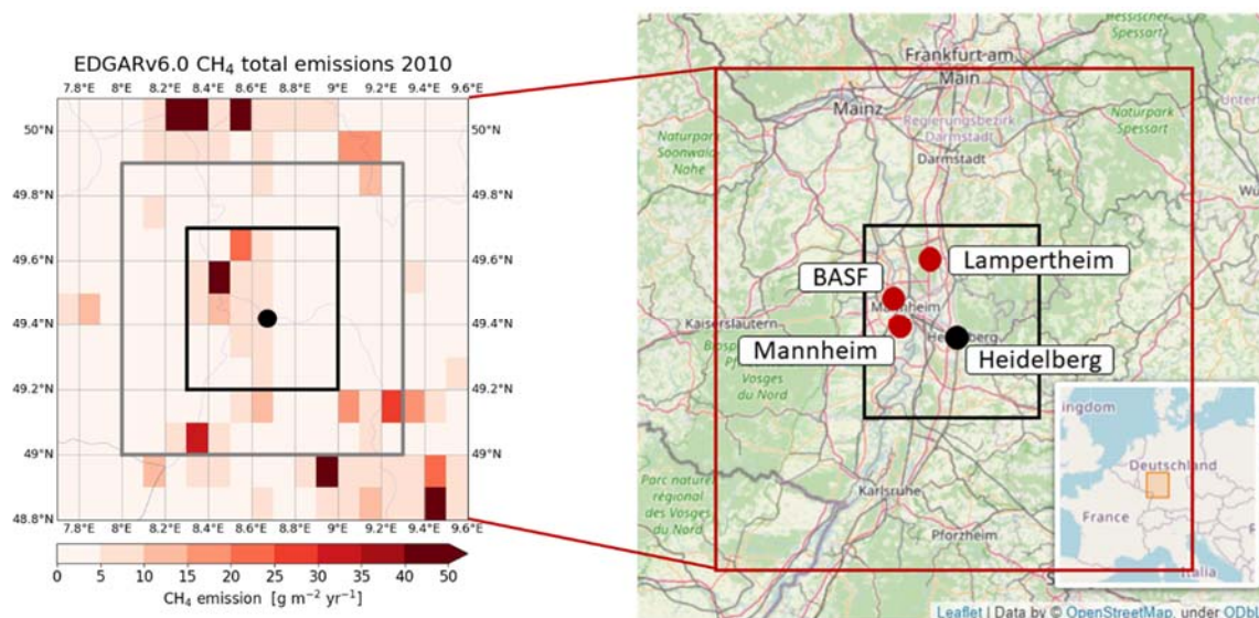
825 830 Figure 1, right panel: Map of the upper Rhine valley south of Frankfurt/Main with the location of Heidelberg (black dot). The red dots indicate industrial areas (Mannheim/Ludwigshafen with the BASF chemical factory) as well as locations of large solid waste deposits (Lampertheim, Mannheim) in the small influence of the station (© OpenStreetMap contributors YEAR. Distributed under the Open Data Commons Open Database License (ODbL) v1.0). Left panel. Gridded CH 4 emissions as reported by the EDGARv6.0 inventory for 2010 (Crippa et al., 2021) covering a ca. 150 km x 150 km (“large”) area surrounding Heidelberg. Two smaller areas, the so-called “small” (ca. 70 km x 70 km) and “intermediate” (ca. 110 km x 110 km) influence areas of Heidelberg are marked as black and grey rectangle, respectively. Long-term trends of average CH 4 emissions from the three influence areas 835 are displayed in Fig. 3.
