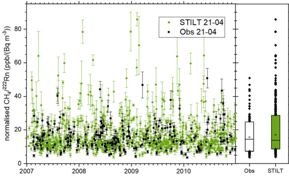
890 Figure 8: Variability of observed (Obs, black squares) and simulated (STILT, green dots) nighttime \text{CH}_4/^{222}\text{Rn} slopes from 2007 to 2010 (left panel). The right panel shows the distributions of all slopes with the boxes including 80% of the data, the open squares representing the mean and the horizontal lines the median values. Note that for the further discussion we excluded the three modelled values >70 \text{ ppb (Bq m}^{-3}\text{)}^{-1} .
