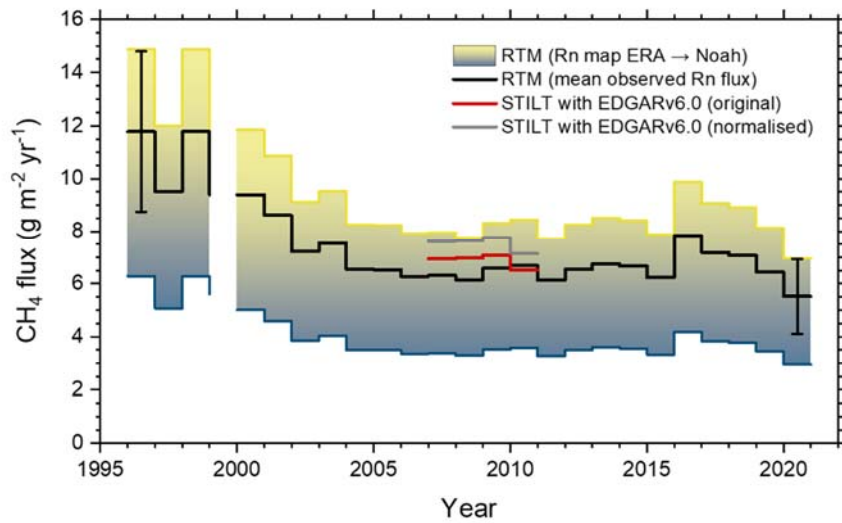
880 Figure 7: Long-term trend of the RTM-based CH 4 flux in the Heidelberg footprint. The black histogram (with typical RTM-based uncertainties shown for the first and the last year of observations) was calculated based on the observation-based 222 Rn flux of 18.3±4.7 Bq m -2 s -1 . The coloured area shows the range of RTM-based CH 4 flux estimates if either the GLDAS Noah soil moisture (yellow) or the ERA Interim Land soil moisture (blue) based 222 Rn flux average of the small influence area would have been used to calculate RTM-based CH 4 fluxes. Also included in the diagram are RTM-based results from STILT-modelled CH 4 and 222 Rn data for 2007 – 2010 (based on the slopes in Fig. 8). The red line shows the original results using the EDGARv6.0 emission 885 inventory and the 222 Rn flux climatology while the grey line shows the STILT results normalised to the observation-based 222 Rn flux (see text).
