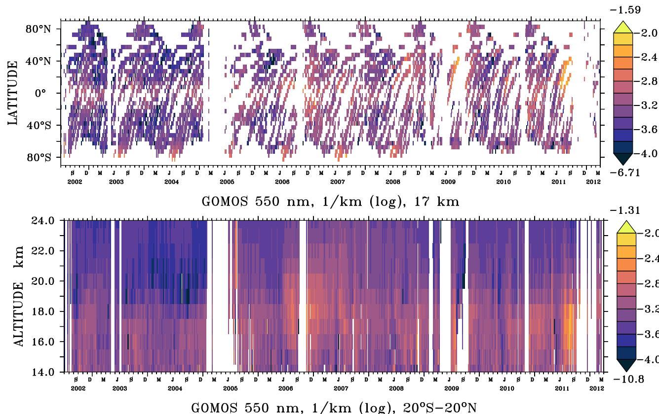
Figure 2. The decadal logarithm (log) of the aerosol extinction coefficient (1/km) as derived from the GOMOS instrument data v.3.00 at 550nm wavelength from Bingen et al. (2017). The dataset spans the period 15 April 2002–8 April 2012 (5-day averages). Horizontal distribution at 17 km altitude (top) and vertical distribution for tropical regions 20° S–20° N (bottom). Maximum and minimum values appear above (yellow) and below (dark blue) the colour keys, respectively. White: no data.
