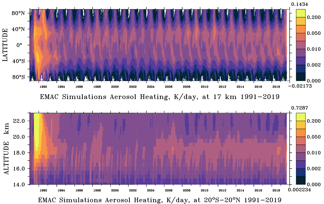
Figure 12. EMAC simulation of the aerosol radiative heating in K per day for solar and infrared radiation from January 1991–August 2019 (5-day averages) based on the volcanic sulfur emission inventory (Table 2), in horizontal distribution at 17 km altitude (top) and in vertical distribution for tropical regions 20° S–20° N (bottom).
