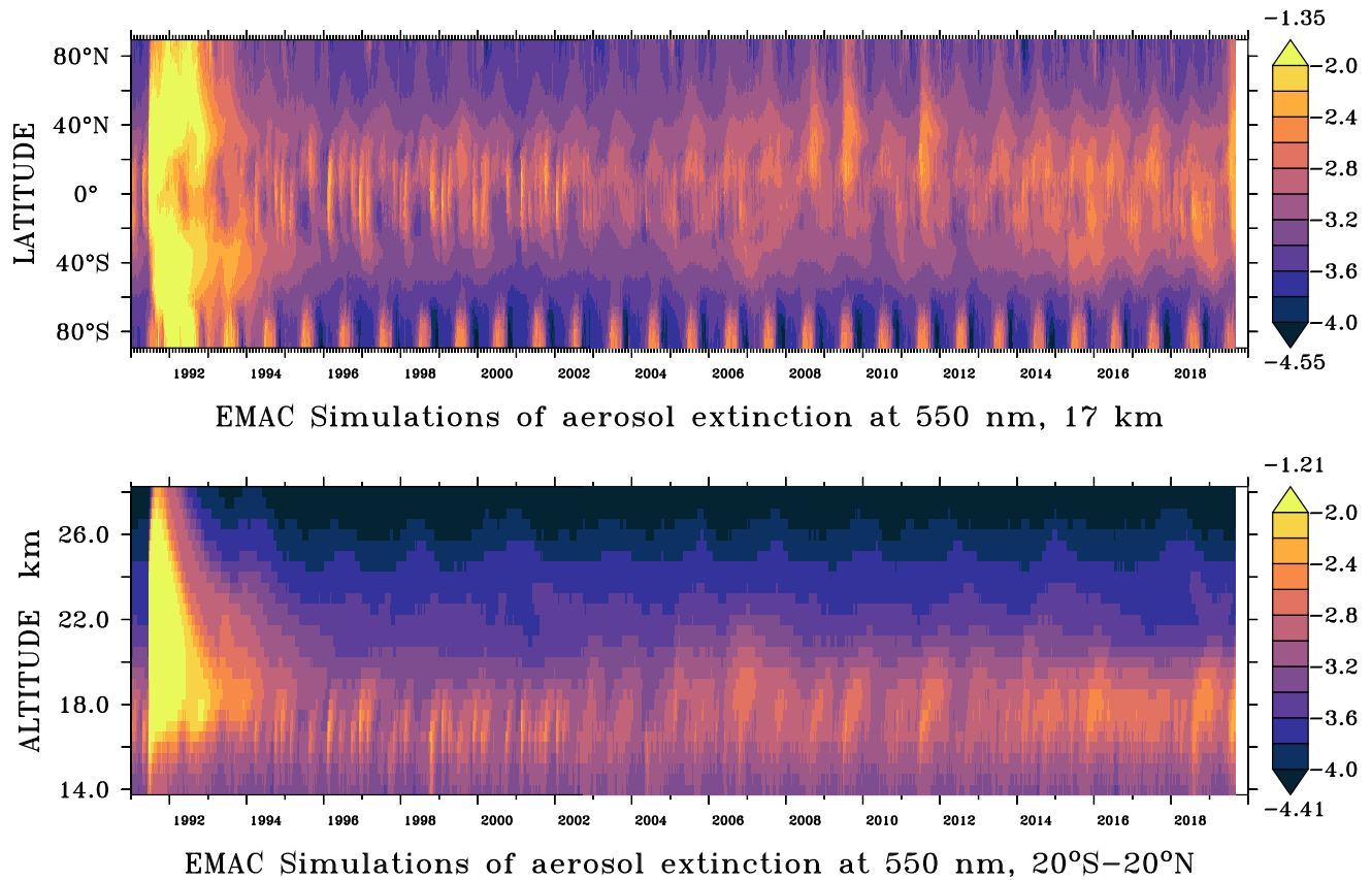
Figure 8. EMAC simulation of the stratospheric aerosol extinction on a logarithmic scale \log(1/\text{km}) for 550nm wavelength from January 1991–August 2019 (5-day averages), zonal mean at 17km altitude (top) and vertical distribution for tropical regions 20° S–20° N (bottom). Maximum and minimum values appear above (yellow) and below (dark blue) the colour keys, respectively.
