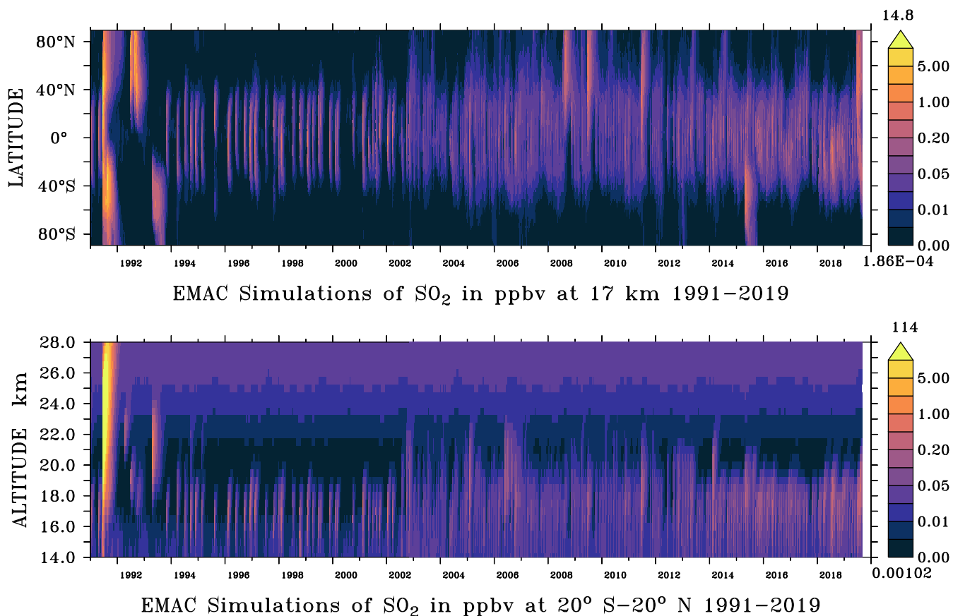
Figure 6. EMAC simulation of the stratospheric \text{SO}_2 mixing ratios (ppbv) (January 1991–August 2019, 5-day averages) using the volcanic sulfur emission inventory (Table 2), at 17 km altitude (top) and in vertical distribution for tropical regions 20° S–20° N (bottom). Maximum and minimum values are indicated above (yellow) and below (dark blue) the colour keys, respectively.
