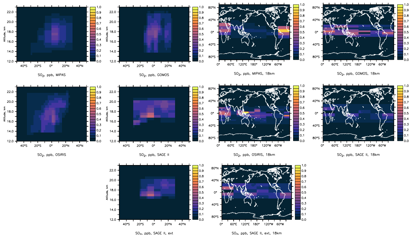
Figure B1. 2002 Reventador eruption: \text{SO}_2 mixing ratio perturbation (ppb) derived from MIPAS and the 3 extinction instruments. MIPAS data of 7 to 17 November 2002, OSIRIS and GOMOS data 11 to 22 November, SAGE II orbits of November and early December 2002. Zonal average vertical distribution (left) and plumes at 18 km altitude (right). OSIRIS with correction factor 0.8 due to remnants from the Ruang eruption, SAGE II with the Grainger-based method. Lower row: SAGE II \text{SO}_2 derived from extinction (interpolated to 750 nm from 525 and 1020 nm). Factor 1 is default.
