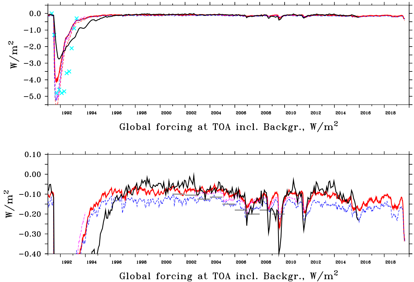
Figure 11. EMAC instantaneous radiative forcing by stratospheric aerosol (red, pink and blue lines, 5-day averages). Solar forcing at the top of the atmosphere (TOA) (dashed red line, upper panel) is compared to solar forcing at the TOA from satellite observations of the Earth Radiation Budget Experiment (ERBE), 72-day means, light blue crosses (Wong et al., 2006; Tooney et al., 2011). The full red line displays the total (solar+IR) forcing at TOA including contributions from aerosol down to the calculated tropopause. The blue dashed line shows the total forcing using the previous scheme at the tropical tropopause (Brühl et al., 2018), the dashed pink line the same with fewer volcanoes of Brühl et al. (2015). Gray bars show annual averages derived from observations by Solomon et al. (2011). The black line shows results from Schmidt et al. (2018) with volcanic effective radiative forcing (aerosol-radiation interactions) at TOA including a background aerosol forcing of -0.05 \text{ Wm}^{-2} . The lower panel is an enhanced representation of the upper panel.
