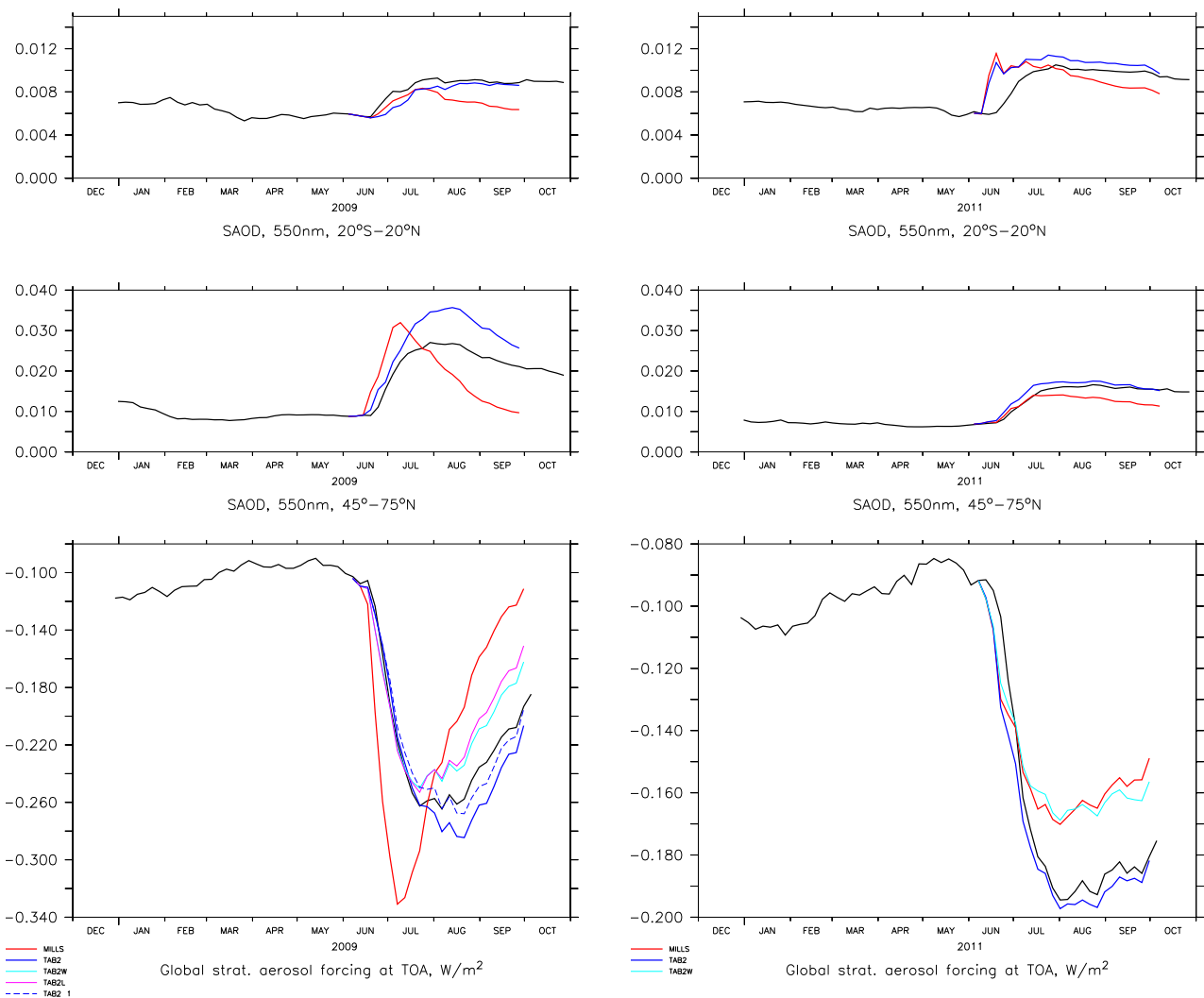
Figure C4. Stratospheric AOD (upper) and global radiative forcing at TOA (lower), Sarychev (left) and Nabro (right), black line as the red line in Figure 9 or Figure 11, blue, light blue and purple lines "point sources" based on Table 2 with different thickness and vertical position of the column into which is injected (see text), red lines with assumptions of Mills et al. (2016). Dashed blue, light blue and purple curves see text.
