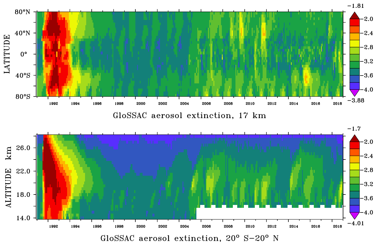
Figure C1. GloSSAC aerosol extinction in logarithmic scale \log(1/\text{km}) for 525 nm wavelength from January 1991–December 2018 zonal mean at 17 km altitude (top) and in vertical distribution for tropical regions 20° S–20° N (bottom). Maximum and minimum values appear above (dark red) and below (violet) the colour keys, respectively. White: no data.
