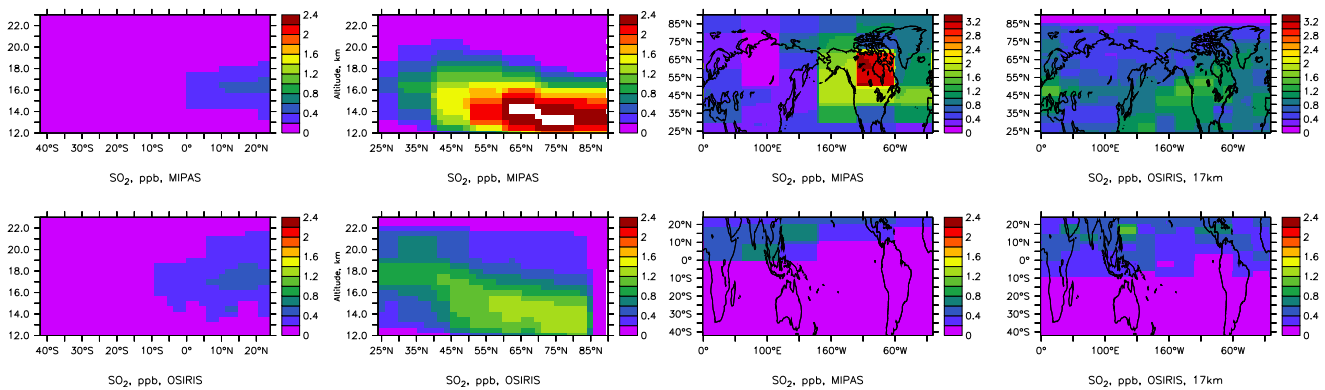
Figure B3. 2009 Sarychev (second column, upper right row) and Mando Hararo (first column, lower right row) eruptions: SO 2 mixing ratio perturbation (ppb) derived from MIPAS and OSIRIS, arrangement of panels because event is split at 24° N as for integrated values in Table 2. MIPAS data 18 June to 18 July 2009, OSIRIS data 17 July to 3 August. Zonal average vertical distribution (left) and plumes at 17 km altitude (right).
