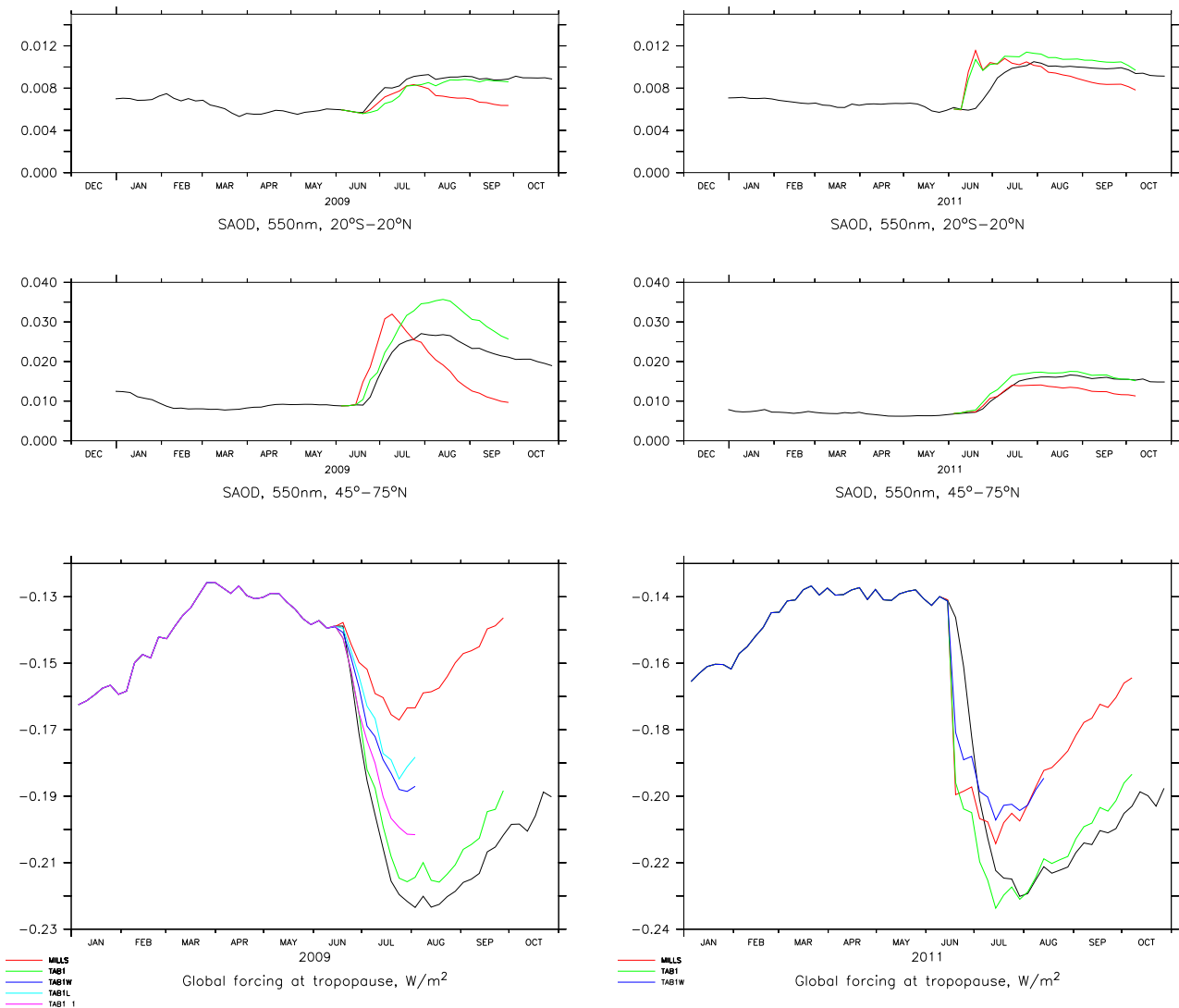
Figure C4. Stratospheric AOD (upper) and global radiative forcing at tropopause (lower), Sarychev (left) and Nabro (right), black line as in Figure 9 or Figure 11, blue, light blue and green from Table 2 with different thickness and vertical position of the column into which is injected (see text), red with assumptions of Mills et al. (2016). Purple and light blue curves see text.
