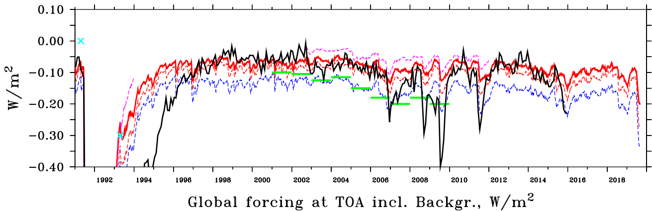
Figure 11. EMAC instantaneous radiative forcing by stratospheric aerosol (red, pink and blue lines, 5-day averages). Solar forcing at the top of the atmosphere (TOA) (dashed red line) is compared to solar forcing at the TOA from satellite observations of the Earth Radiation Budget Experiment (ERBE) (72-day means) (Wong et al., 2006; Toohey et al., 2011) (light blue crosses). The full red line displays the total (solar+IR) forcing at TOA while the blue dashed line shows the same at the tropopause. The dashed pink lines show total forcing at TOA of Brühl et al. (2015). Green bars show annual averages derived from observations by Solomon et al. (2011). The black line shows results from Schmidt et al. (2018) with volcanic radiative forcing at TOA including a background aerosol forcing of -0.05 \text{ Wm}^{-2} . The lower panel is a zoom of the upper panel.
