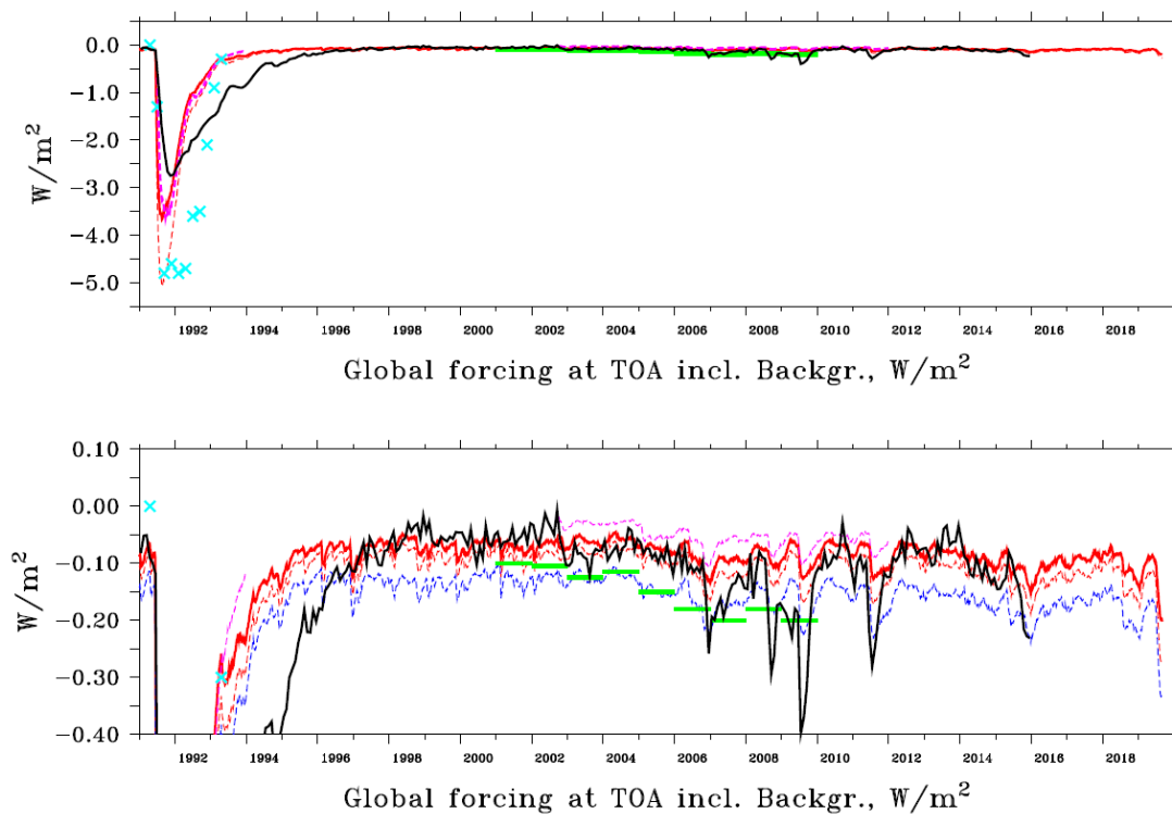
Figure 11. EMAC instantaneous radiative forcing by stratospheric aerosol (red, pink and blue lines, 5-day averages). Solar forcing at the top of the atmosphere (TOA) (dashed red line) is compared to solar forcing at the TOA from satellite observations of the Earth Radiation Budget Experiment (ERBE) (72-day means) (Wong et al., 2006; Toohy et al., 2011) (light blue crosses). The full red line displays the total (solar+IR) forcing at TOA while the blue dashed line shows the same at the tropopause. The dashed pink lines show total forcing at TOA of Brühl et al. (2015). Green bars show annual averages derived from observations by Solomon et al. (2011). The black line shows results from Schmidt et al. (2018) with volcanic radiative forcing at TOA including a background aerosol forcing of -0.05 \text{ Wm}^{-2} . The lower panel is a zoom of the upper panel.
