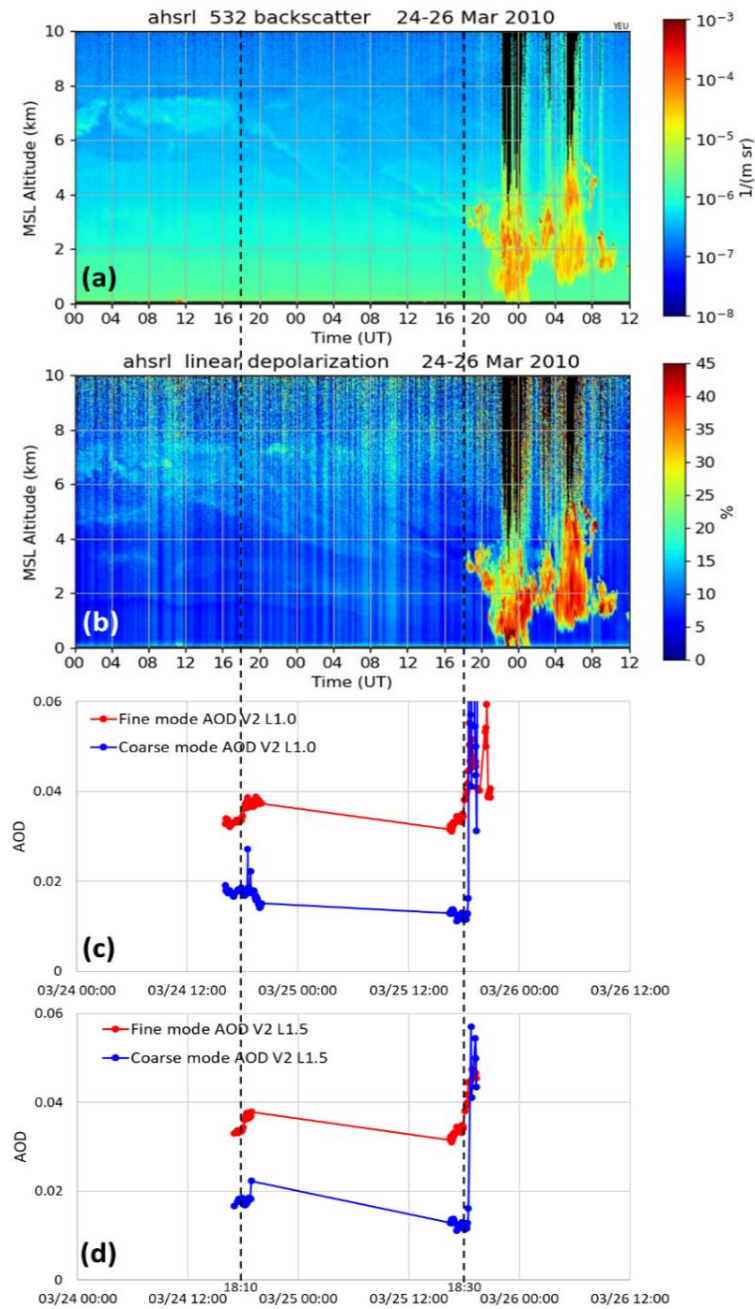
75 Figure 1: (a) AHSRL backscatter coefficient ( \beta ) profile. (b) AHSRL linear depolarization ( \delta ) profile. (c) Level 1.0 (non cloud-screened) fine mode and coarse mode AODs. (d) Level 1.5 (cloud-screened) fine mode and coarse mode AODs (a standard AERONET product). All times are UT. The March 24, 18:10 dashed vertical line indicates the beginning of the decrease in thickness of the coarse mode plume seen in the weak \beta profile and the moderate \delta profile with an attendant weak decrease in the coarse mode AOD (decrease \sim 0.005 from approximately 0.02 to 0.015 for the Version 2 Level 1.0 coarse mode AOD retrievals). The same decrease
