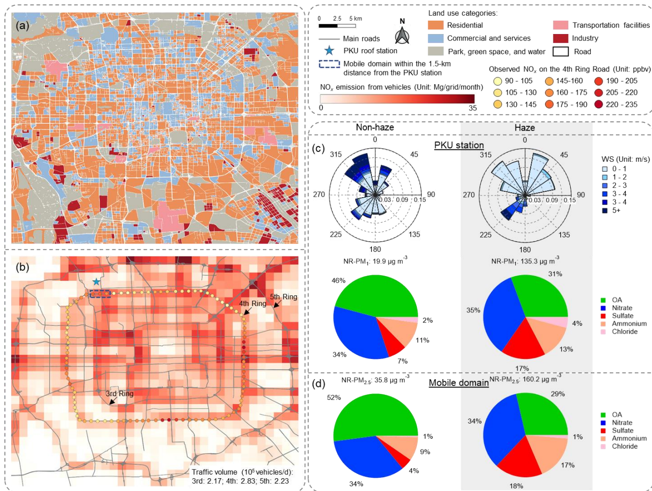
Figure 1. (a) Land use categories in the area of Beijing that were taken from the Mapping Essential Urban Land Use Categories in China (EULUC-China) database (Gong et al., 2020). (b) Monthly \text{NO}_x emissions from vehicle provided by Yang et al. (2019) in November 2018 and the mean \text{NO}_x concentrations observed by the mobile laboratory between 9 a.m. to 4 p.m. during the non-haze measurement period on the 4th Ring Road in Beijing. (c) Wind rose diagrams and the average NR- \text{PM}_{10} composition measured by LTOF-AMS at the PKU roof site. (d) The average NR- \text{PM}_{2.5} composition measured by the TOF-ACSM on the mobile lab on the 4th Ring Road within the distance of 1.5 km from the roof site. Base maps are provided by OpenStreetMap.
