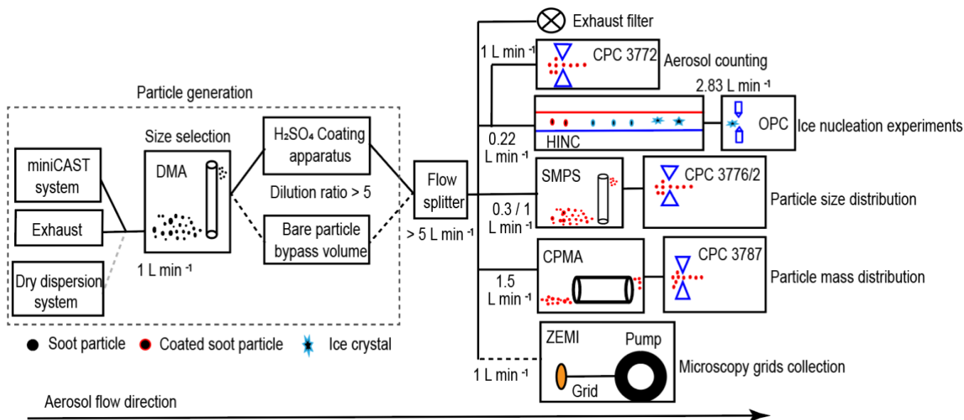
185 Figure 1. Schematic of the experimental setup. miniCAST-miniature Combustion Aerosol Standard; DMA-Differential Mobility Analyser; CPC-Condensation Particle Counter; HINC-Horizontal Ice Nucleation Chamber; OPC-Optical Particle Counter; SMPS-Scanning Mobility Particle Sizer; CPMA-Centrifugal Particle Mass Analyser; ZEMI-Zurich Electron Microscope Impactor.
