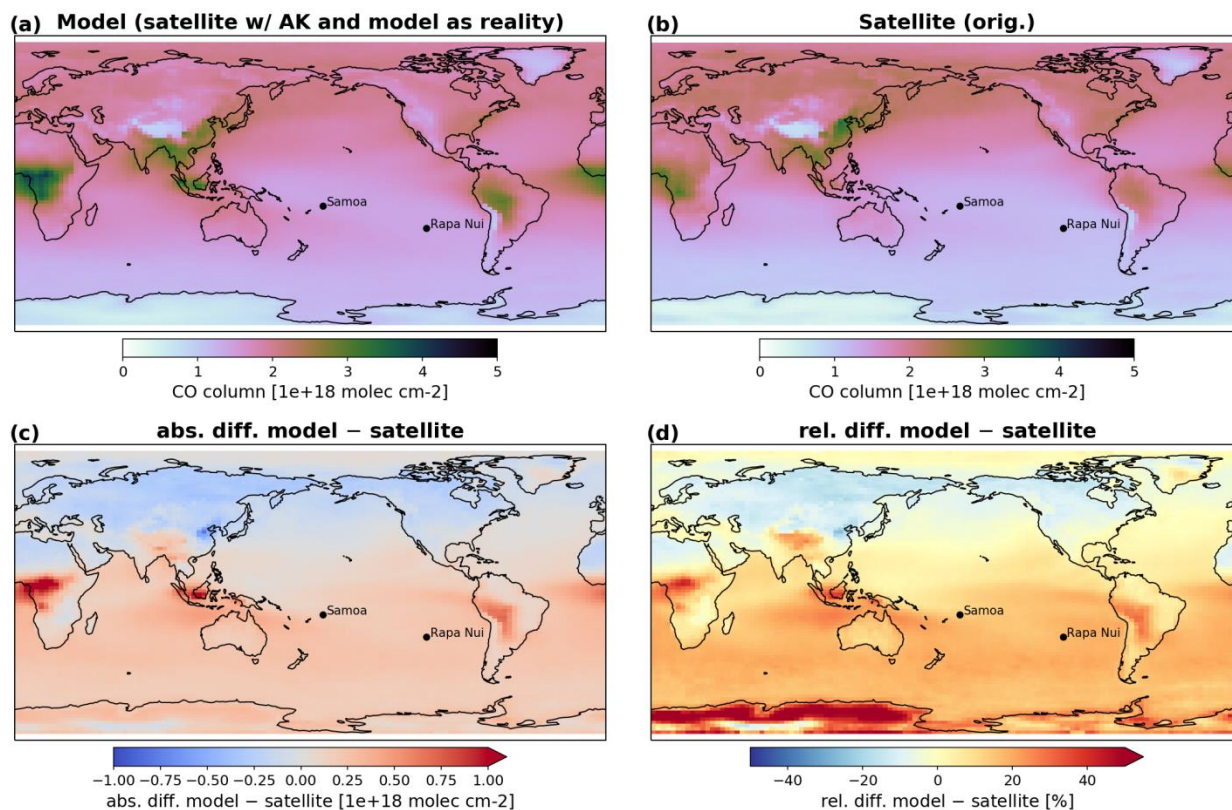
905 Figure 5. Model – Satellite comparison between TM4-ECPL and MOPITT for CO total columns averaged from 2000 to 2014 (in 910 1018 molec/cm 2 ). (a) modelled data sampled following the satellite track and the overpass times and averaged over the period, (b) satellite data averaged over the period, (c) absolute difference (in 1018 molec/cm 2 ) and (d) relative difference (in %) between the mean values of model results and satellite in the 22km x 22km grids of MOPITT. The black dots show the location of Samoa (left) and Rapa Nui (right)
