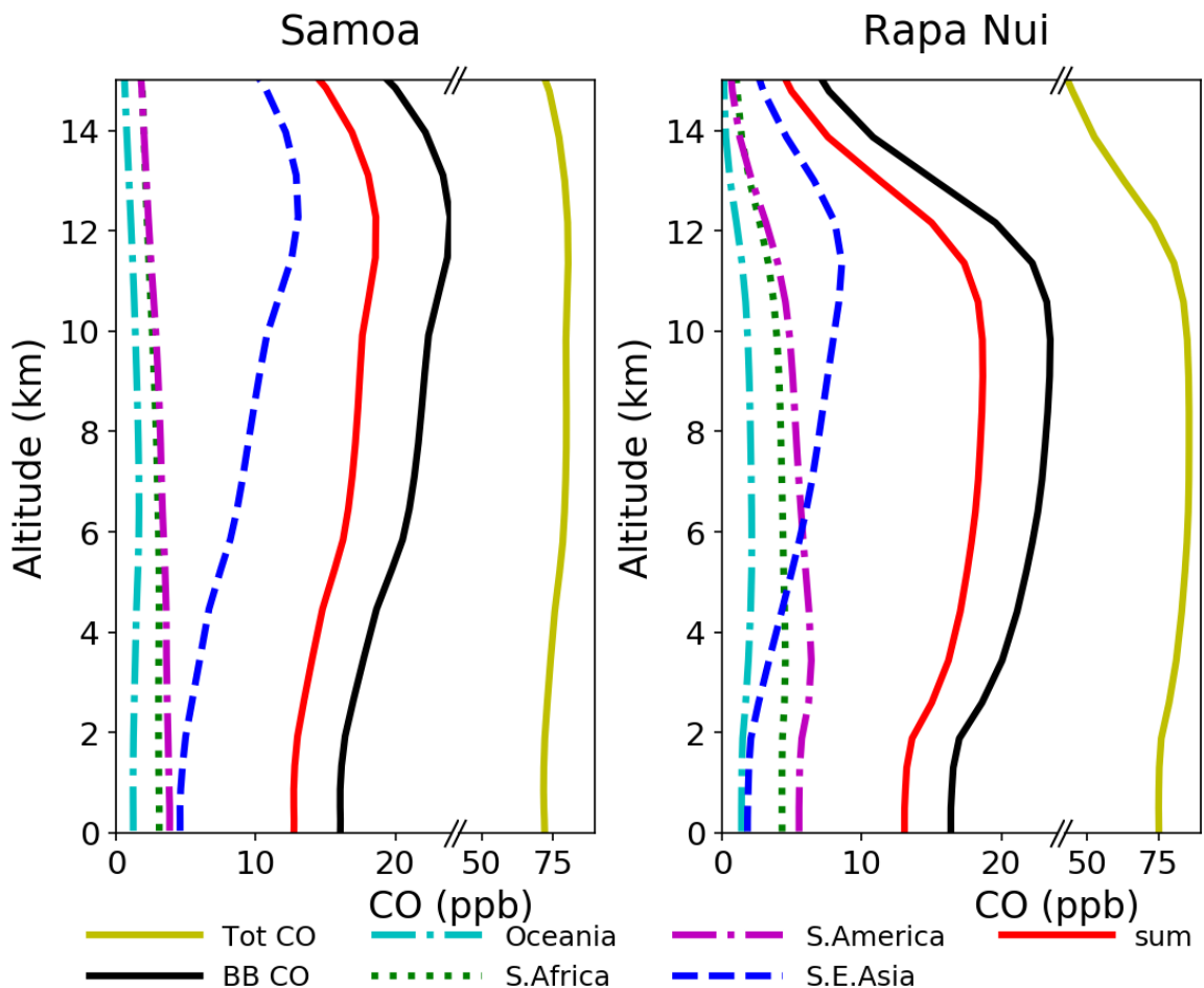
Figure 11. Vertical distribution of CO from different source regions (see legend) in Samoa (left) and Rapa Nui (right) for the high burning period (September-October-November) . Tot CO represents the contribution of all sources of CO, whereas BB CO represents the sum of all shown biomass burning sources. The line in red (sum) indicates the sum of all individual BB contributions shown.
