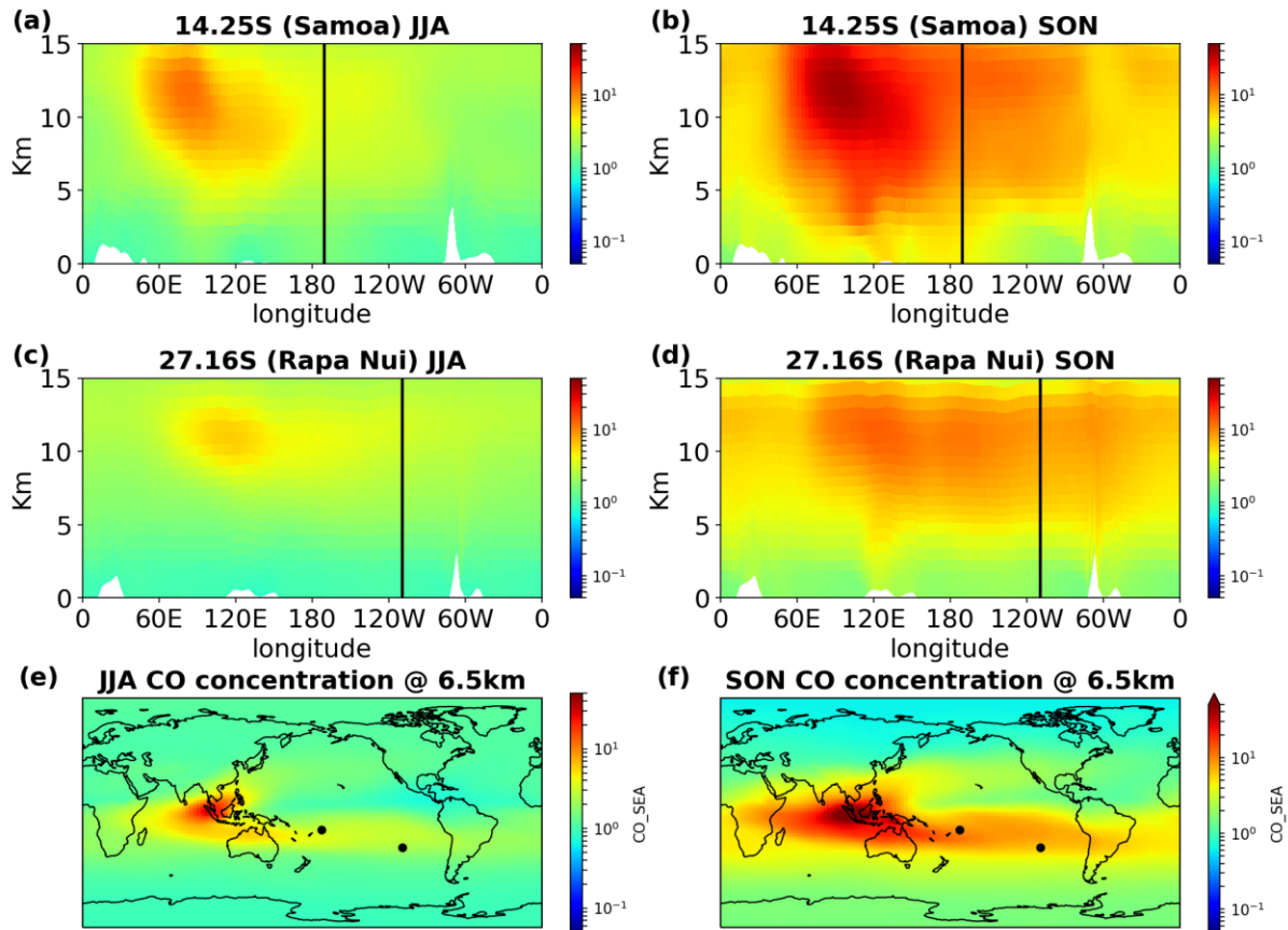
Figure 14. Impact of S. E. Asian fires to CO concentrations. a) JJA and b) SON 20 year mean impact at the cross-section of Samoa, c) JJA and d) SON at the cross-section of Rapa Nui. e) JJA. and f) SON horizontal distribution of the contribution at 6.5 km altitude
