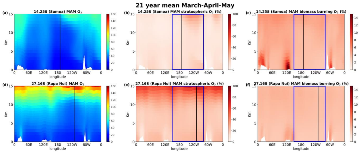
Figure 10. As in Figure 10, but for southern hemisphere autumn (March-April-May). Note that the third column scale is up to 15%.
