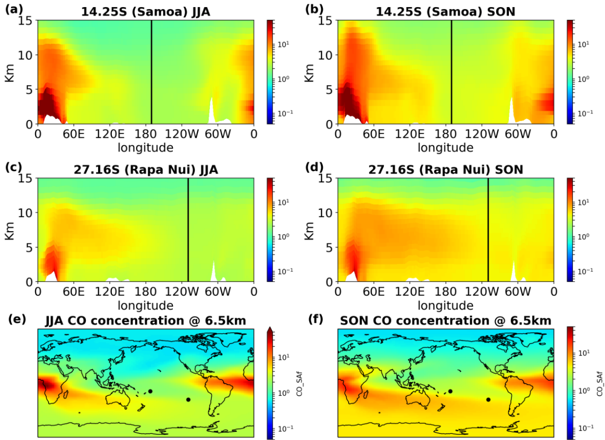
980 Figure 13. Impact of S. African fires to CO concentrations. a) JJA and b) SON 20 year mean impact at the cross-section of Samoa, c) JJA and d) SON at the cross-section of Rapa Nui. e) JJA. and f) SON horizontal distribution of the contribution at 6.5 km altitude
