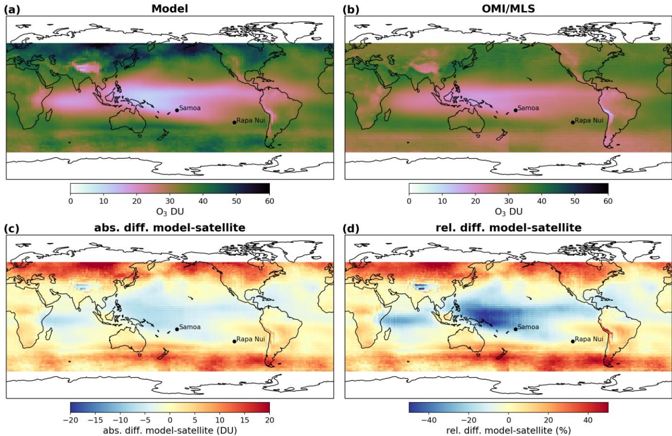
890 Figure 3. Model – Satellite comparison between TM4-ECPL and OMI/MLS mean tropospheric ozone column between October 2004 and December 2014. The top left panel shows the average modelled tropospheric ozone column for the period, the top right the average observed tropospheric ozone column, the bottom left is the absolute difference between model and satellite (DU) and the bottom right the relative difference (%) between model and satellite in the 10x1.25o grid of OMI. The black dots show the location of Samoa (left) and Rapa Nui (right)
