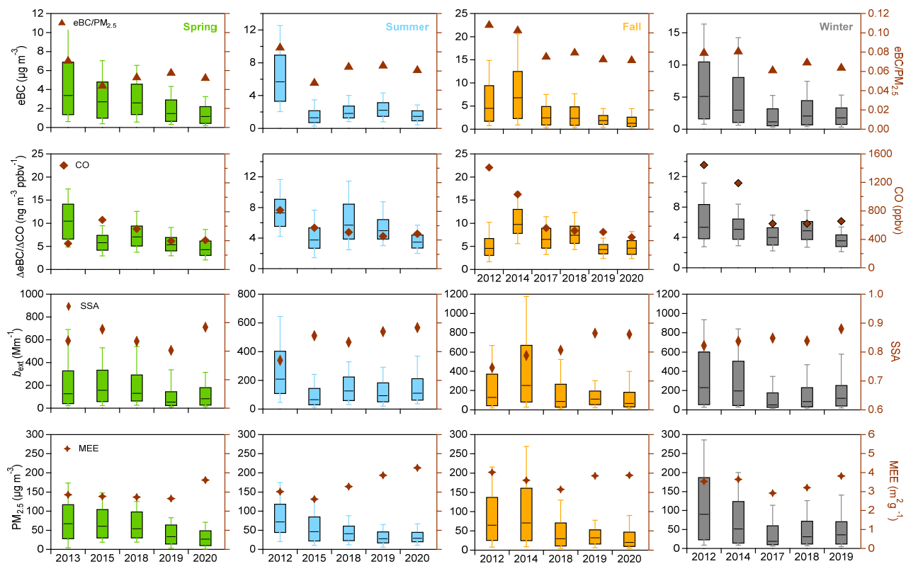
Fig. 3. Seasonal variations in eBC, eBC/PM 2.5 , \Delta eBC/ \Delta CO, CO, b_{\text{ext}} , SSA, PM 2.5 and MEE.
