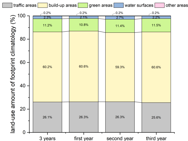
215 Figure 5: Amount of land-use contributing to the flux footprint climatologies separated according to the different time periods of measurement. For data analysis, the footprint information in a 4 km x 4 km grid centred on the measurement site was used (4 m spatial resolution). This footprint area completely includes the 80 % contour line.
