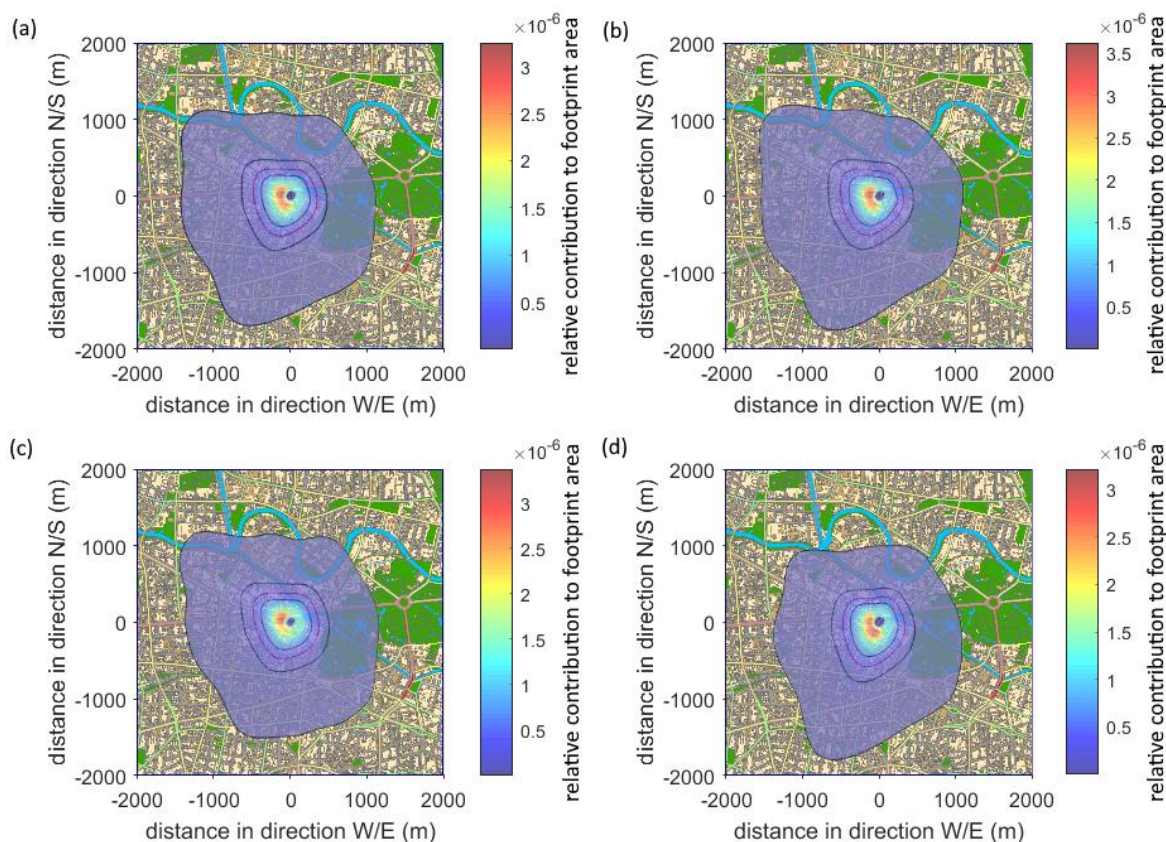
210 Figure 4: Footprint climatology of (a) the entire three-year period, (b) the first year, (c) the second year, and (d) the third year. Flux footprints were calculated for a 4 km x 4 km area (4 m spatial resolution). For reasons of clarity only the 40 %, 50 % (purple), 60 %, and 80 % contour lines are shown (footprint model: Kljun et al., 2015; map data sources: Geoportal Berlin, 2014 (modified), 2021; Umweltatlas Berlin, 2017).
