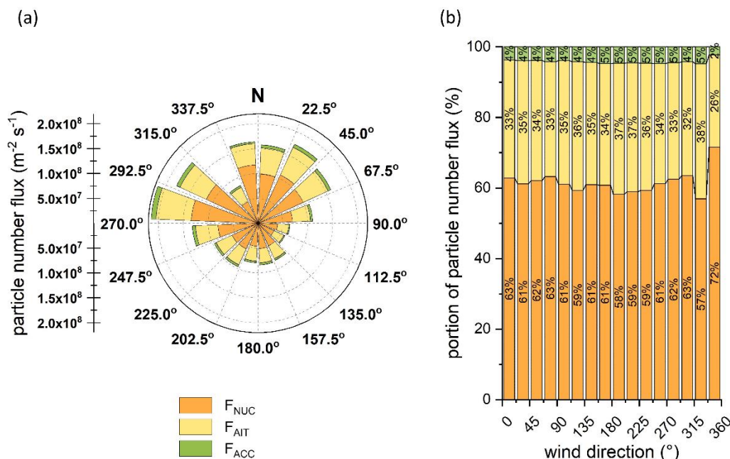
300 Figure 11: (a) Average particle number fluxes and (b) fraction of specific particle mode fluxes binned into 22.5^\circ sectors for F_{\text{NUC}} , F_{\text{AIT}} , and F_{\text{ACC}} .
