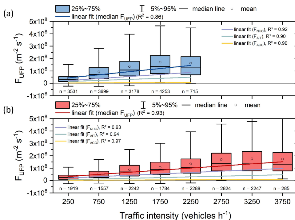
325 Figure 14: Relationship between F_{UFP} and traffic intensity at (a) “Hardenbergstraße” (HS) and (b) “Straße des 17. Juni” (S17J). Linear regression lines for the particle mode fluxes F_{NUC} , F_{AIT} , and F_{ACC} are given.
