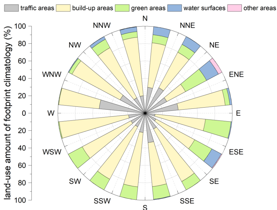
Figure 13: Fraction of land-use per wind direction sector contributing to the three-year flux footprint. For data analysis the flux footprint was defined as a circle centred of the flux site with a radius of 2 km.
