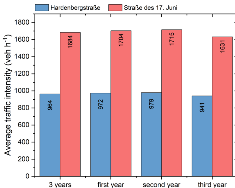
410 Figure A3: Average traffic intensity measured at the two traffic counting stations “Hardenbergstraße” (HS) and “Straße des 17. Juni” (S17J) for the entire measurement period and each observation year.
