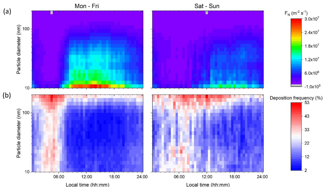
265 Figure 9: Diurnal cycles for a weekday (Mon – Fri) and a day of weekend (Sat – Sun) of (a) size-resolved average particle number fluxes ( F_N ) and (b) the frequency of particle deposition. In (a) colours indicate the strength of emission fluxes while grey colour symbolises a slight particle deposition.
