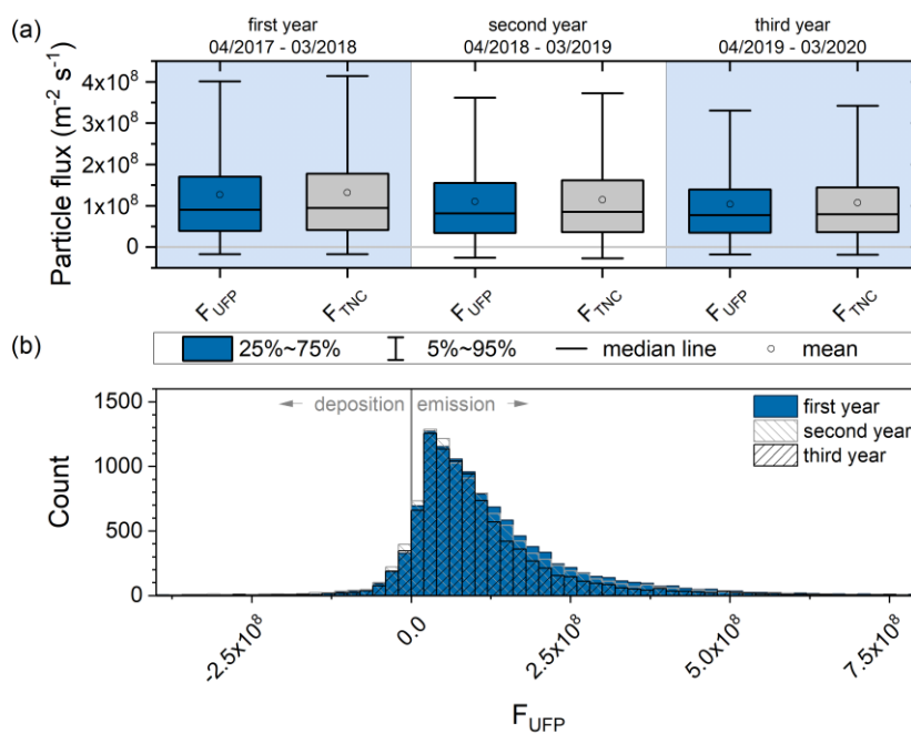
235 Figure 6: (a) Range of F_{TNC} and F_{UFP} and (b) the frequency distributions of F_{UFP} for each of the three years of measurement.
