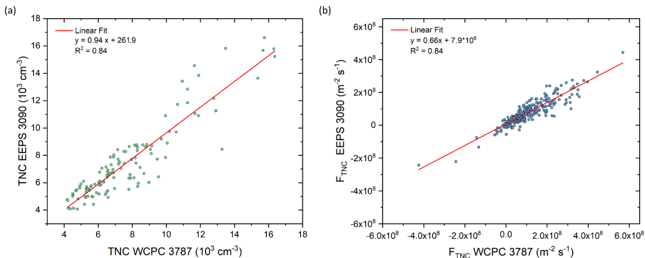
405 Figure A2: Measurement comparison of EEPS 3090 with WCPC 3787 at the Berlin site concerning (a) total particle number concentration (TNC, 4 days, July 2020) and (b) total particle number flux ( F_{TNC} , 12 days, September 2020). The data of EEPS relate to particle sizes between 10 and 200 nm whereas the WCPC counts particles with D_p > 5 nm.
