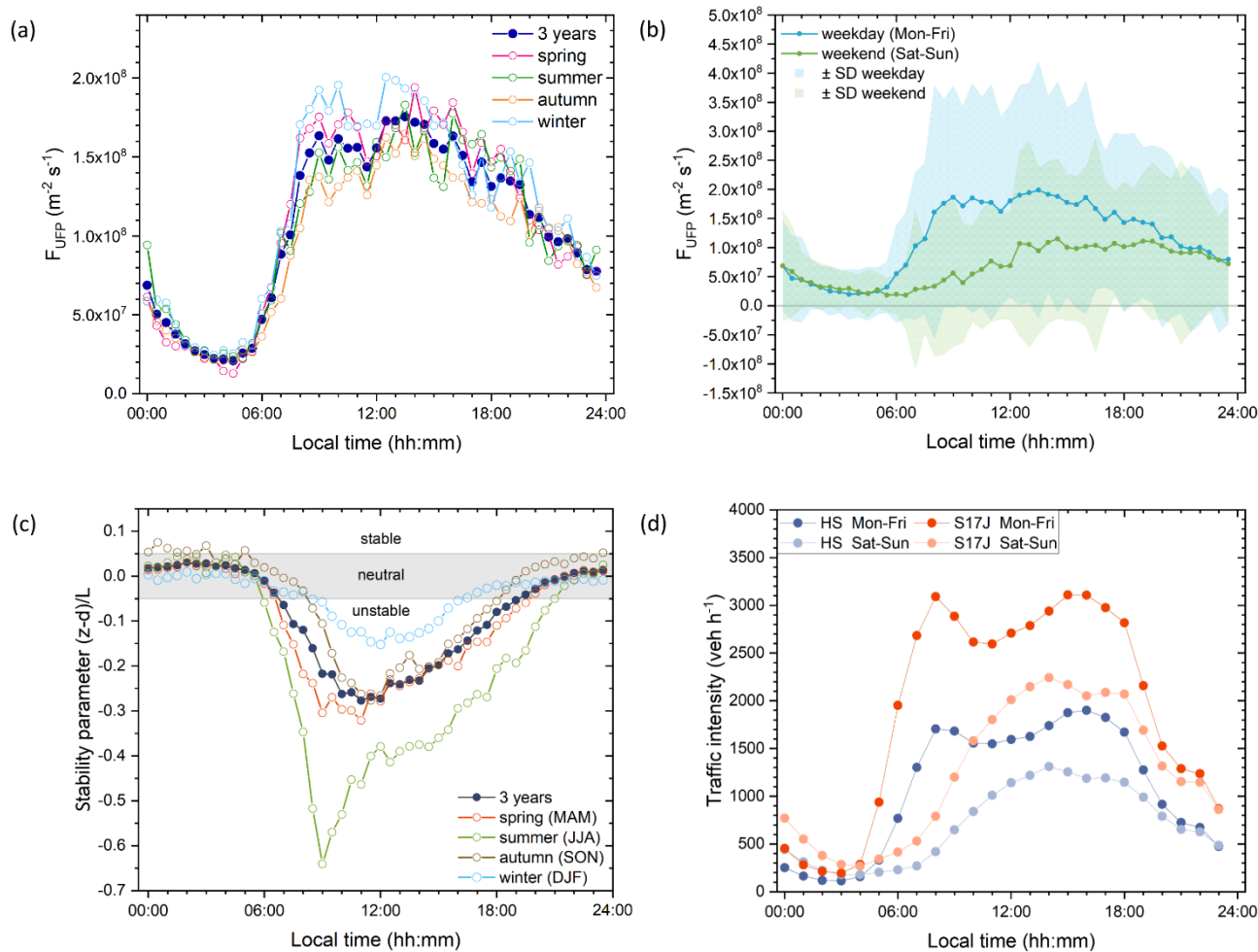
250 Figure 8: Diurnal cycles of (a) average and seasonal F_{UFP} , (b) average F_{UFP} for weekdays and weekends with standard deviation (SD), (c) median stability parameter (z-d)/L for each season and the whole measurement period with z = measurement height, d = displacement height, and L = Monin-Obukhov length, and (d) average traffic intensity at HS and S17J.
