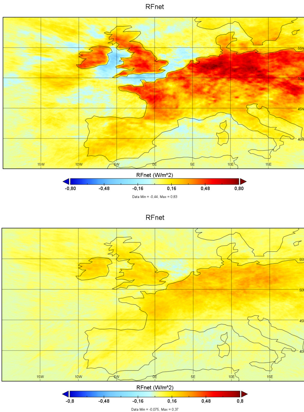
Figure 9: Mean net RF in W m^{-2} from contrails, March-August mean, 2019 (top) and 2020 (bottom).
