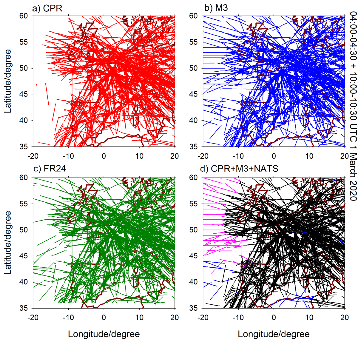
485 Figure 1: Geographic map of the European domain under consideration for contrail simulations with coloured flight tracks for two half-hour example time periods of 1 March 2020, before the COVID-19 crisis. Individual panels show track data from a) CPR (red), b) M3 (blue), c) FR24 (green) and d) from the combination of CPR with M3 and NATS data for flights extending beyond the CPR range (black, blue, and purple lines).
