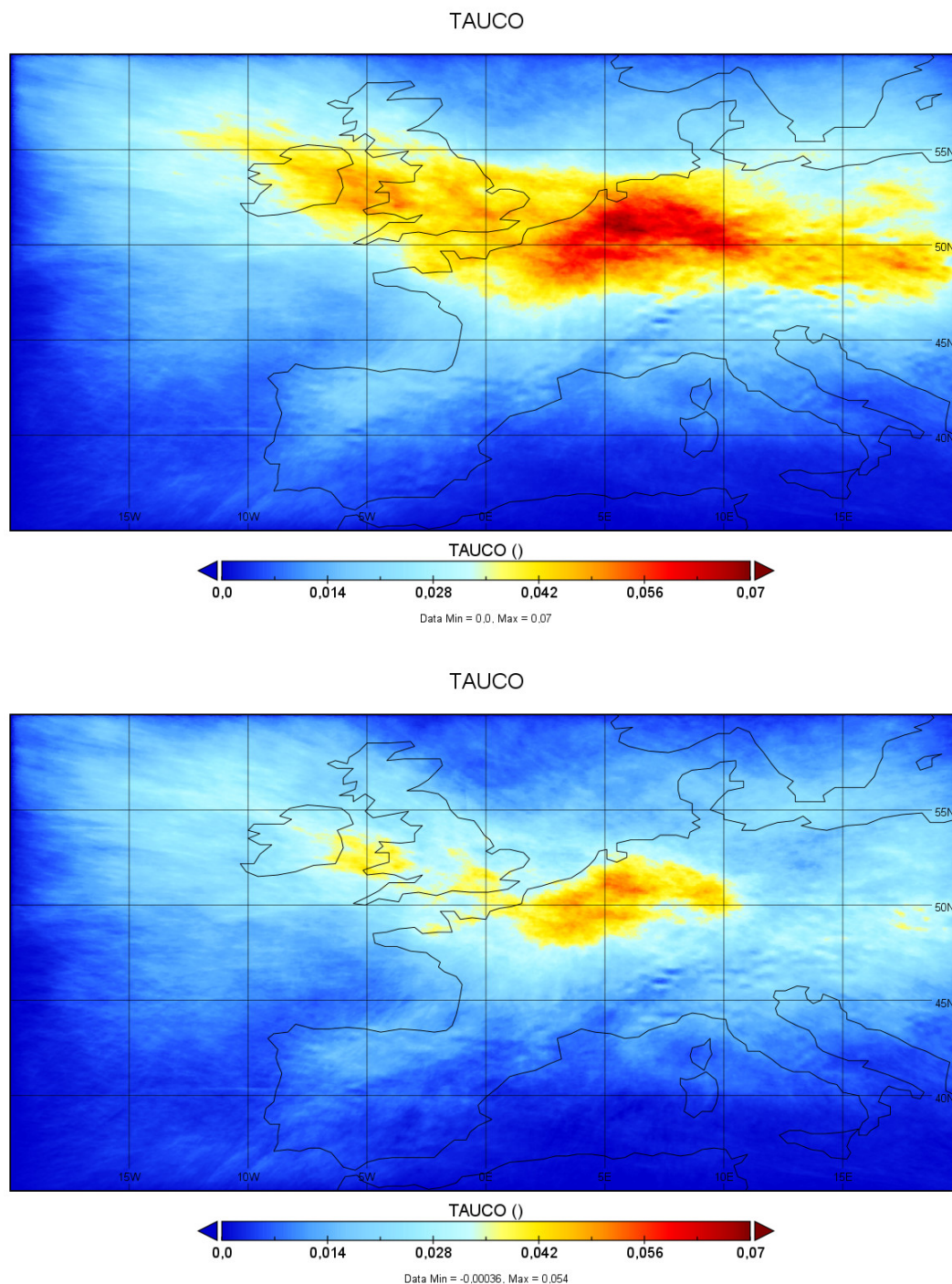
535 Figure 8: Mean optical thickness of contrails, March-August mean, 2019 (top) and difference 2019-2020 (bottom).
