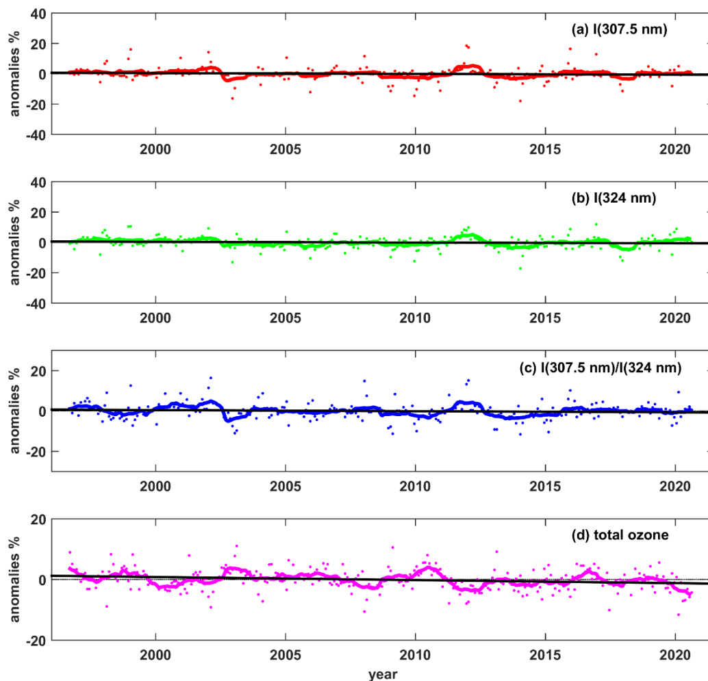
695 Figure 6. Anomalies (% differences relative to the monthly climatological values, represented by dots), 12-month moving averages (thick coloured lines), and trends (black lines) for Rome, for the monthly averages of (a) the irradiance at 307.5 nm, (b) the irradiance at 324 nm, (c) the ratio between the 307.5 nm and 324 nm irradiances, and (d) the total ozone.
