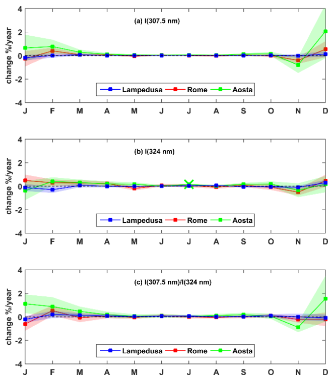
Figure 3: Average change (%) per year of (a) irradiance at 307.5 nm, (b) irradiance at 324 nm, and (c) the 307.5/324 nm ratio. Results are for SZA=67° for the period September 2006 – August 2020. Statistically significant changes have been marked with x. Shaded areas correspond to the 1-sigma standard deviation.
