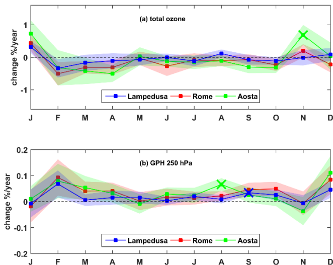
690 Figure 5: Average (%) change per year of (a) total ozone, and (b) GPH for the period 2006 – 2020. Statistically significant changes have been marked with x.
