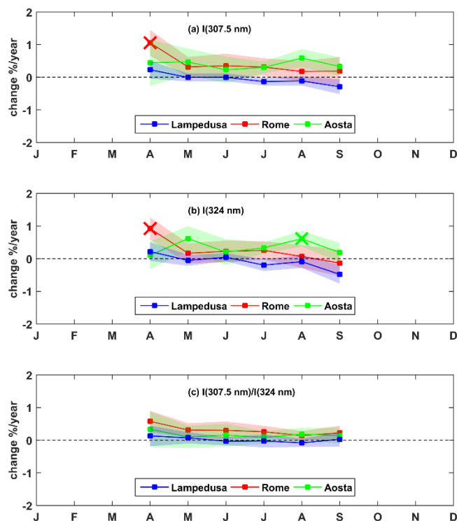
685 Figure 4: Average (%) change per year of (a) irradiance at 307.5 nm, (b) irradiance at 324 nm, (c) the ratio between the irradiances at 307.5 nm and 324 nm. Results are for 45^\circ the period 2006 – 2020. Statistically significant changes have been marked with x. Shaded areas correspond to the 1-sigma standard deviation.
