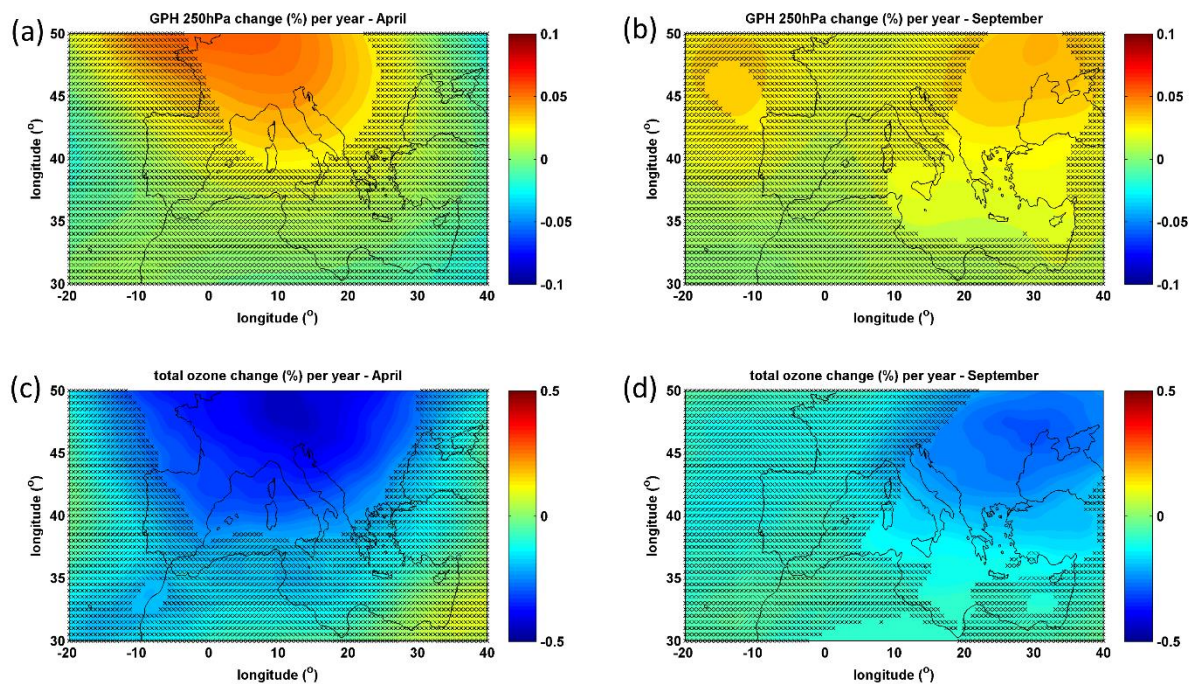
705 Figure 9: Changes (%) of GPH at 250 hPa (a,b) and total ozone (c,d) and for April (a,c), and September (b,d). Areas over which changes are not statistically significant are covered by x.
