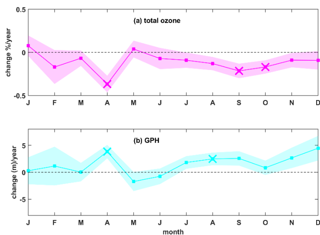
Figure 8: Average (%) change per year of (a) total ozone, and (b) GPH, for Rome. Statistically significant trends have been marked with x. Shaded areas correspond to the 1-sigma standard deviation.
