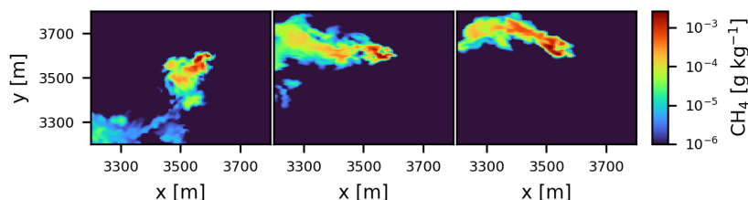
Figure 5. Snapshots of instantaneous plumes at 3 m above the surface. Plume at (left) 11:30:00 UTC, (middle) 12:11:30UTC, (right) 13:00:00 UTC.
