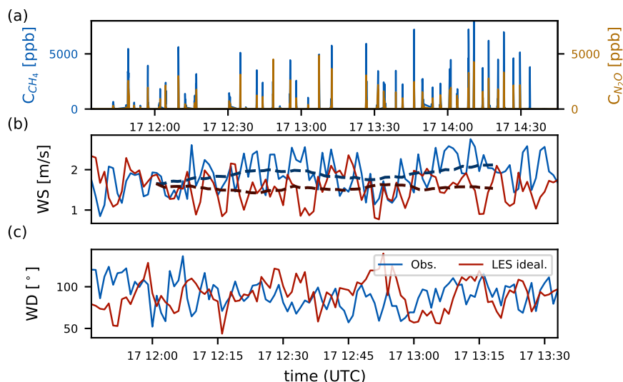
Figure 6. (a) \text{CH}_4 concentrations measured over the read adjacent to the emitting oil-well and \text{N}_2\text{O} concentrations emitted from next to the well. Comparison of the observed and simulated (b) horizontal wind speed, (c) horizontal wind direction. The values are given as one minute averages of instantaneous wind. The dotted lines are rolling means of respective wind speeds, shown here for easier interpretation of the mean wind speed.
