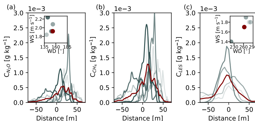
Figure 7. Averages of instantaneous plumes over periods of half hour from (a) \text{N}_2\text{O} , (b) \text{CH}_4 and (c) LES. LES transects were taken at 3 m height and 78 m downwind from the source. Plumes are shown with a color gradient corresponding to the half-hour increments i.e. lightest gray plume is the average of plumes measured over the time period 11.30 - 12.00 UTC, dark grey is the average over 14.00 - 14.30 UTC. The inset shows horizontal wind speed and direction for the corresponding half-hour averages in (a) measurements and (c) LES. Overplotted in red is the average of all the plumes, as well as the averages of horizontal wind speed and direction in the insets.
