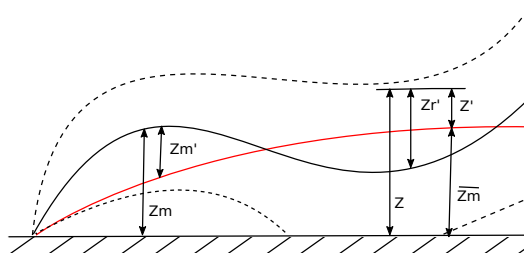
Figure 4. Scheme of idealized plume dispersing from a ground point-source. Shown here are the mean position of the instantaneous plume z_m and the centerline position and the total mean of centerline positions \overline{z_m} (red line). Also shown are the displacements of particles in the instantaneous plume from its centerline position z_r and from the total mean centerline position z' as well as the displacement of the instantaneous centerline from the total mean centerline z'_m .
