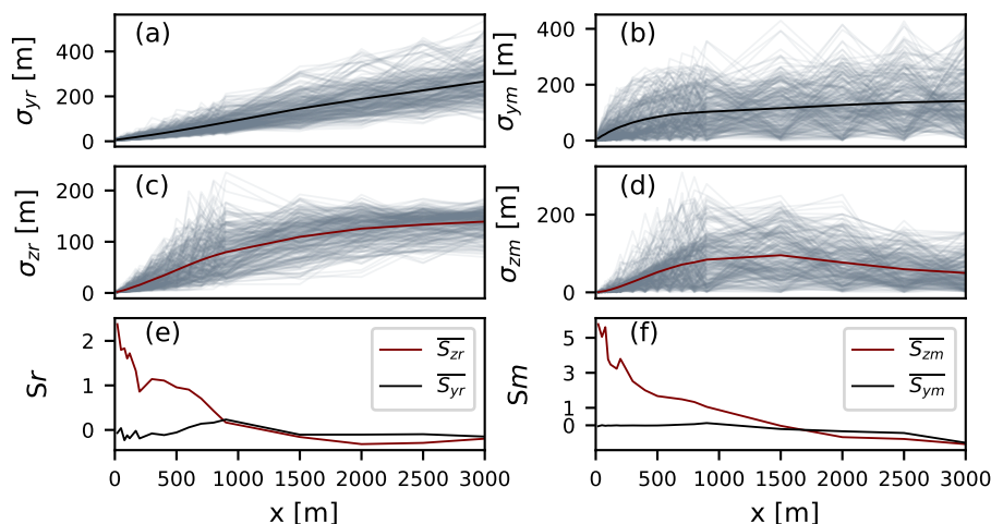
Figure 11. The second and third statistical moments of the simulated plume for the relative (left row) components centered around the mean plume position and for the meandering (right row) components. The first two panels in a row show the plume width in the y and z directions. All values are shown as functions of downwind distance. In grey are shown values of instantaneous plumes while their mean values are shown as solid black and red lines in y and z directions respectively. The last panel shows skewness of the mean relative plume position as a function of distance from the source.
