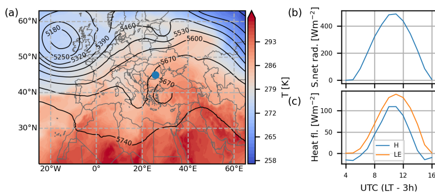
Figure 2. Meteorological situation over Europe on 17th October 2019. (a) Geopotential height (m) at the 500 hPa pressure level and temperature at 850 hPa at 12 UTC. Location of the studied region is indicated on the map by a blue circle. (b) Surface net solar radiation, (c) hourly values of sensible and latent heat at the location of the measurements.
