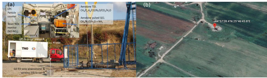
Figure 1. (a) (Inset figure) The measurement set-up inside the TNO vehicle. (Main figure) The TNO vehicle used in the measurement campaign, the location of the inlet is indicated on the figure. (b) Google Earth view of the measurement site with the oil-well location pointed out.
