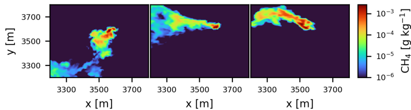
Figure 5. Snapshots of instantaneous plumes at 3 m above the surface. Plume at (left) 11:30:00 UTC, (middle) 12:15:00 UTC, (right) 13:00:00 UTC.
