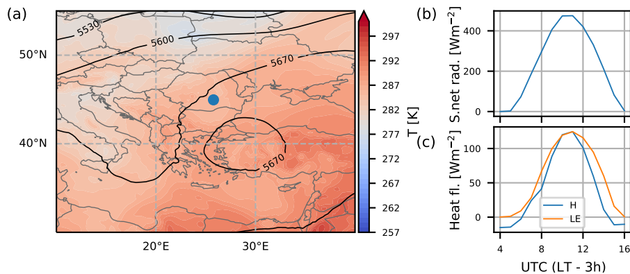
Figure 2. Meteorological situation over SE Europe on 17th October 2019. (a) Geopotential height (m) at the 500 hPa pressure level and temperature at 850 hPa at 12 UTC. The location of the studied region is indicated on the map by a blue circle. (b) Surface net solar radiation, (c) hourly values of sensible and latent heat at the location of the measurements.
