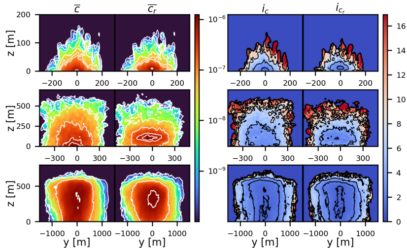
Figure 12. (First two columns) y - z transect of mean plume concentrations in absolute ( \bar{c} ) and relative ( \bar{c}_r ) coordinate system. (Last two columns) Concentration fluctuation intensity in y - z plume in absolute ( i_c ) and relative ( i_{cr} ) coordinate systems. Distances from the source are (top) 100 m, (middle) 600 m and (bottom) 3000 m.
