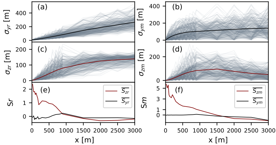
Figure 11. The second and third statistical moments of the simulated plume for the relative (left column) components centered around the mean plume position and for the meandering (right column) components. The first two panels in a row show the plume width in the y and z directions. All values are shown as functions of downwind distance. In grey are shown values of instantaneous plumes while their mean values are shown as solid black and red lines in y and z directions respectively. The last panel shows skewness of the mean relative plume position as a function of distance from the source.
