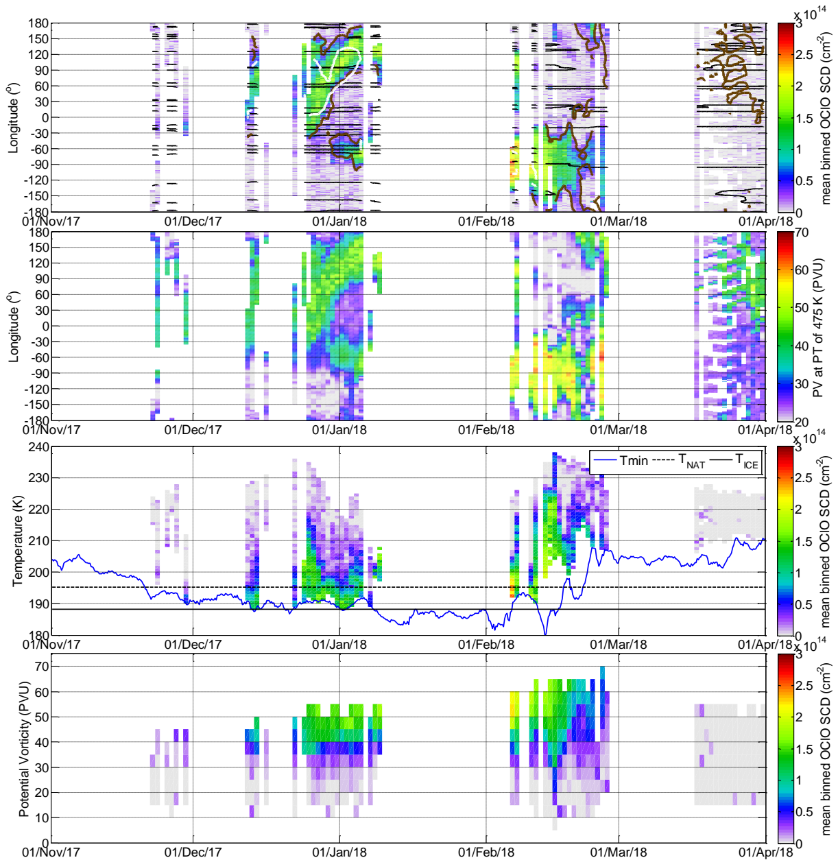
Figure 2. Top panel: Time series of the daily measured OCIO SCDs for 89^\circ < \text{SZA} < 90^\circ resolved longitudinally (resolution 1^\circ , positive values – East longitudes, negative values – West longitudes) for the Arctic winter 2017/2018. Black, brown and white contourlines indicate the maximum surface elevation of 1 km, PV 35 PVU at PT 475 K and temperature T_{\text{NAT}} , respectively. Second panel: Time series of the potential vorticity at the location of the OCIO measurements shown in the panel above. Third panel: The same OCIO dataset as in the top panel but resolved as function of temperature (resolution 1 K) at the PT 475K level. Here also the minimum polar hemispheric temperature (mimumum temperature for latitudes above 60^\circ ) at this potential temperature level (blue line) and the values of T_{\text{NAT}} and T_{\text{ICE}} (at 19.5 km) are indicated. Bottom panel: Same OCIO dataset as in the top panel, but resolved as function of the potential vorticity (resolution 5 PVU) .
