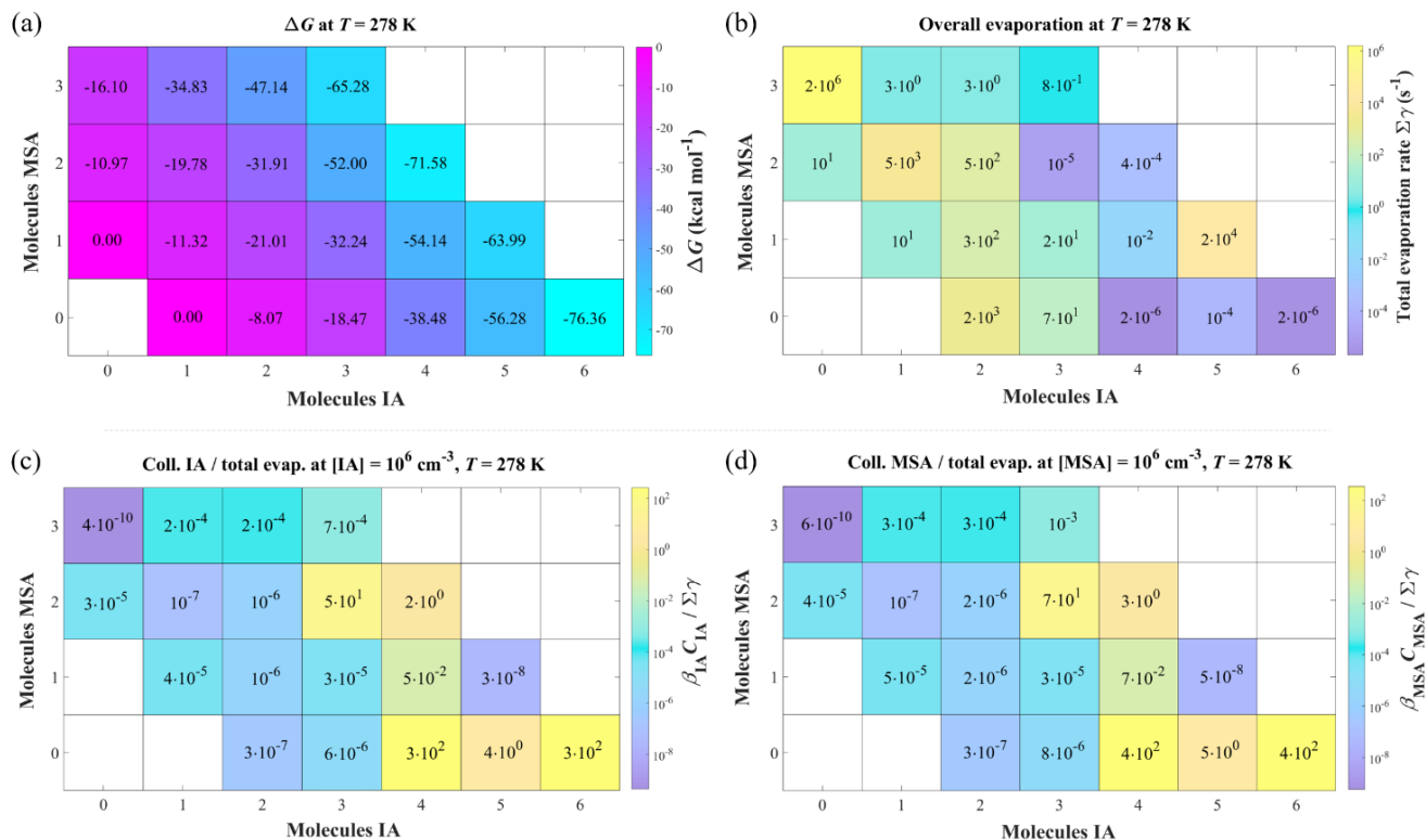
Figure 2. (a) Gibbs formation free energy ( \Delta G , \text{kcal mol}^{-1} ) of the (IA)_x(MSA)_y ( 0 \leq x \leq 6 , 0 \leq y \leq 3 , 1 < x + y \leq 6 ) clusters calculated at the RI-CC2/aug-cc-pV(T+d)Z(-PP)// \omega B97X-D/6-311++G(3df,3pd) + aug-cc-pVTZ-PP level of theory, T = 278 K, p = 1 atm. (b) the total evaporation rate coefficients ( \Sigma\gamma , \text{s}^{-1} ), and the ratios of collision frequencies with (c) IA monomer or (d) MSA monomer versus total evaporation rate coefficients ( \beta_{IA}C_{IA}/\Sigma\gamma or \beta_{MSA}C_{MSA}/\Sigma\gamma ) of the corresponding clusters. \beta is the rate coefficient of cluster collision with monomer, and C is the monomer concentration.
