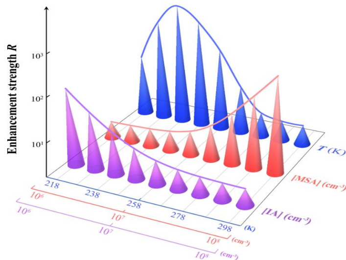
Figure 4. Enhancement strength R of MSA on cluster formation rates under different atmospheric conditions: T = 218 - 298 \text{ K} (blue cones, [\text{IA}] = 10^7 and [\text{MSA}] = 10^7 \text{ molecules cm}^{-3} ), [\text{MSA}] = 10^6 - 10^8 \text{ molecules cm}^{-3} (red cones, T = 278 \text{ K} and [\text{IA}] = 10^7 \text{ molecules cm}^{-3} ), [\text{IA}] = 10^6 - 10^8 \text{ molecules cm}^{-3} (purple cones, T = 278 \text{ K} and [\text{MSA}] = 10^7 \text{ molecules cm}^{-3} ), and \text{CS} = 2.0 \times 10^{-3} \text{ s}^{-1} .
