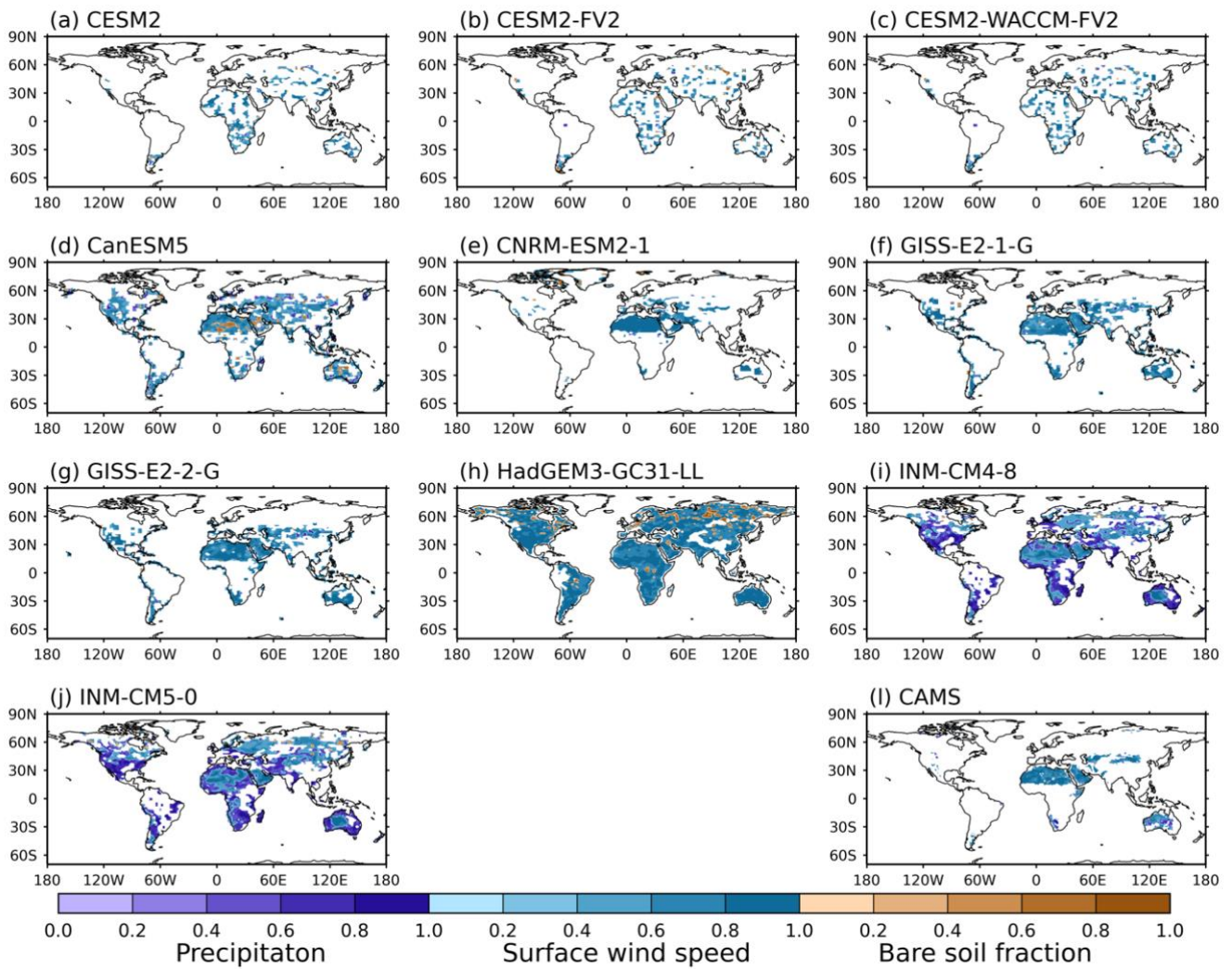
760 Figure 5: The dominant driver of dust emission and its relative importance (scaled to 0-1) in (a-k) models and (l) CAMS reanalysis. Purple for precipitation, blue for surface wind speed, and brown for bare soil fraction. Data used for regressions are 30 years (1985-2014) for models and 10 years (2005-2014) for CAMS due to data availability. Surface wind speed and precipitation in panel (l) are taken from ERA5.
