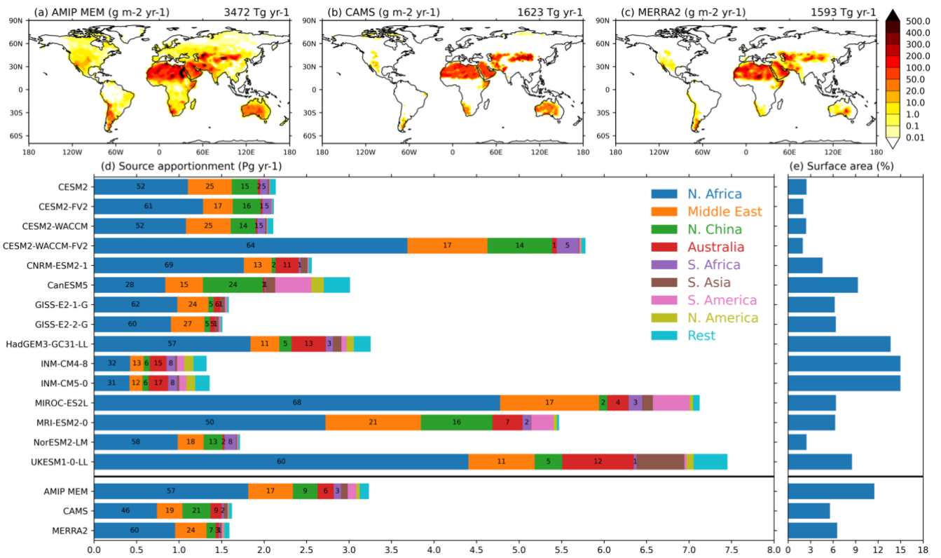
Figure 3: Intercomparison of 2005-2014 annual mean dust emissions between models and reanalyses. Maps show the annual mean dust emissions ( \text{g m}^{-2} \text{ yr}^{-1} ) from (a) AMIP MEM, (b) CAMS and (c) MERRA2. The numbers on the top right of each panel denote the global total dust emission budget ( \text{Tg yr}^{-1} ). The global annual total dust emission budgets (d; \text{Pg yr}^{-1} ) and the fraction of total dust emission areas relative to the global surface area (e; %) are shown for each individual model as well as for the AMIP MEM, CAMS and MERRA2. The contributions of major dust source regions are coloured out in (d), where the percentage contributions of the first five largest source regions are given at the centres of each coloured bars.
