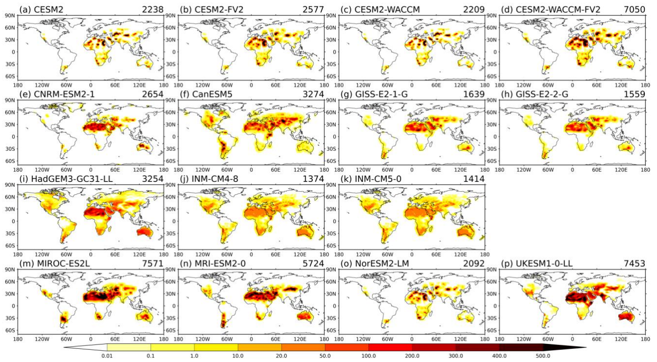
745 Figure 2: The CMIP6 AMIP models' simulated global annual mean (2005-2014) dust emission ( \text{g m}^{-2} \text{s}^{-1} ) climatology. The numbers on the top right of each panel denote the global total dust emission budget ( \text{Tg yr}^{-1} ).
