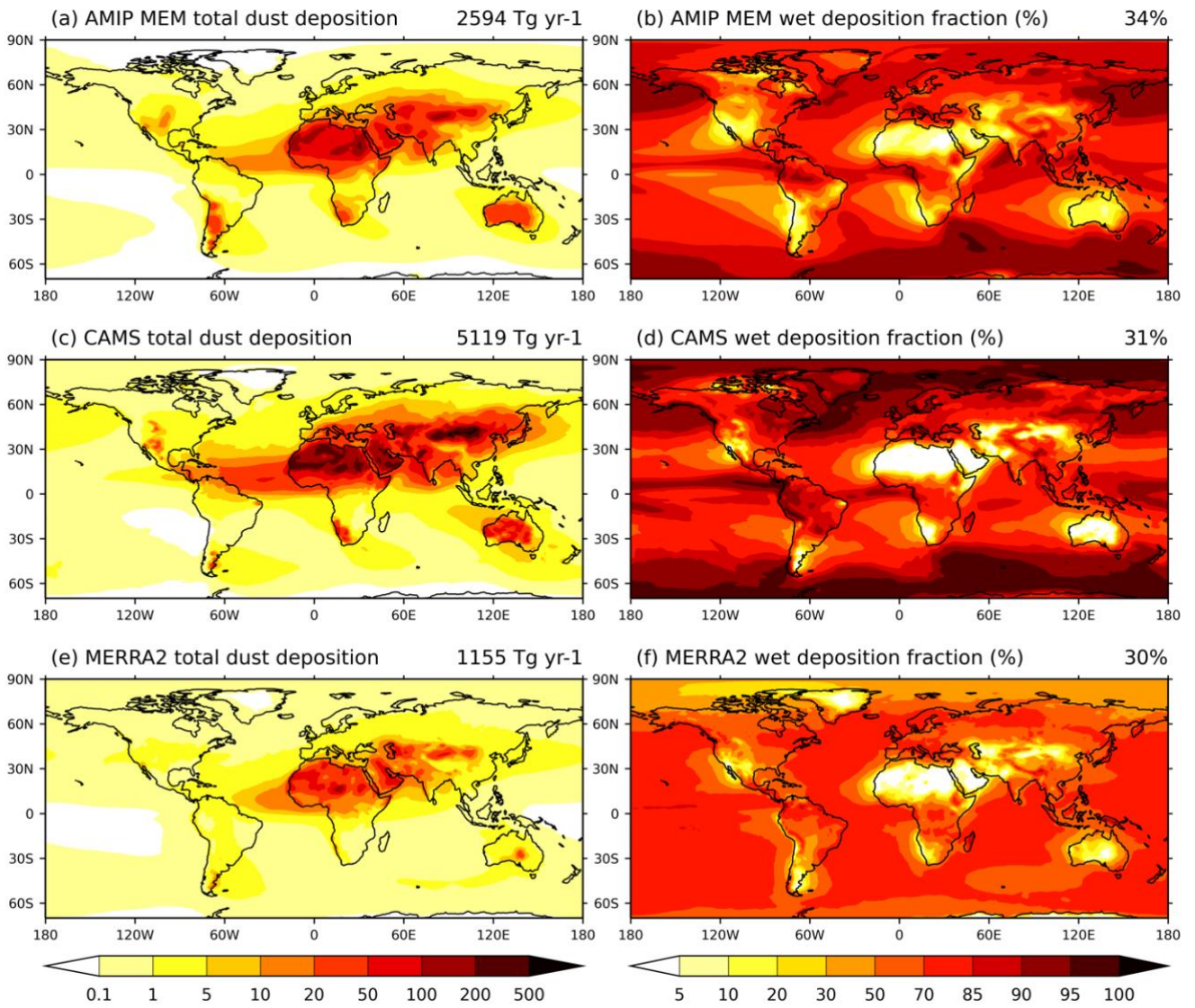
775 Figure 8: Intercomparison of 2005-2014 mean of annual total (dry + wet) dust deposition (left; \text{g m}^{-2} \text{yr}^{-1} ) and the ratio of wet-to-total depositions (right; %). Top row for AMIP MEM, middle for CAMS and bottom for MERRA2. The numbers on the top right of each panel denote the global total dust deposition flux ( \text{Tg yr}^{-1} ) and the fraction of global wet-to-total dustdepositions (%).
