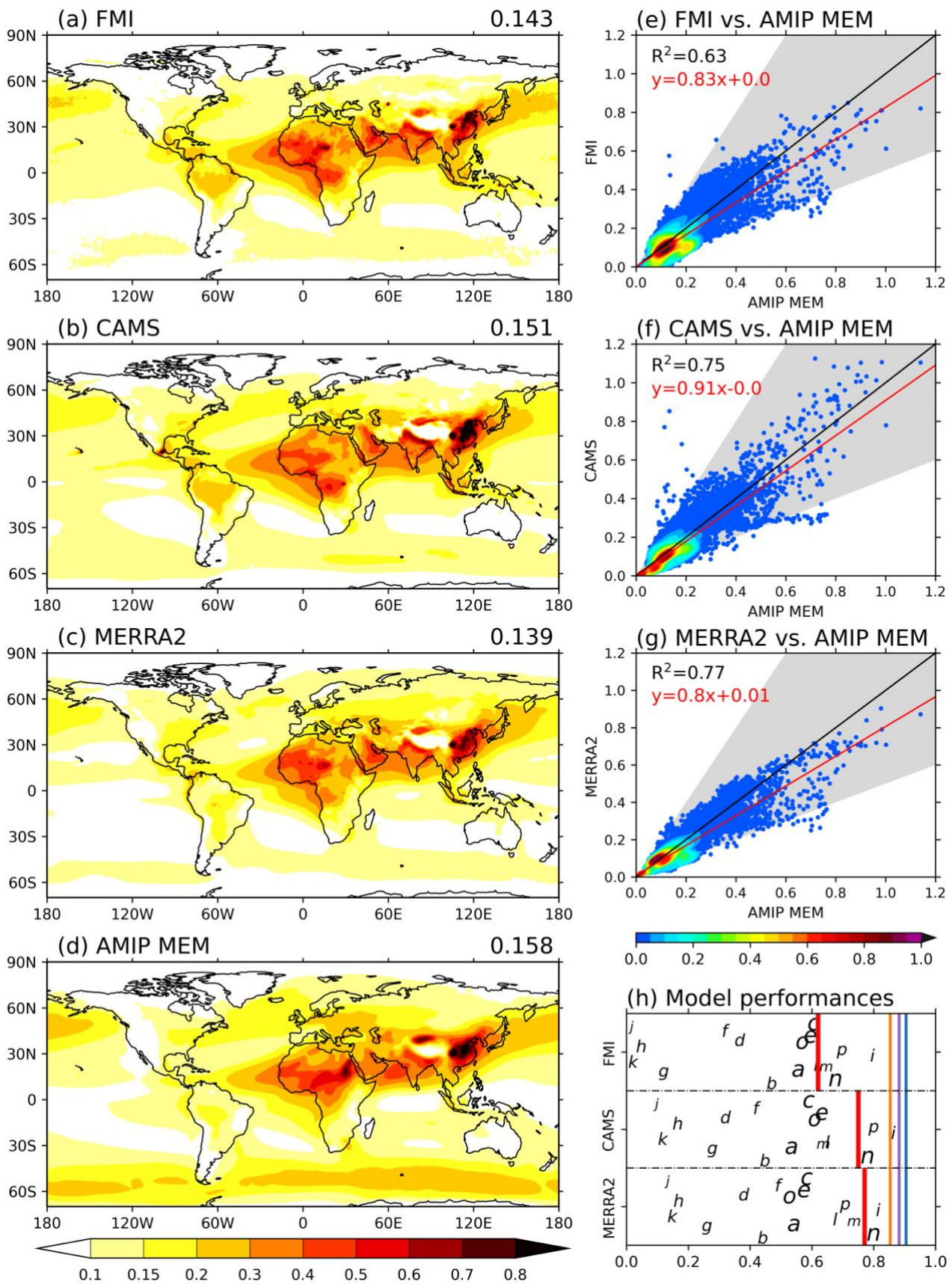
Figure 11: Intercomparison of 2005-2014 annual mean AOD from (a) FMI merged satellite retrievals, (b) CAMS, (c) MERRA2 and (d) AMIP MEM. (e-g) show the density ( 10^{-4} ) scatter plots of observation/reanalyses (a-c; y-axes) vs. AMIP MEM (d; x-axes); the black lines are the 1:1 correspondence while the red lines are the linear fitting ( R^2 and the regression equation given at top left corners). (h) is a summary of the performance of each individual model and observation/reanalyses. The Y-axes do not have any physical meaning, and is used to make the plot readable. Models are shown by letters (cf. Table 1). The red vertical bars denote where the AMIP MEM stands. The blue vertical bar shows the spatial R^2 between CAMS and FMI. Similarly, orange bars for MERRA2 vs. FMI, and purple for CAMS vs. MERRA2.
