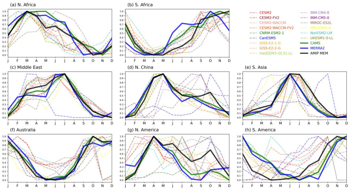
755 Figure 4: Normalised seasonal cycles of dust emissions over the eight dust source regions. Dashed curves represent individual models, while the AMIP MEM is shown in solid black. Also shown are results from CAMS (solid green) and MERRA2 (solid blue). The absolute dust emission seasonal cycles are included in Supplementary Figure S1.
