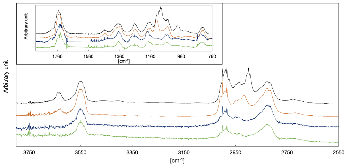
Figure 5. FTIR spectra of the residuals assigned to 2HPr obtained in the 1080 L chamber (green) and 480 L chamber (blue) 3\text{P2} + \text{OH} experiments and residuals obtained from the ozonolysis of 3-penten-2-ol (brown) and 3-buten-2-ol (black).
