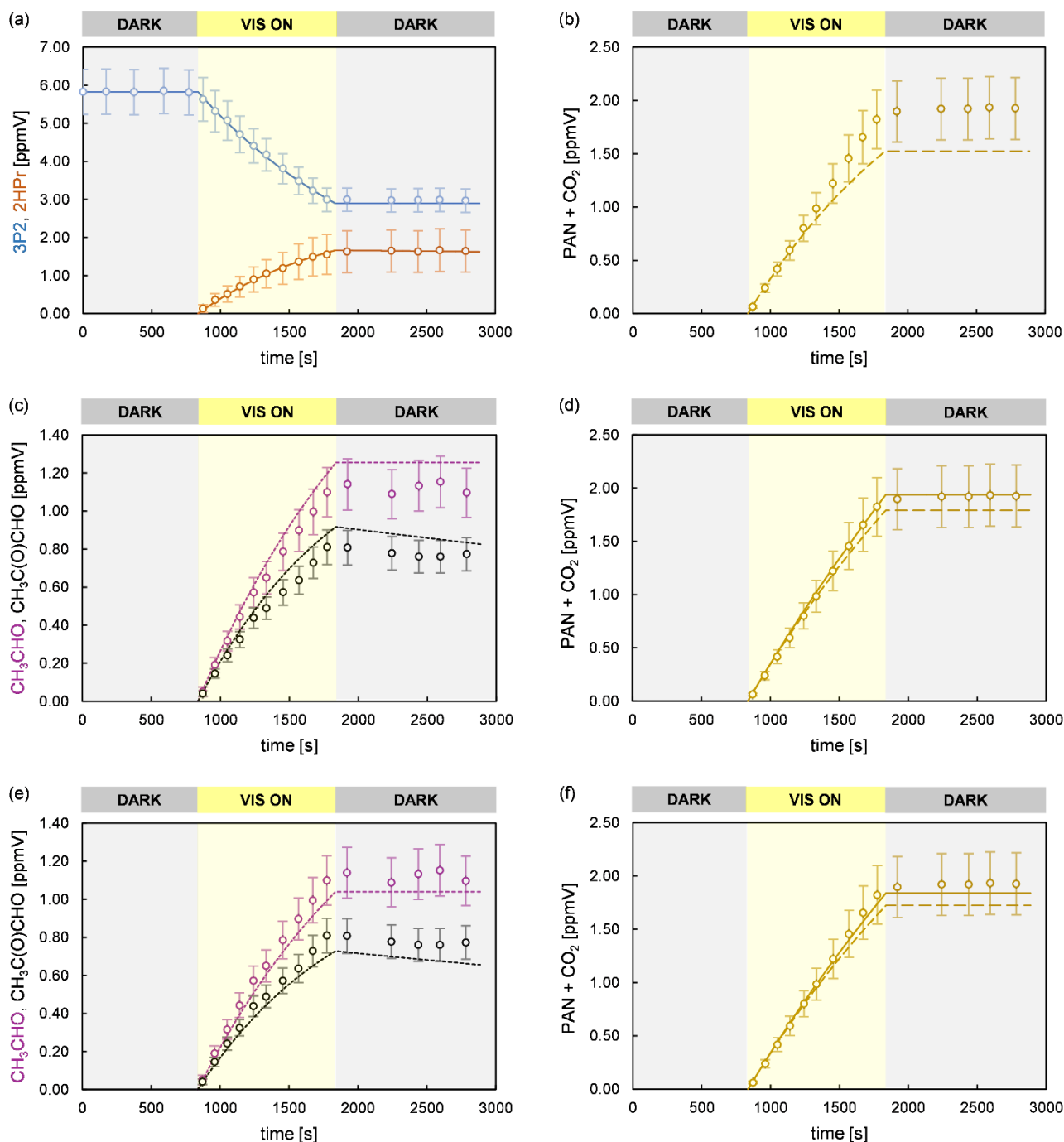
Figure 8. Experimental (circles) and simulated (lines) temporal behaviour of 3P2, 2HPr, acetaldehyde, methyl glyoxal and PAN + CO 2 in an experiment performed in the 480 L chamber. The error bars of the experimental data represent the accuracy error. Model runs of the sum parameter PAN + CO 2 are shown considering only the formation of PAN and CO 2 due to CH 3 C(O) radicals formed in the reaction system (dashed line) and including additionally the CO 2 source from 2HPr + OH (solid line). The model run in panel (b) considers only primary PAN and CO 2 formation from 3P2 + OH. Panel (c) and (d) represent model runs according to scenario 3 (acetaldehyde and methyl glyoxal
