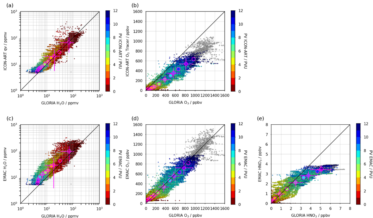
Figure 11. Correlation of GLORIA H_2O , O_3 and HNO_3 to corresponding ICON-ART and EMAC output variables. The large data points framed in magenta are a binned representation of the small data points. Magenta bars indicate the standard deviation of the binned data points. Colour-coding: PV from corresponding model.
