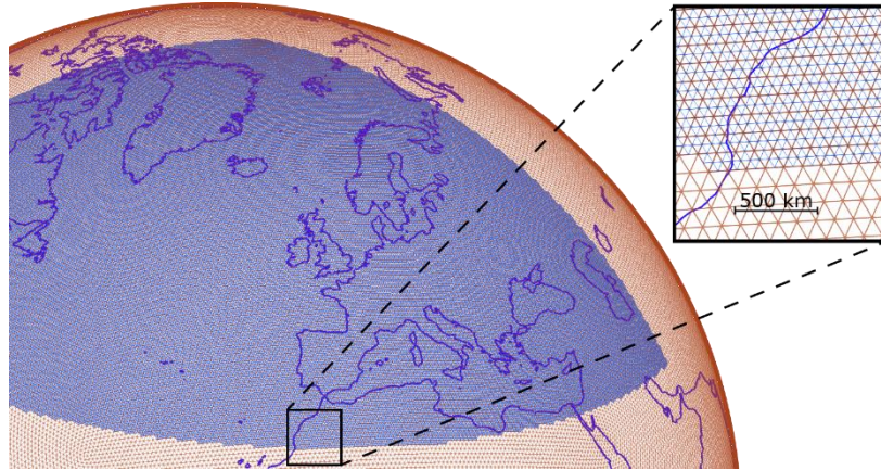
Figure 2. For the POLSTRACC winter, a global ICON-ART simulation with a global R2B6 grid was carried out (red). In the area of the flights, a nest with a R2B7 grid with \sim 20 km horizontal grid spacing was used to resolve mesoscale processes in more detail (blue).
