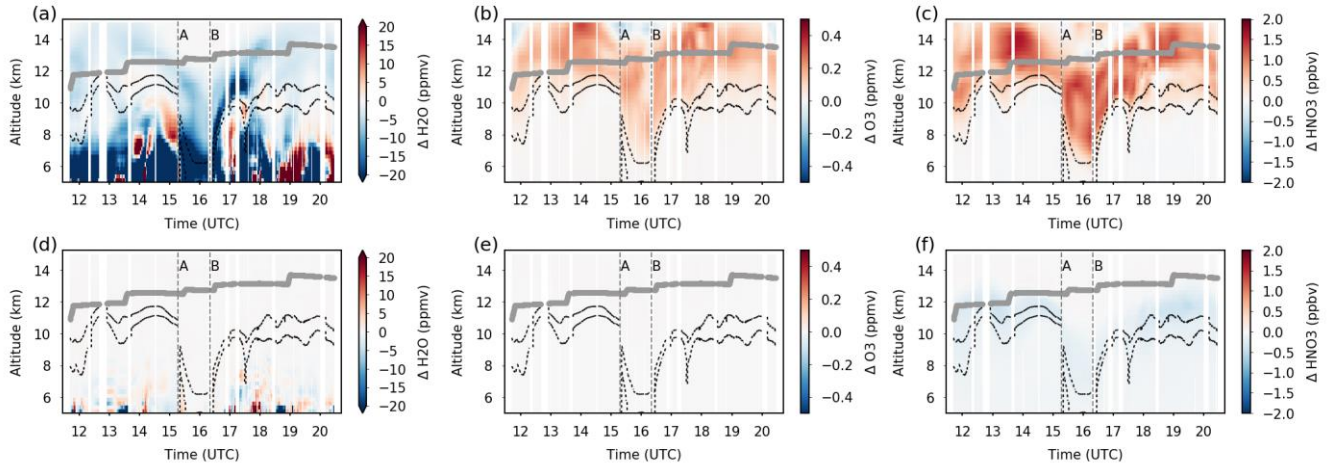
Figure 13. Modelled differences in H 2 O, O 3 and HNO 3 due to lower resolution (a-c, T106 minus T42 resolution) and neglecting scavenging processes in clouds (d-f, EMAC-STD minus EMAC-NOSCAV). Black dashed lines: EMAC 2 PVU and 4 PVU isolines (lower and higher lines, respectively) as indicators for the dynamical tropopause. Grey lines: HALO flight altitude.
