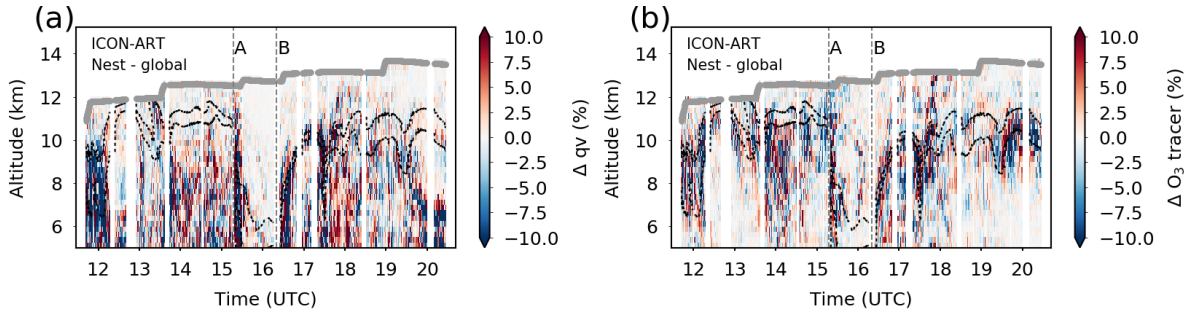
Figure 8. Residuals between the ICON-ART nested R2B7 and global R2B6 domains of q_v (a) and O_3 (b). Black lines: 2 PVU and 4 PVU isolines as indicators for the dynamical tropopause. Grey lines: HALO flight altitude.
