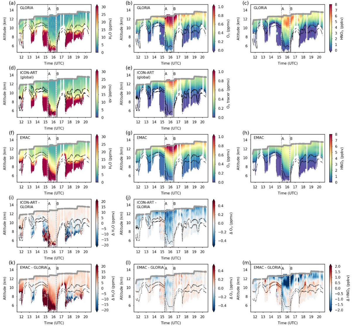
Figure 7. Observed and modelled trace gas distributions. GLORIA observations of water vapour, ozone and nitric acid (a-c). ICON-ART (global R2B6 grid) short-term forecast of specific humidity (d) and free-running simulation of ozone using simplified ozone depletion parameterisation (e). EMAC free-running simulations of water vapour, ozone and nitric acid (f-h). Residuals between the shown model data and GLORIA observations above (i-m). Black lines: 2 PPU and 4 PPU isolines (lower and higher lines, respectively) from ECMWF reanalysis (a-c), ICON-ART (d,e) and EMAC (f-h) as indicators for the dynamical tropopause. Grey lines: HALO flight altitude.
