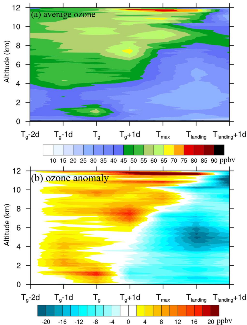
305 Figure 5: (a) Vertical ozone concentrations (unit: ppbv) at each typhoon developmental stage averaged over the typhoon ensemble over 2014-2018 at Taiwan. (b) Anomaly of vertical ozone concentrations relative to T_g-2d stage of the subsequent typhoon developmental stages. The temporally dense ozone profiles are available from the airborne observations of atmospheric compositions under the IAGOS framework collected at Taoyuan International Airport of Taiwan.
