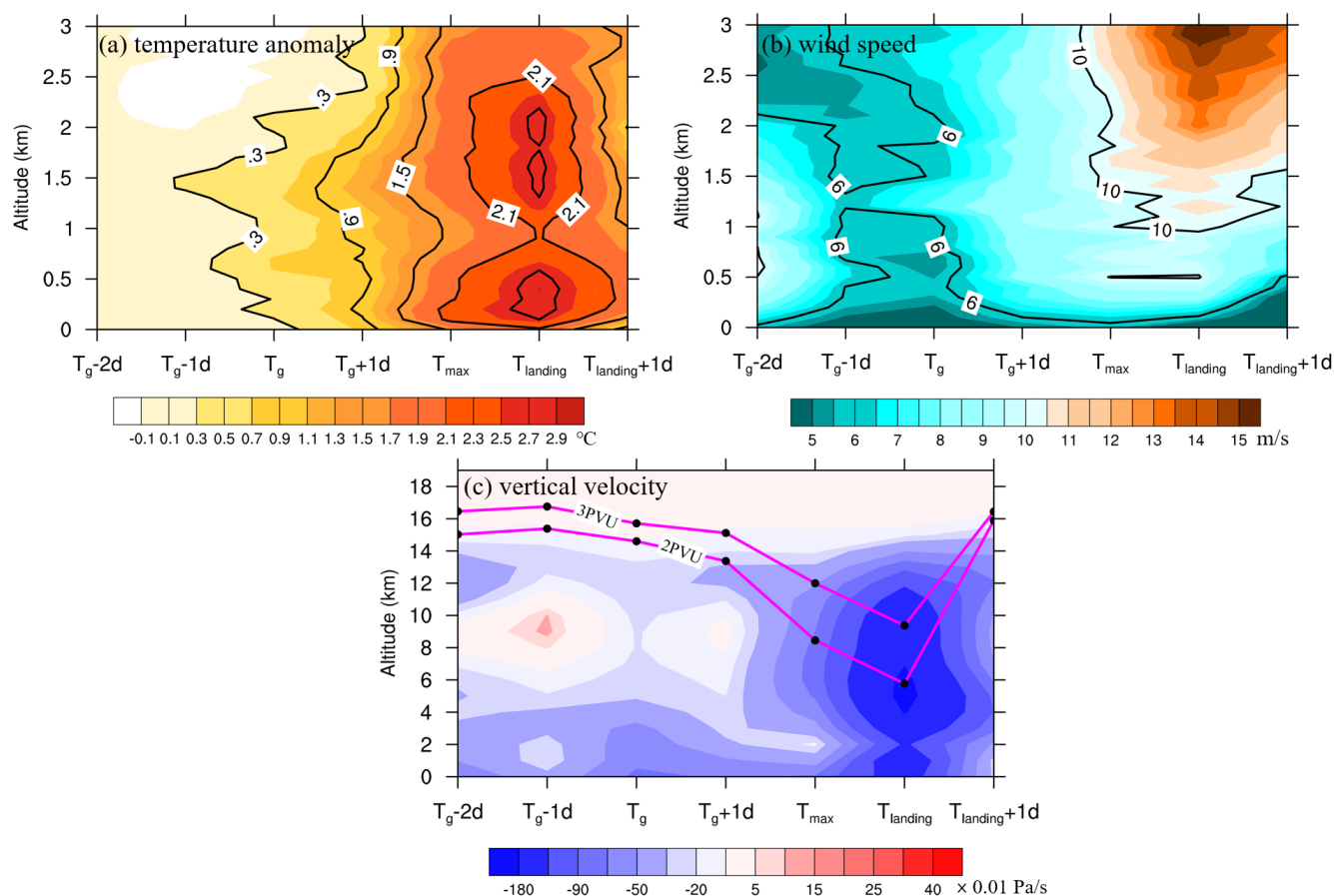
Figure 6: (a) Temperature anomaly relative to T_{g-2d} (unit: ^{\circ}C ) and (b) wind speed at each typhoon-developmental stage within the boundary layer using the simultaneous flight observations at Taoyuan International Airport of Taiwan. (c) Vertical velocity (shaded, unit: 0.01 Pa/s ) and the average height of 2-PVU (potential vorticity units, 1 PVU = 10^{-6} m^2 s^{-1} K kg^{-1} ) and 3-PVU regions. The data are averaged over the large ensemble of typhoons over 2014-2018.
