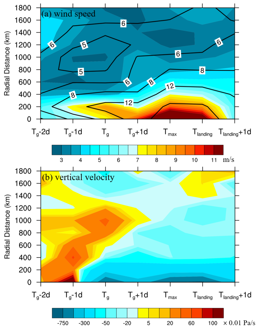
Figure 4: Same as Fig. 3, but for nighttime (0200 LST).
