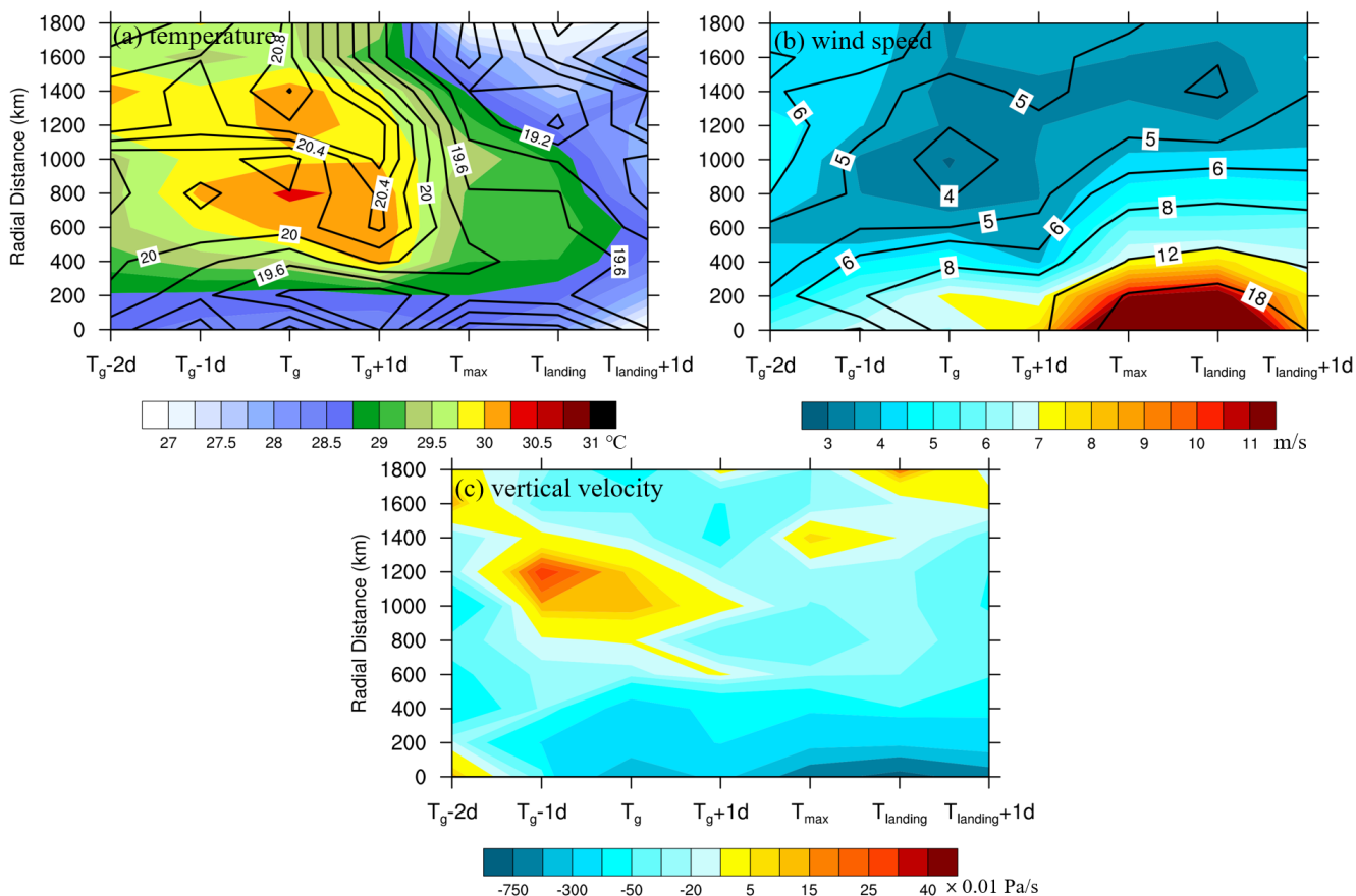
250 Figure 3: (a) 10-m (shaded) and 850-hPa (contour lines) air temperature (unit: °C), (b) 10-m (shaded) and 850-hPa (contour lines) wind speed (unit: m/s) and (c) 500-hPa vertical wind velocity (unit: 0.01 Pa/s, positive values for downward air motions and vice versa) at daytime (1400 LST) based on MERRA-2 reanalysis at different radial distances and typhoon developmental stages averaged over the large ensemble of typhoons over 2014-2018.
