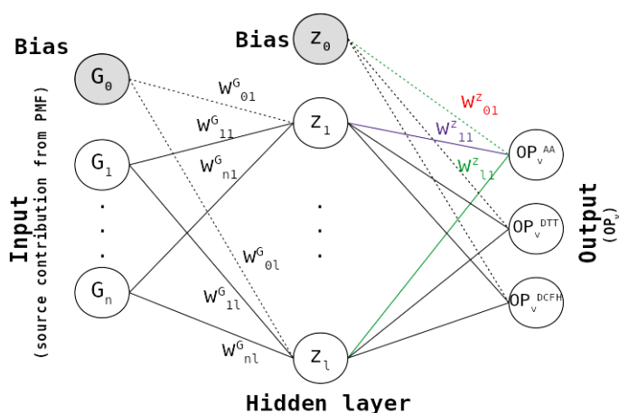
215 Figure 2: The MLP neural network architecture used in this study, where n refers to the number of source, G is the normalized contribution from the PMF, and OP_v is the different volume-normalized OP activities ( OP_v^{DTT} , OP_v^{AA} , and OP_v^{DCFH} )
