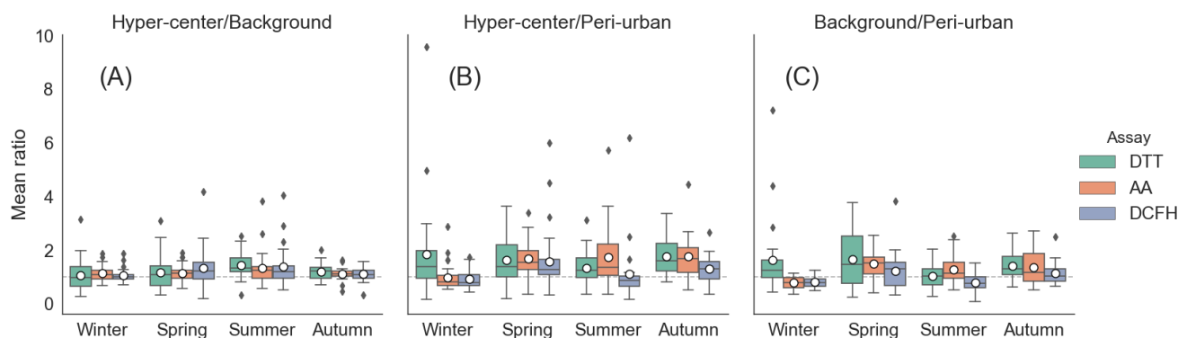
300 Figure 3: Seasonal mean ratios (MR) between the sites ((A) Hyper-center/Background (UH/UB), (B) Hyper-center/Peri-urban (UH/PU), and (C) Background/Peri-urban (UB/PU)) using volume-normalized OP activities ( OP_v^{DTT} , OP_v^{AA} , and OP_v^{DCFH} ). Dashed grey line denotes MR equal to 1 suggesting total spatial homogeneity. Boxplot mean marked by white circle and median marked by black line.
