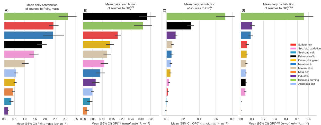
Figure 6: Overall daily mean OP_v contribution of the sources to PM_{10} , OP_v^{DTT} , OP_v^{AA} , and OP_v^{DCFH} using MLR analysis in the form of mean and 95% confident interval of the mean (error bar) (n=378 samples).
