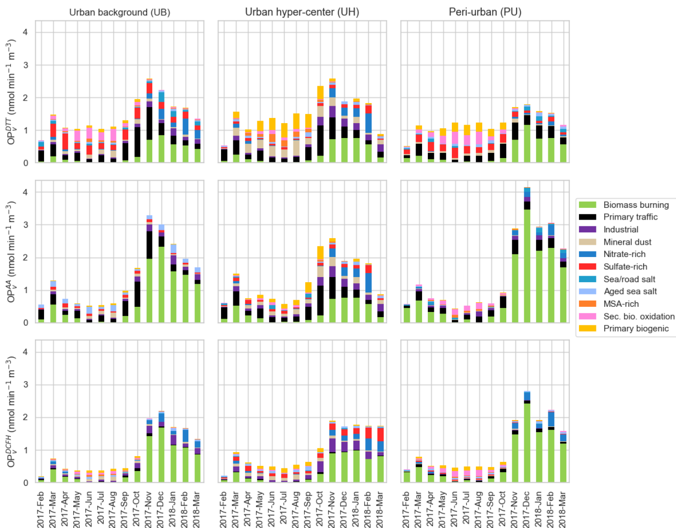
430 Figure 7: The monthly mean OP_v contributions of each PM_{10} source in the three urban sites in Grenoble, France for OP_v^{DTT} , OP_v^{AA} , and OP_v^{DCFH} .
