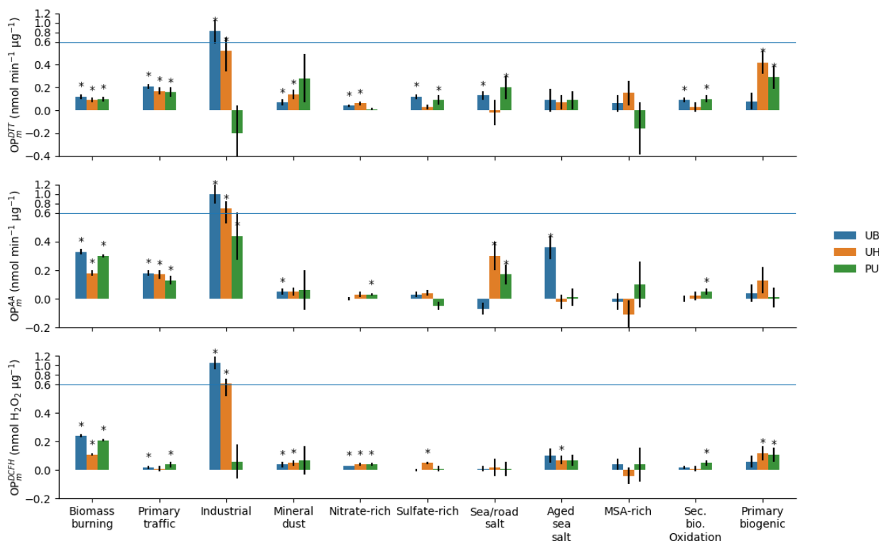
340 Figure 5: Site-specific intrinsic OP ( OP_m ) per source analysis from each assay ( OP_m^{DTT} , OP_m^{AA} , and OP_m^{DCFH} ) represented by mean (bar) and standard deviation (error bar) based on the MLR (Urban background, UB: blue, Urban hyper-center, UH: orange, Peri-urban, PU: green). Note: Asterisks represent statistically significant OP_m within 95% confidence interval ( p\text{-value} \leq 0.05 ).
