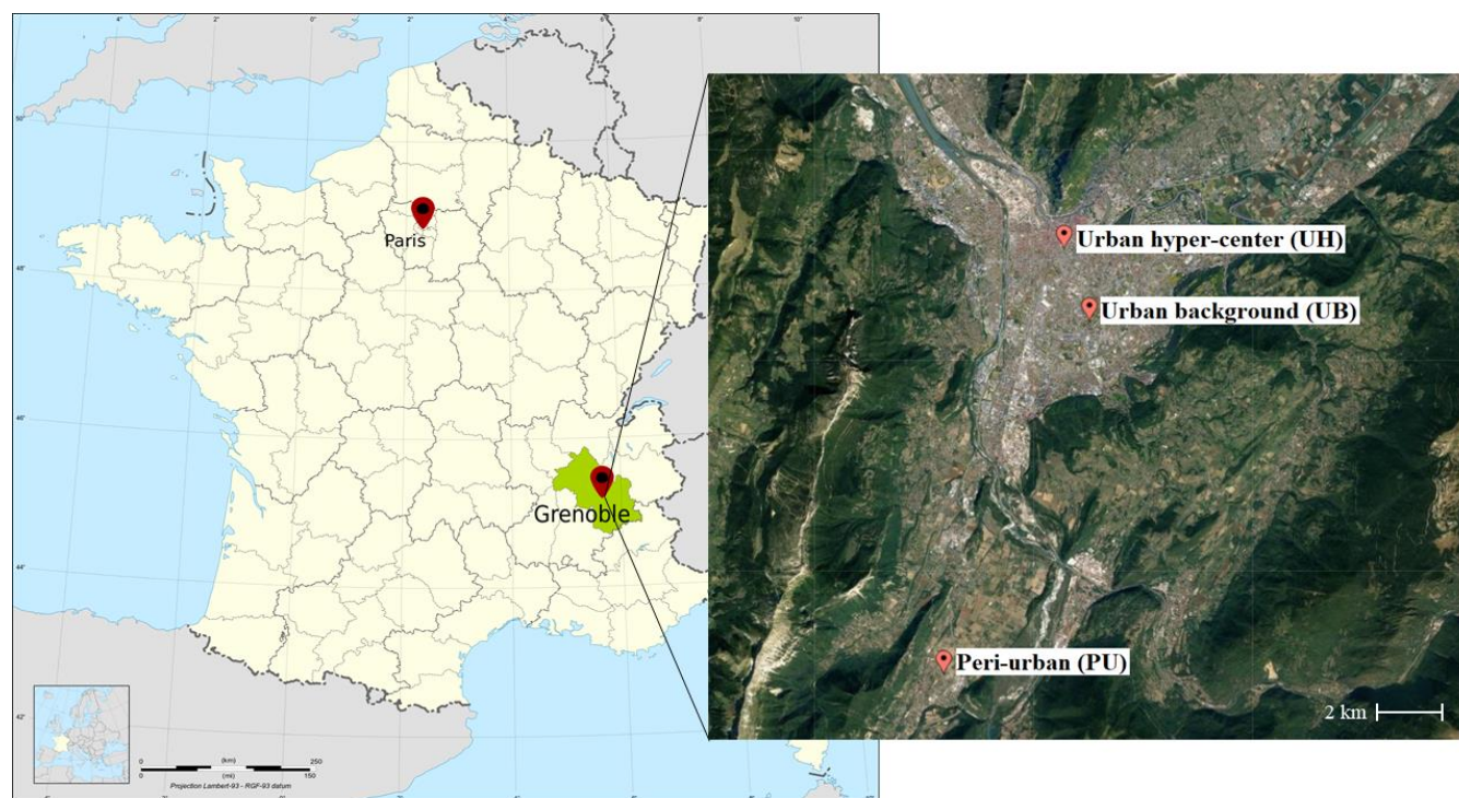
115 Figure 1: Study area in Grenoble (France) on a European map (left) and location of the three urban sites (right), namely Les Frères or UB (urban reference background site), Caserne de Bonne or UH (urban hyper-center site), and Vif or PU (peri-urban site). ©OpenStreetMap contributors 2020. Distributed under a Creative Commons BY-SA License
