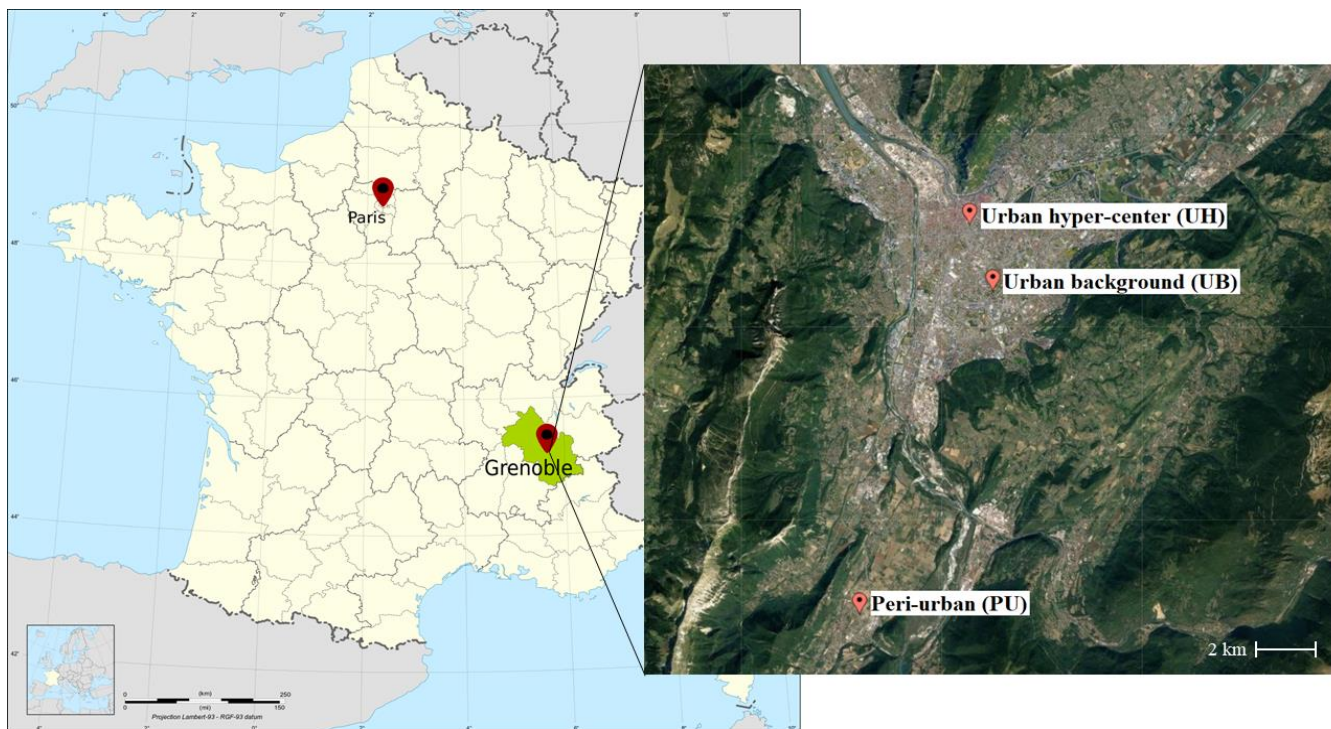
120 Figure 1: Study area in Grenoble (France) on a European map (left) and location of the three urban sites (right), namely Les Frênes or UB (urban reference background site), Caserne de Bonne or UH (urban hyper-center site), and Vif or PU (peri-urban site). ©OpenStreetMap contributors 2020. Distributed under a Creative Commons BY-SA License
