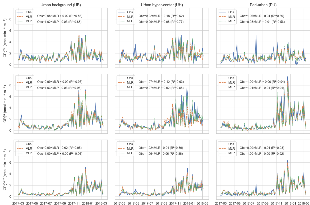
325 Figure 4: Comparison of the observed and modelled OP_v ( OP_v^{DTT} , OP_v^{AA} , and OP_v^{CFH} ) at different urban sites using MLR and MLP models. The equation of the line and goodness-of-fit ( R^2 ) between observed and modelled OP are included.
