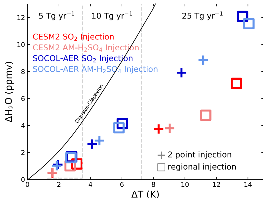
5 Figure 11: Scatter plot of water vapor change (ppmv) relative to change in temperature (K) at 90 hPa and averaged between 30° S and 30° N for injections of 5, 10, and 25 Tg(S) yr -1 of SO 2 or AM-H 2 SO 4 . Results from CESM2 and SOCOL-AER only are shown, as the MAECHAM5-HAM model used fixed H 2 O.
