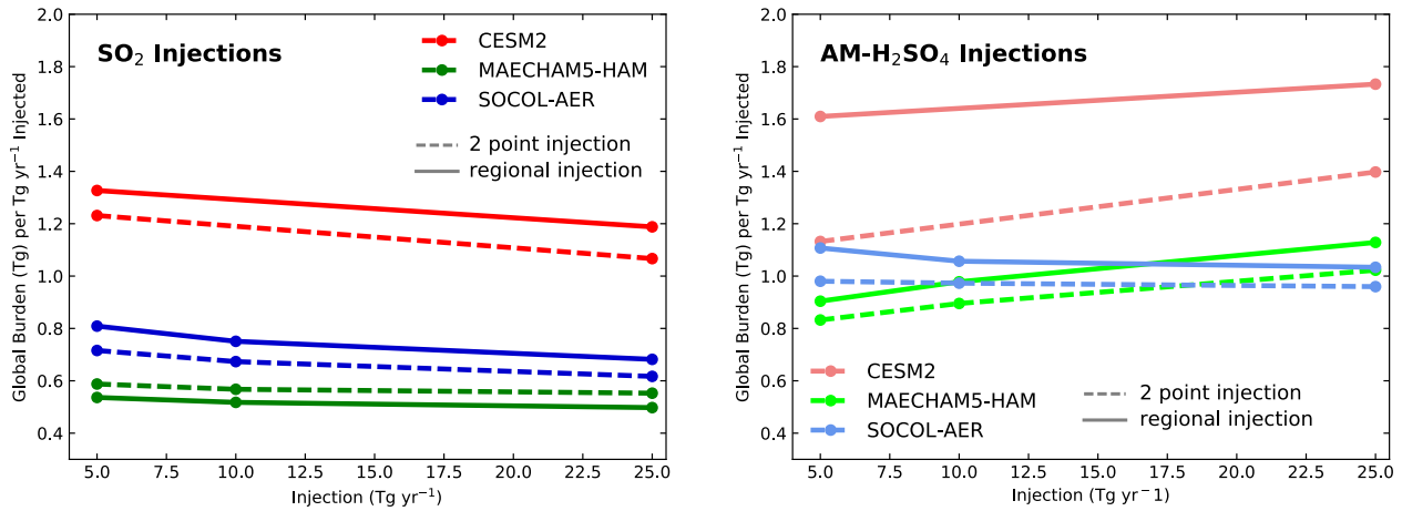
Figure 3: Increase in global sulfuric acid aerosol burden normalized by geoeengineering injection rate in units of \text{Tg(S) per (Tg(S) yr}^{-1}) as a function of injection rate. The y-axis also represents the residence time in years of injected sulfur as aerosol. \text{SO}_2 injections (left panel) show decreasing residence time with increasing injection rate whereas \text{AM-H}_2\text{SO}_4 injections (right panel) show increasing residence time with increasing injection rate for the CESM2 and MAECHAM5-HAM models. Regional injections (solid lines) show longer residence times than 2point injections (dashed lines) in most cases.
