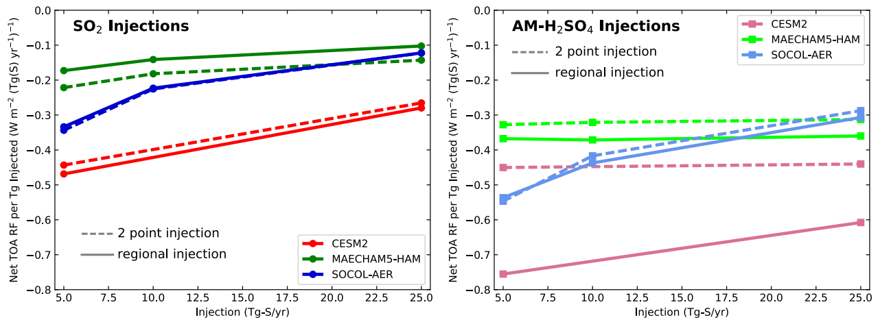
Figure 7: Globally averaged change in net top-of-atmosphere shortwave+longwave radiative forcing ( \text{W m}^{-2} ) per unit annual injection ( \text{Tg(S) yr}^{-1} ) due to geengineering injection as a function of injection rate for (left panel) \text{SO}_2 injections and (right panel) \text{AM-H}_2\text{SO}_4 injections.
