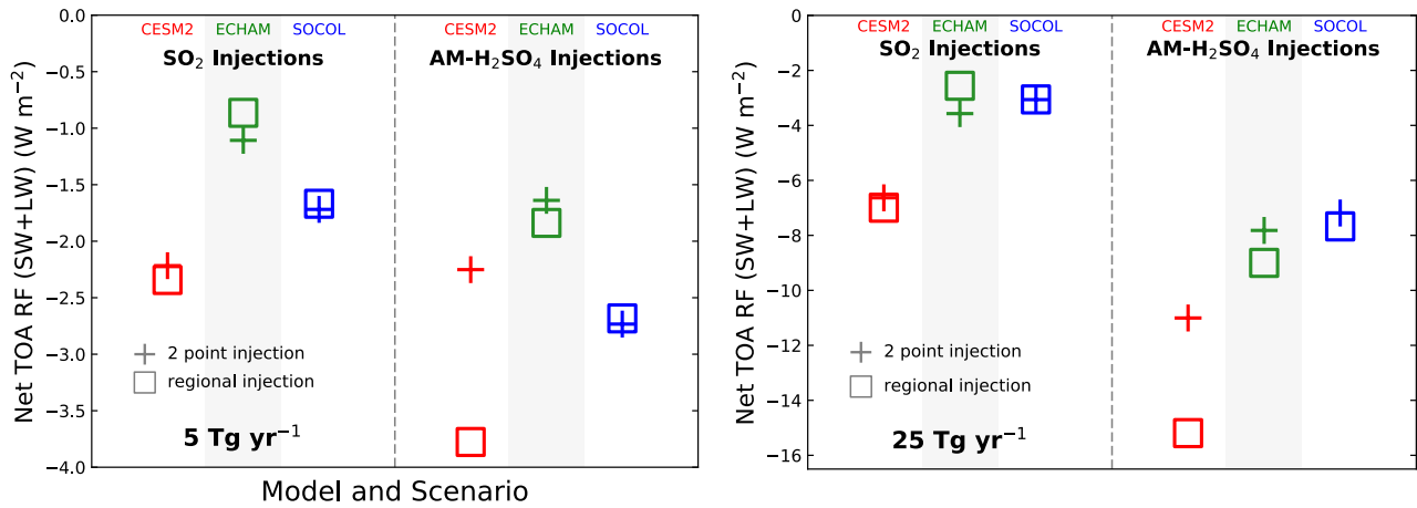
Figure 6: Globally averaged change in net top-of-atmosphere shortwave+longwave radiative forcing ( W m^{-2} ) due to geoengineering injection of (left panel) 5 Tg(S) yr -1 and (right panel) 25 Tg(S) yr -1 . Colors and symbols as in Figure 1.
