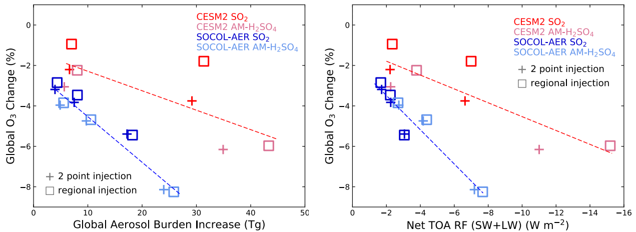
Figure 13: Global average change in column ozone (%) due to geoengineering injection plotted against (left panel) the global average aerosol burden increase (Tg(S)), and (right panel) the average change in SW+LW radiative forcing ( \text{W m}^{-2} ). Regression lines are shown for each model with R^2 values of 0.95 and 0.90 for SOCOL-AER (burden and RF, respectively) and of 0.58 and 0.72 for CESM2.
