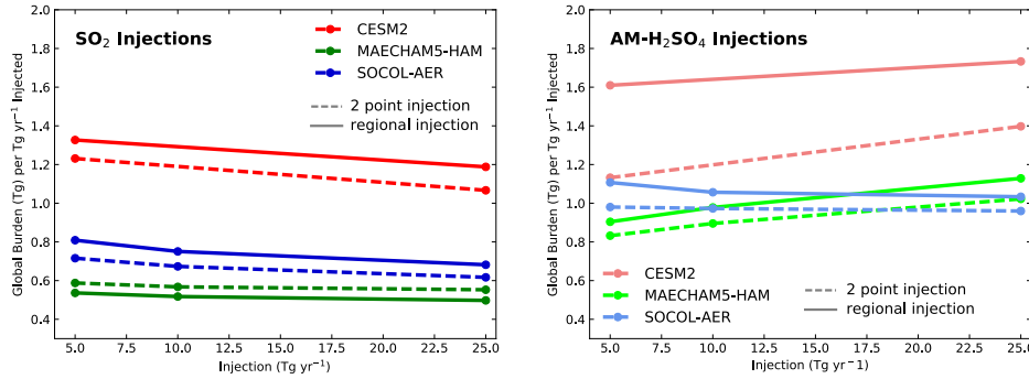
10 Figure 3: Increase in global sulfuric acid aerosol burden normalized by geoengineering injection rate in units of \text{Tg(S) per (Tg(S) yr}^{-1}) as a function of injection rate. The y-axis also represents the residence time in years of injected sulfur as aerosol. \text{SO}_2 injections (left panel) show decreasing residence time with increasing injection rate whereas \text{AM-H}_2\text{SO}_4 injections (right panel) show increasing residence time with increasing injection rate for the CESM2 and MAECHAM5-HAM models. Regional injections (solid lines) show longer residence times than 2-point injections (dashed lines) in most cases.
