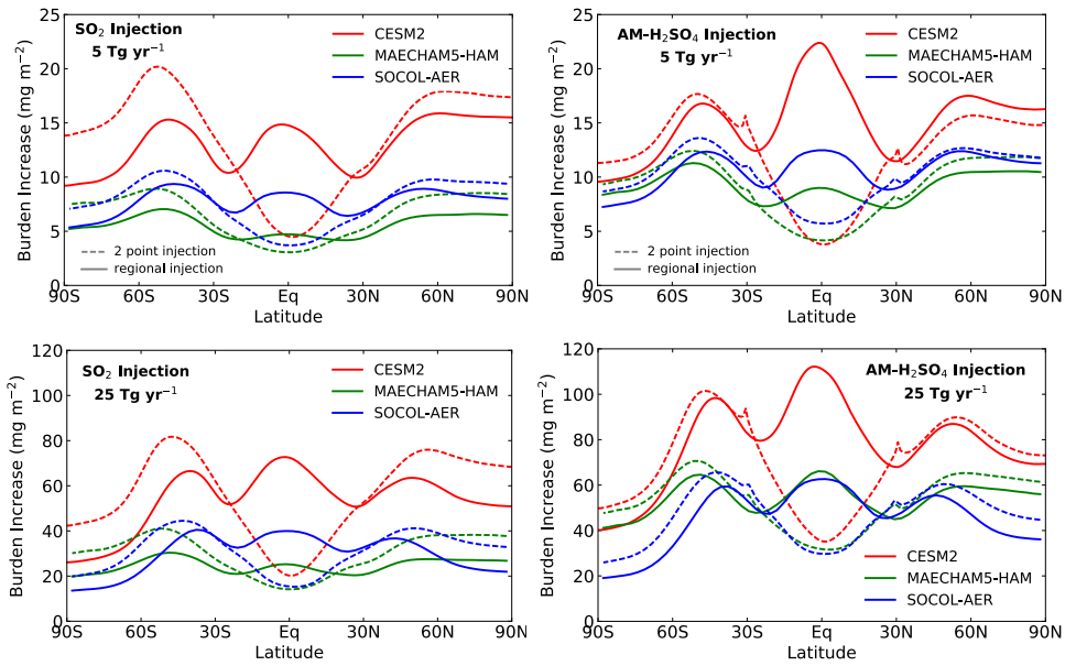
Figure 2: Zonal mean aerosol column burden increase above background ( \text{mg m}^{-2} ) with 5 \text{ Tg(S) yr}^{-1} injections (top panels) and 25 \text{ Tg(S) yr}^{-1} injections (bottom panels) as a function of latitude for \text{SO}_2 injections (left panels) and \text{AM-H}_2\text{SO}_4 injections (right panels). Regional injections are shown with solid lines and 2point injections with dashed lines.
