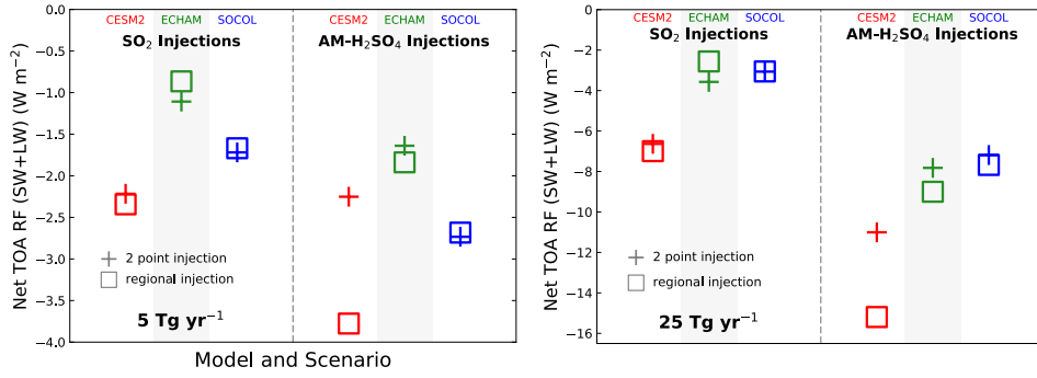
Figure 6: Globally averaged change in net top-of-atmosphere shortwave+longwave radiative forcing ( W m^{-2} ) due to geoengineering injection of (left panel) 5 Tg(S) yr^{-1} and (right panel) 25 Tg(S) yr^{-1} . Colors and symbols as in Figure 1.
