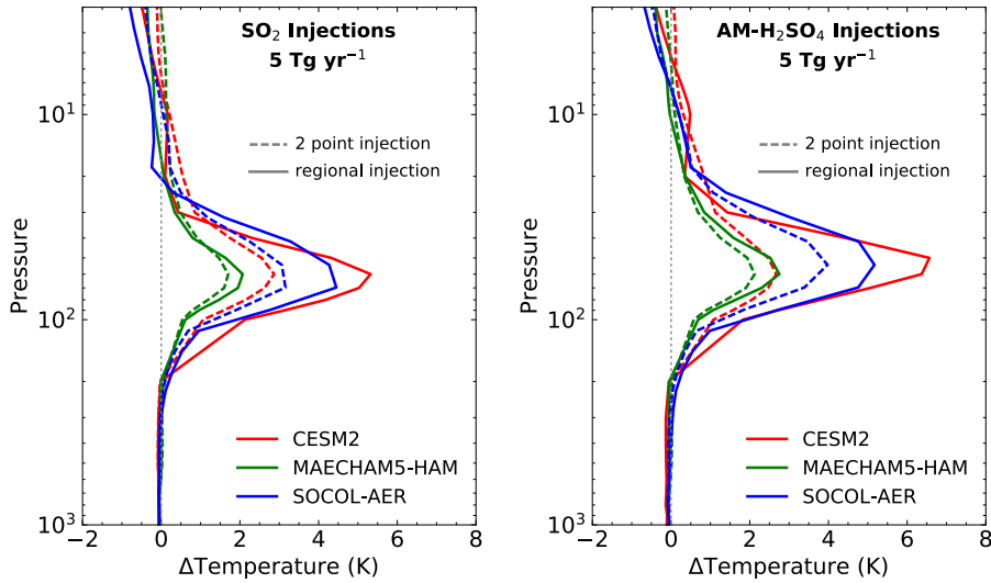
5] Figure 10: Change in atmospheric temperature (K) averaged between 30°S and 30°N due to 5 Tg(S) yr -1 of geoengineering injection as a function on height for (left panel) injections of SO 2 , and (right panel) injections of AM-H 2 SO 4 .
