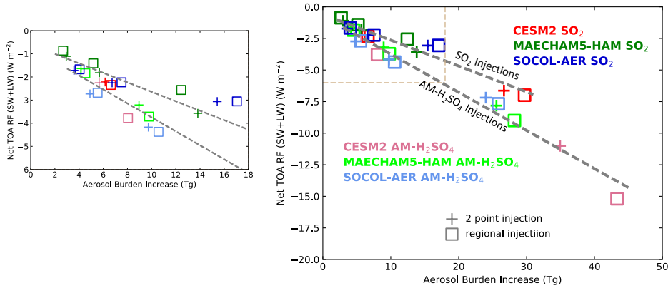
10] Figure 8: Scatter plot of globally averaged net TOA shortwave+longwave radiative forcing ( W m^{-2} ) due to geoengineering injection relative to the corresponding increase in global aerosol burden ( Tg(S) ). The smaller figure is finer scale for the upper left corner of the main plot. Regression lines are shown for SO 2 injections ( R^2=0.93 ) and for AM-H 2 SO 4 injections ( R^2=0.98 ).
