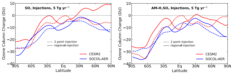
Figure 12: Average change in column ozone (Dobson units) due to geoengineering injection as a function of latitude for (left panel) 5 \text{Tg(S) yr}^{-1} of \text{SO}_2 injection and (right panel) 5 \text{Tg(S) yr}^{-1} of \text{AM-H}_2\text{SO}_4 injection.
