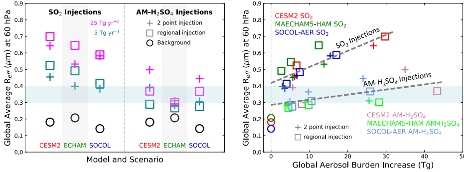
10 15 Figure 4: Global average effective radius (mm) at 60 hPa (left panel) for the 3 models with SO 2 injections of 5 and 25 Tg(S)/yr (left side) and with AM-H 2 SO 4 injections of 5 and 25 Tg(S)/yr (right side). Scatter plot of global average effective radius (mm) at 60 hPa plotted against the global increase in aerosol burden in Tg(S) (right panel), with AM-H 2 SO 4 injections shown with lighter symbols. Regression lines are shown for both SO 2 (R 2 =0.74) and AM-H 2 SO 4 (R 2 =0.34) injections. Injections into regions are shown by open squares, while injections at two points are shown with plus symbols, and for background conditions with open circles. The light blue shaded region represents the optimal effective radius for scattering of solar radiation assuming a lognormal distribution and s between 1.1 and 1.8 (Dykema et al., 2016; Dykema private communication).
