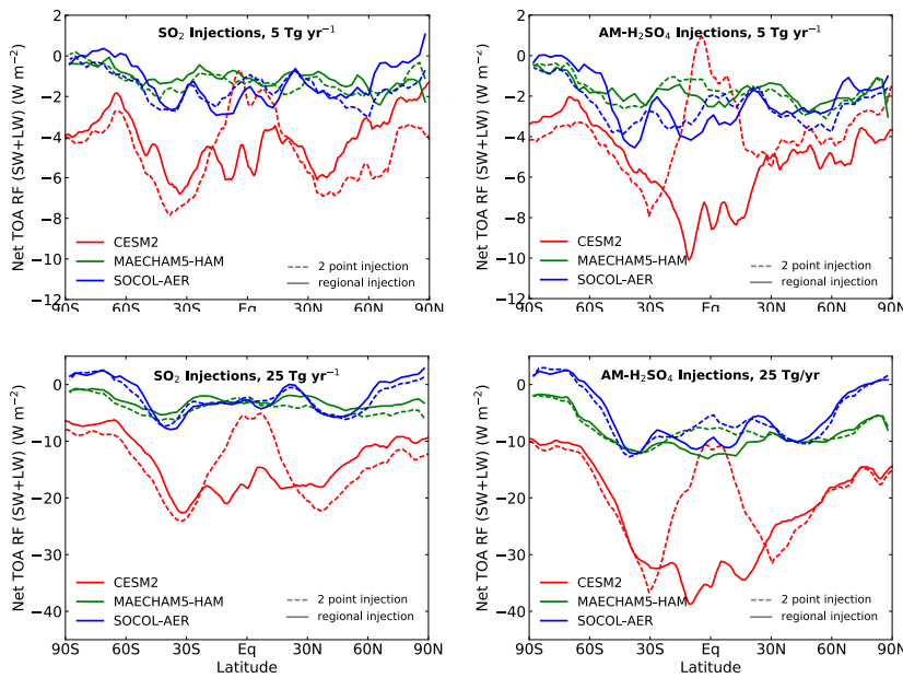
Figure 9: Zonal mean net top-of-atmosphere shortwave+longwave radiative forcing with 5 Tg(S)/yr injections (top panels) and 25 Tg(S)/yr injections (bottom panels) as a function of latitude for SO 2 injections (left panels) and AM-H 2 SO 4 injections (right panels). Regional injections are shown with solid lines and 2point injections with dashed lines.
