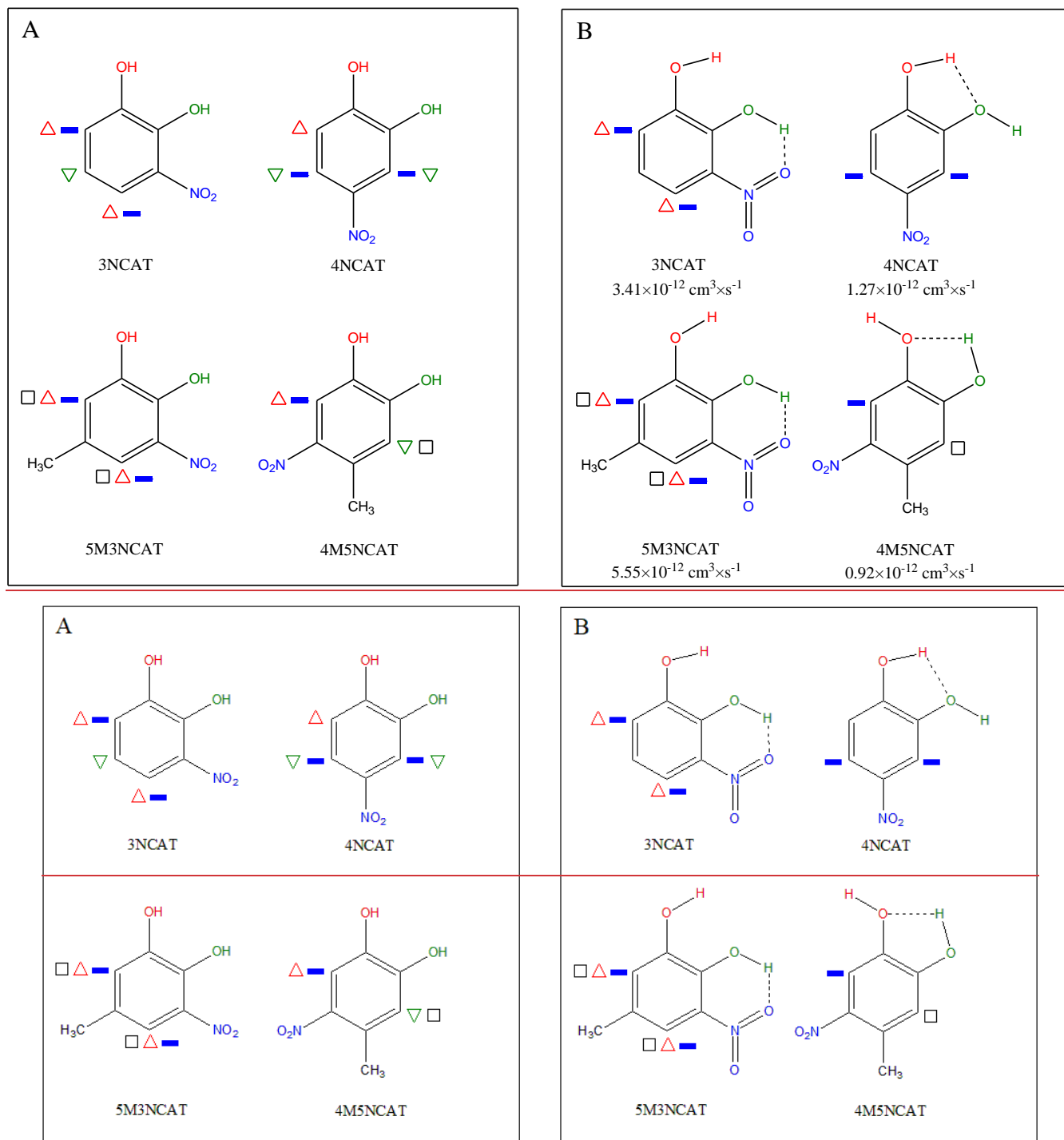
Figure 7: Electromeric effect distribution on the aromatic ring for the all investigating nitrocatechols in the present study:
