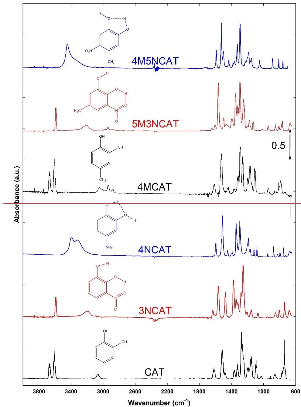
725 Figure 5: A - Gas-phase IR spectra of catechol (CAT), 3NCAT, 4NCAT; B - Gas-phase IR spectra of; 4-methylcatechol (4MCAT), 5M3NCAT; and 4M5NCAT.
