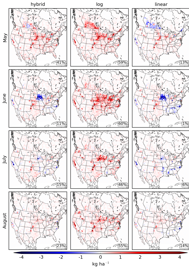
Figure 8. Monthly mean ammonia emissions increments for May to August 2016 on the GEM-MACH model grid for inversions using different observation operators. Inversions displayed in the left, middle, and right columns use the hybrid, log, and linear observation operators, respectively. The left column, which is identical to the right column of Fig. 3, is shown for comparison. Percentages in the lower right corners show the change over the whole domain.
