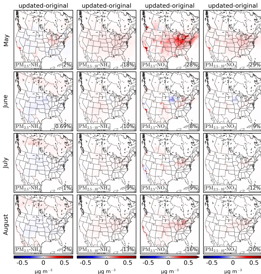
Figure 12. Monthly mean differences of GEM-MACH surface fields for fine (PM 2.5 ) and coarse-fraction (PM 2.5-10 ) ammonium and nitrate for May to August 2016 on the 0.09° × 0.09° model grid. 2016. Plots show mean differences between the run with the updated ammonia emissions and the original emissions. The total difference over the model domain as a percentage of the original field is shown in the lower right corner of each plot.
