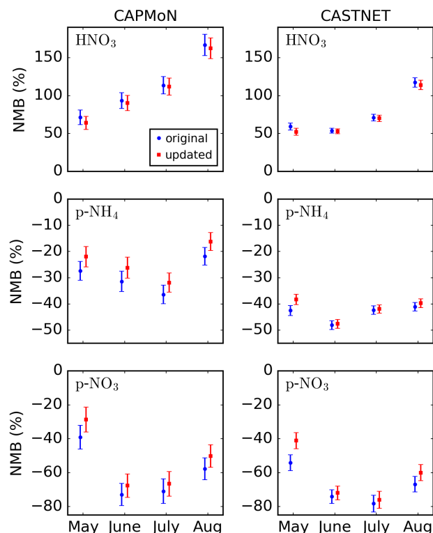
Figure 11. Normalized mean biases between GEM-MACH HNO 3 , p-NH 4 , and p-NO 3 surface fields and observations from the CAPMoN and CASTNET networks for May to August 2016. In the legend, ‘original’ and ‘updated’ indicate the ammonia emissions used in GEM-MACH. Error bars correspond to the standard error.
