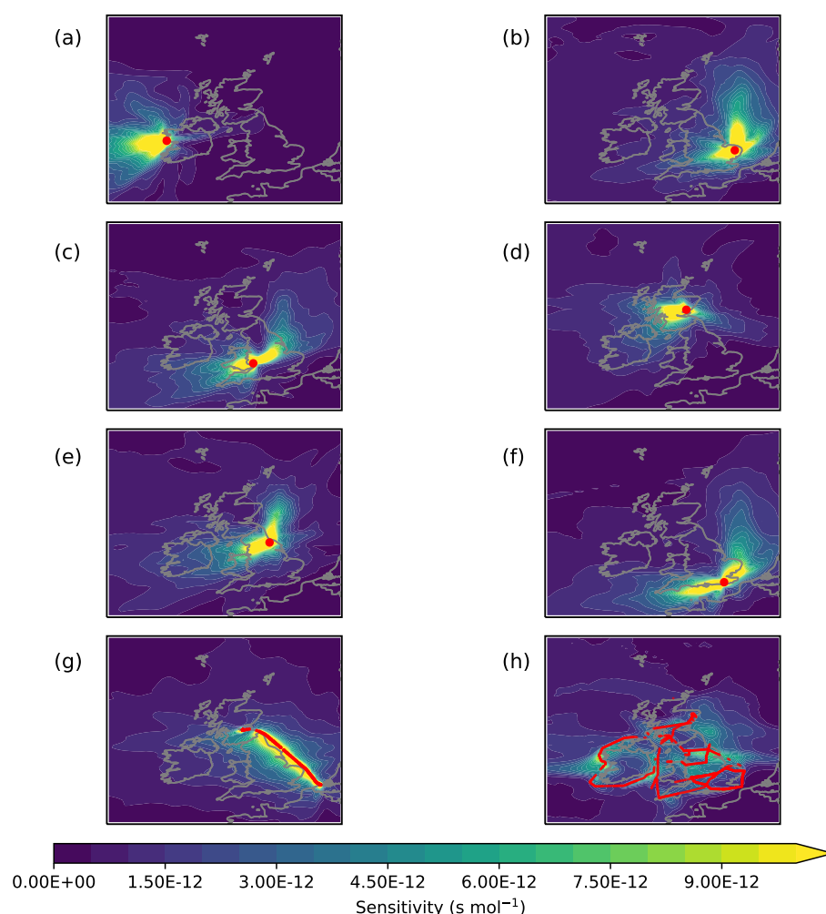
Figure 1. Annual mean NAME footprints for each of the measurement sites in 2015, showing the areas the measurements are most sensitive to (overall sensitivity extends much wider). (a) MHD, (b) TAC, (c) RGL, (d) TTA, (e) BSD, (f) HFD, (g) Ferry, (h) FAAM aircraft. Data for the FAAM aircraft (seven flights) are from 2014. Red dots show the measurement locations.
