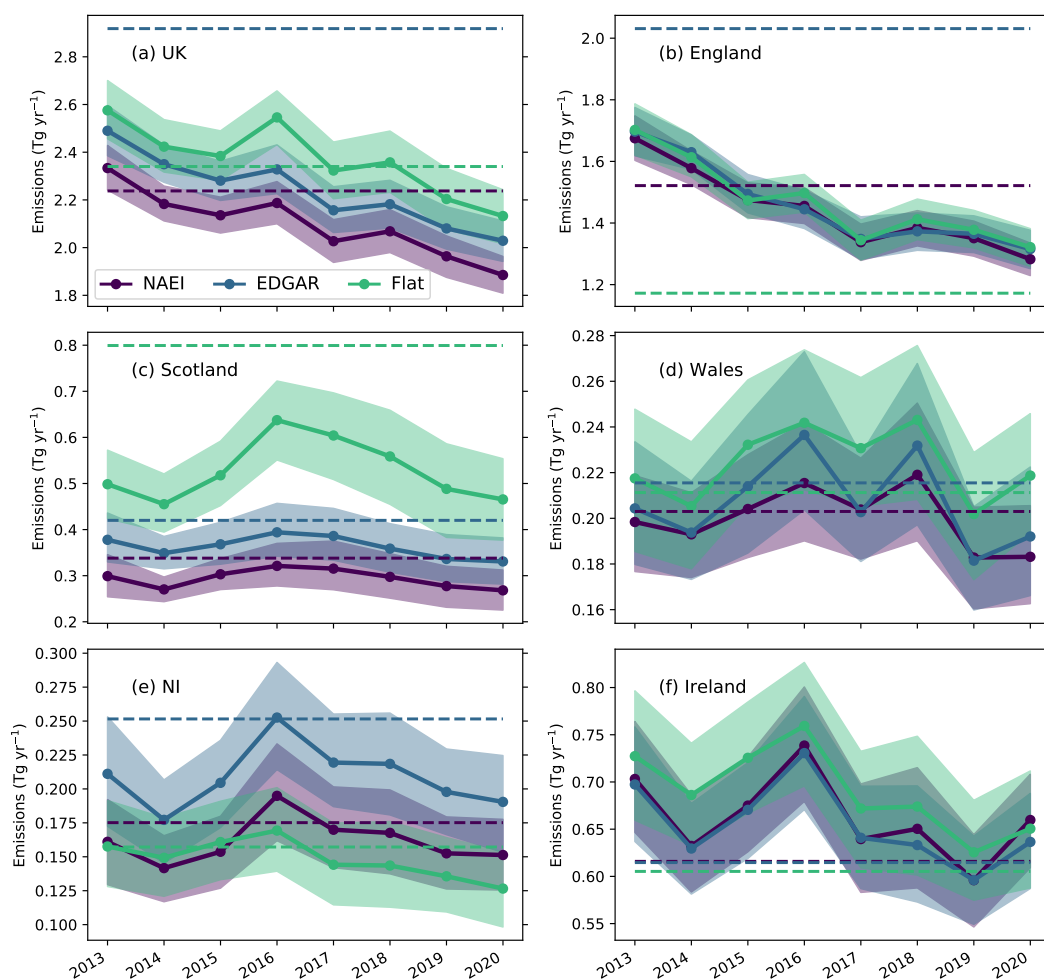
Figure 8. Annual mean emissions between 2013–2020 for inversions using different prior distributions from the NAEI (purple), EDGAR (blue) and a flat distribution (green). Estimates are shown for (a) the UK, (b) England, (c) Scotland, (d) Wales, (e) NI and (f) Ireland. Shading represents the 95% confidence interval. Dashed lines represent the magnitudes of the respective priors.
