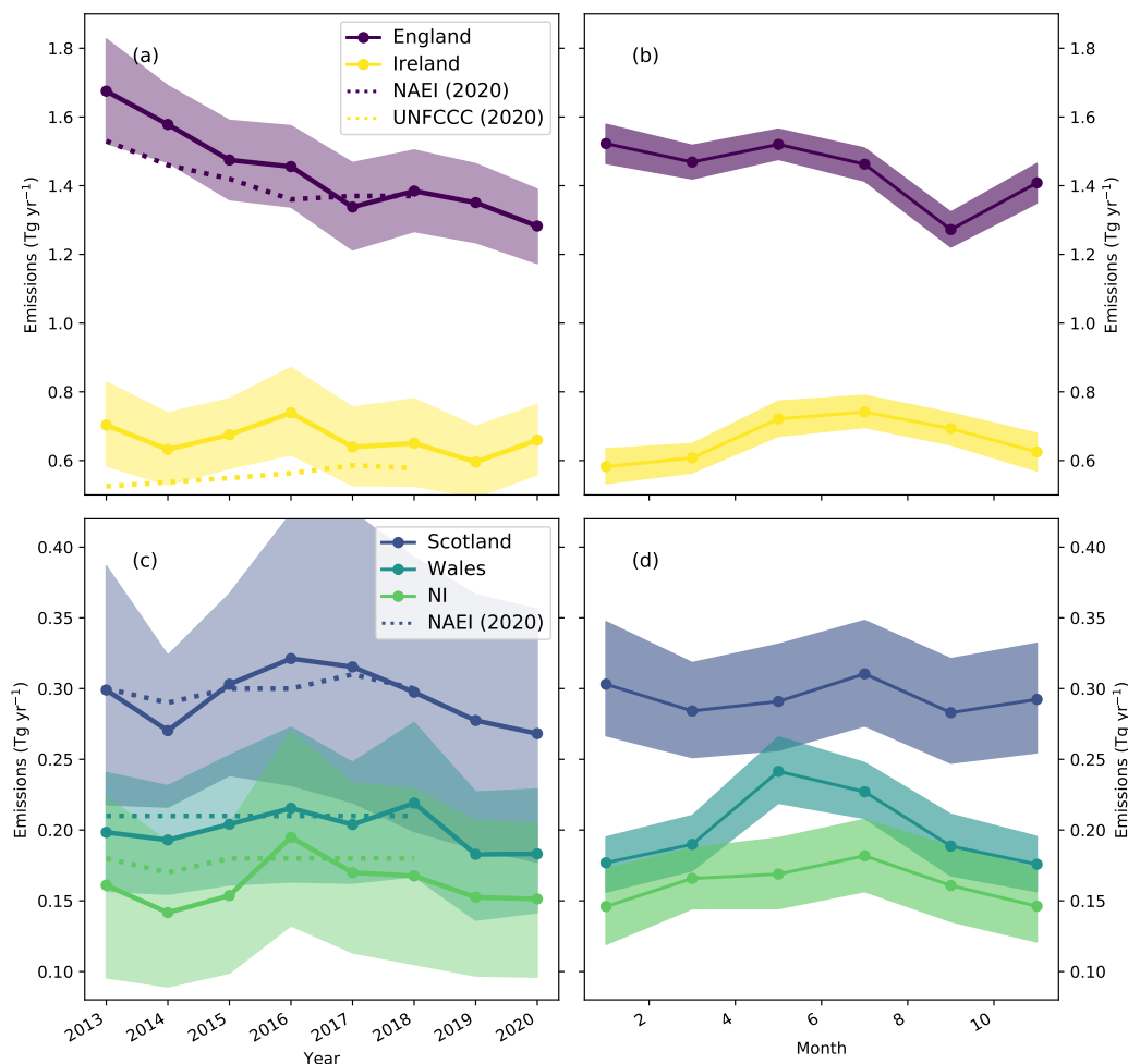
Figure 5. Annual emission estimates for the individual devolved administrations (DAs) of the UK and estimates for the Republic of Ireland. Showing: (a) the rw-mcmc annual mean estimates for England and Ireland; (b) the mean seasonal cycle for England and Ireland; (c) annual means for Scotland, Wales and Northern Ireland (NI); (d) the mean seasonal cycle for the respective DAs. The shading represents the 95% confidence interval. Dotted lines represent the DA NAEI estimates from the 2020 report.
