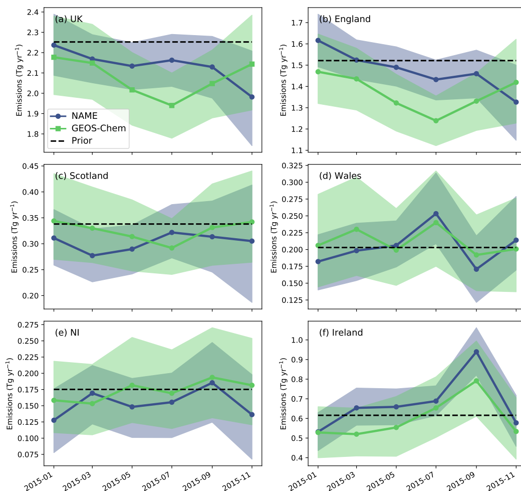
Figure 7. Two-monthly posterior estimates for 2015 from NAME (blue) and GEOS-Chem (green) inversions, and the prior used for the inversions (black dash). The panels show estimated emissions for (a) the UK, (b) England, (c) Scotland, (d) Wales, (e) NI and (f) Ireland. Shading represents the 95% confidence range of the inversion estimates.
