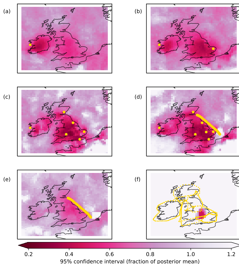
Figure 6. Posterior 95% confidence interval for 2015 as a fraction of the posterior estimate for each grid box. Darker colors indicate regions of lower uncertainty. Maps are shown for the following different measurement networks: (a) MHD, (b) MHD-TAC, (c) DECC network, (d) GAUGE network (DECC + GLA + Ferry), (e) Ferry, (f) FAAM aircraft (2014). Gold dots indicate locations of measurements used.
