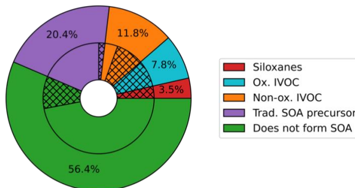
275 Figure 2. Percentage of the VCP emissions assigned to each category of CMAQ surrogates using the SAPRC07TIC_AE7I_VCP speciation profiles. The total rate of VCP emissions in Los Angeles County is 8.3 \times 10^7 \text{ kg yr}^{-1} . The outer ring depicts the percentage of total VCPy-derived emissions assigned to each of the three new VCP categories (siloxanes in red, oxygenated IVOCs in blue, and nonoxygenated IVOCs in orange), the traditional SOA precursors described by existing model surrogates (purple), and existing surrogates that do not form SOA (green). The inner ring gives an indication of the original assignments of each of the 280 outer ring categories. Hatching indicates emissions originally assigned to model surrogates that do not participate in model chemistry: IVOC, NVOL, and NROG. Solid colors represent other surrogate assignments.
