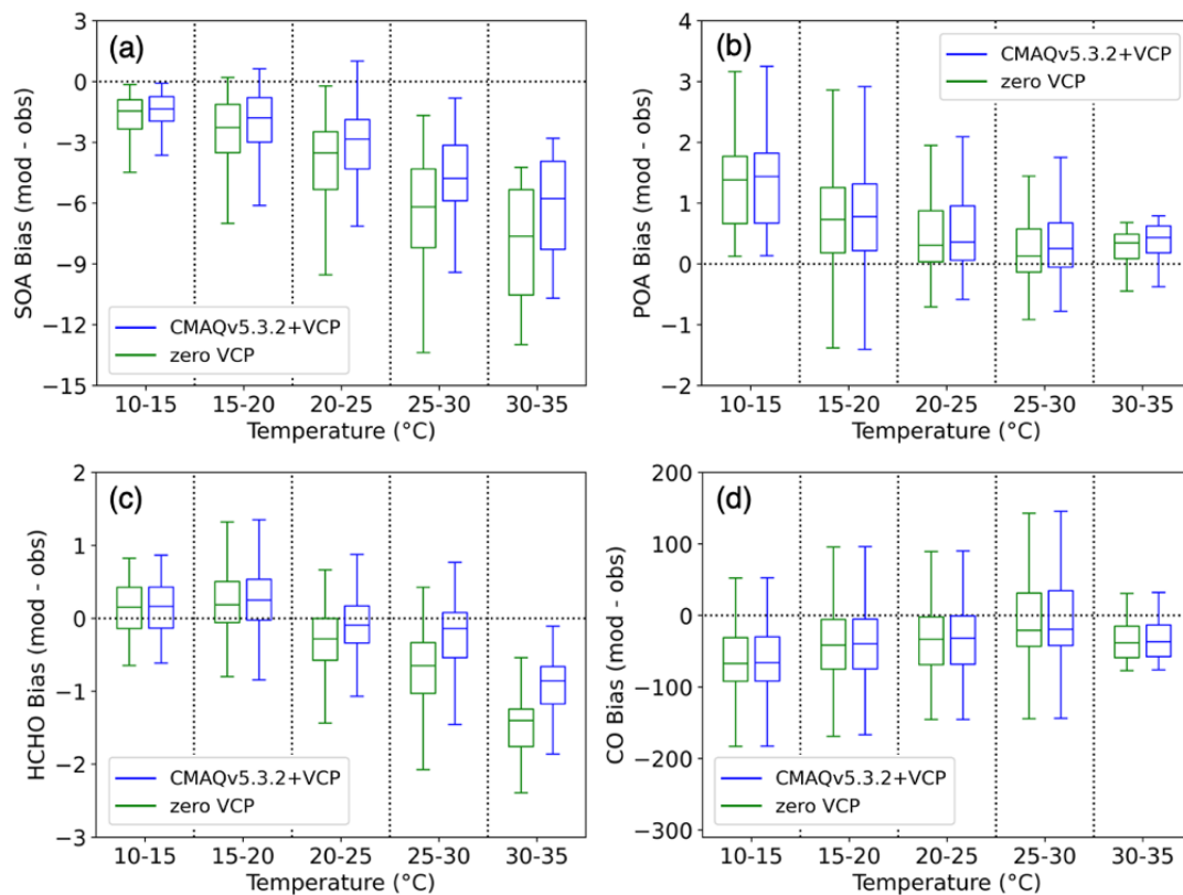
455 Figure 5. Bias (modeled - observed) of hourly concentrations vs. modeled temperature for the zero VCP case (green) and CMAQv5.3.2+VCP case (blue). Hourly concentrations are binned into five temperature ranges of 5°C each and the data in each bin is represented by a box-and-whisker plot. The horizontal midline depicts the median of the data, the edges of the box extend from the lower to upper quartile of the data, and the whiskers extend from the minimum to the maximum of the data. a) PM 1 SOA bias (µg m -3 ). b) PM 1 POA bias (µg m -3 ). c) Formaldehyde (HCHO) bias (ppb). d) CO bias (ppb).
