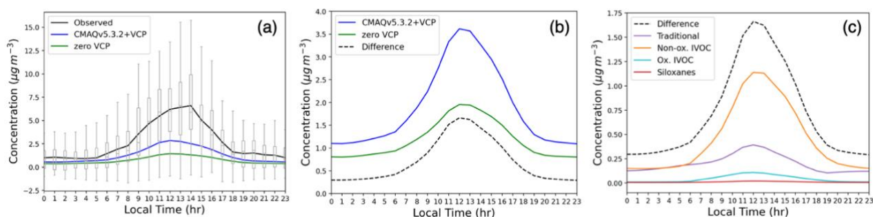
Figure 3. a) Average hourly concentrations of background-corrected PM_1 SOA observed and simulated by the zero VCP and CMAQv5.3.2+VCP modeling cases May 15-June 15. Box and whiskers show all hourly concentrations observed by AMS at the 315 CalNex site. A constant background value was removed from all observed concentrations according to the method in Hayes et al. (2015). The background value of each simulation was determined by averaging the lower 50% of hourly concentrations from 00:00 LT to 04:00 LT and subtracting that from each curve. b) Average hourly concentration of total (not size-resolved) SOA for the two simulation cases and their difference (CMAQv5.3.2+VCP – zero VCP). c) Difference in hourly concentrations of total SOA by category.
