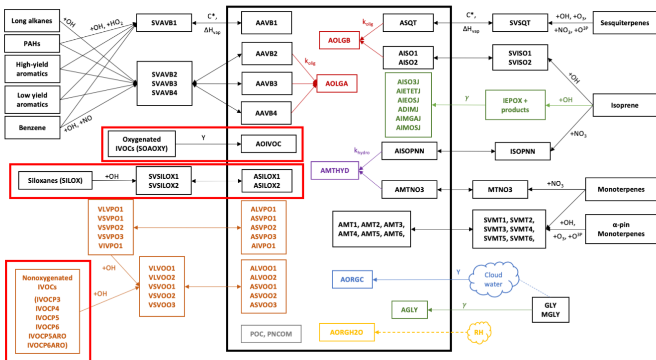
220 Figure 1. Treatment of OA chemistry in the CMAQv5.3.2+VCP model. The thick black box surrounds all aerosol-phase species. All smaller black boxes depict species undergoing gas-phase oxidation from VOCs to semivolatile or nonvolatile SOA species. Orange font depicts the VBS model for S/IVOCs. Red font depicts particle-phase accretion reactions while purple font depicts particle-phase hydrolysis reactions. Green font represents heterogeneous processes. Blue font shows cloud-processed aerosol and yellow font shows aerosol water associated with the organic phase. Gray boxes are nonvolatile primary organic aerosol (POA) species. Double-sided arrows represent reversible processes and one-sided arrows represent irreversible processes. Dashed lines represent processes that are dependent on relative humidity. The diagram includes the AERO7 mechanism plus the three VCP- 225 forming pathways specific to this work (thick boxes in red). See AE7I Species Table (2016/2021) for species descriptions.
