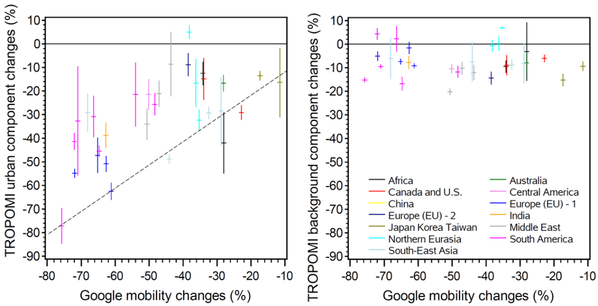
Figure 15. A scatter plot of Google mobility statistic changes vs. TROPOMI NO 2 VCD changes for (left) the urban and (right) background components during the period from March 16 to June 15, 2020 compared to the baseline period. The Google mobility statistic changes show the difference with the pre-lockdown period (Jan 3 – Feb 6, 2020) in percent. For TROPOMI, the difference is between the 2020 and the 2018-2019 average. Each symbol represents one country; the dot colour demonstrates the region as shown in the legend. Only countries with at least two cities used in this study are included in this plot. The correlation coefficient between the two data sets is 0.62. The dashed Y=X line is shown for reference. The error bars represent the standard errors.
