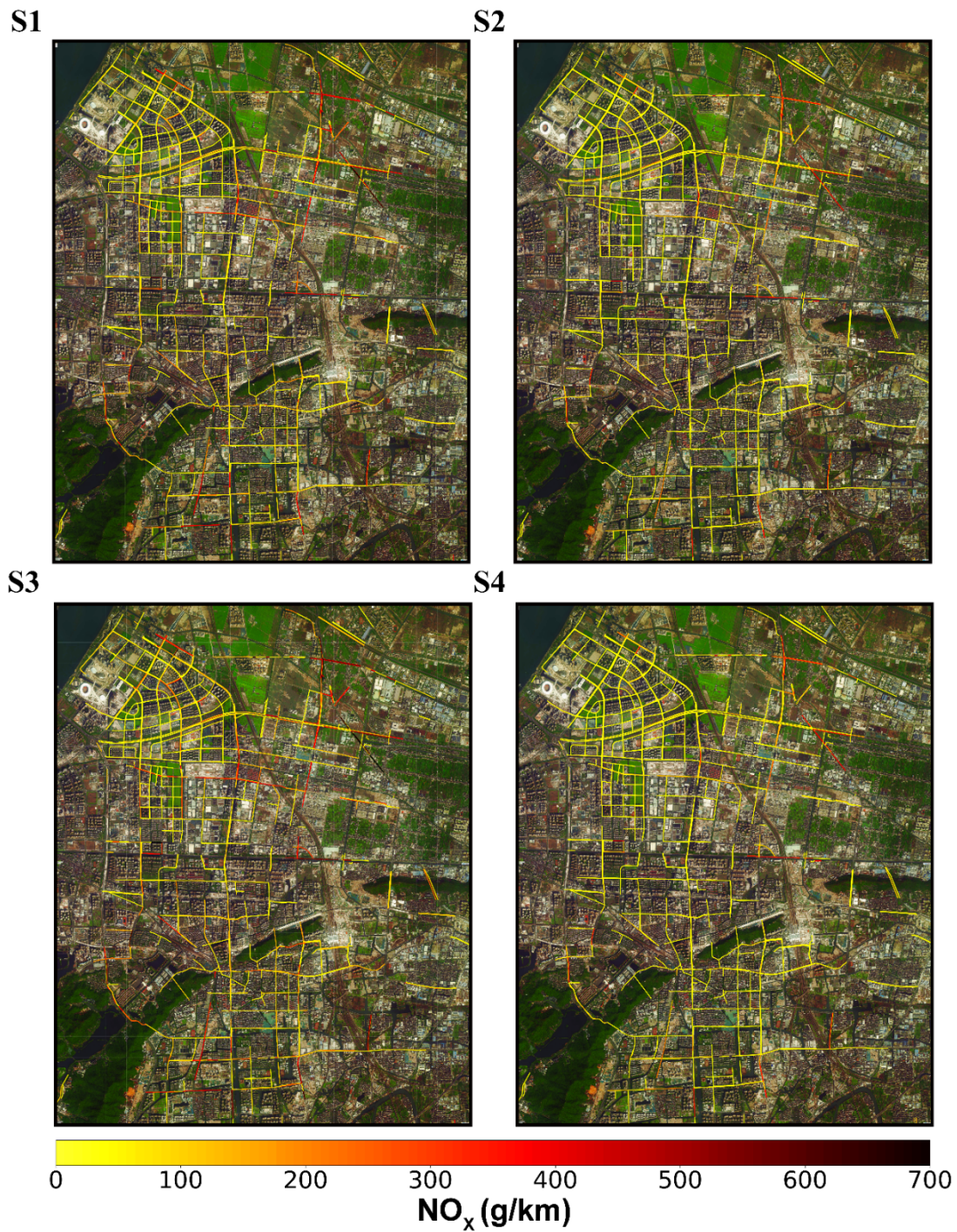
Figure 7. Impacts of traffic control strategies (i.e., S1, ~ S4) on daily average on-road vehicle NO x emissions. Map data © 2021, Gaode Map.
