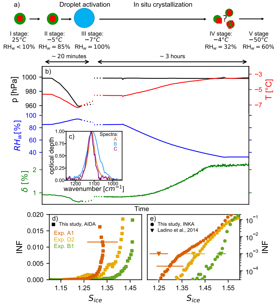
Figure 7. In-situ crystallization process—Liquid cloud processing, re-crystallization, and ice nucleation results (experiment type D). a) Schematic of the phase state and possible morphology of the particles after the in situ crystallization process. b) Time series of pressure (black line), temperature (red line), relative humidity with respect to water (blue line), and backscattering linear depolarization ratio (green line) during the in situ crystallization for experiment D2. The left part of the plot shows the short expansion run started at -5 °C and RH_w = 85\% to activate the seed aerosol particles to homogeneously mixed, aqueous droplets. After refilling of the AIDA chamber to ambient pressure (not shown in the figure), the relative humidity was reduced to RH_w = 32\% to induce the AS efflorescence. c) Normalized infrared spectra in the regime of the \nu_3 ( \text{SO}_4^{2-} ) mode obtained after transfer of the particles into the AIDA chamber (spectrum B) and after the in situ crystallization (spectrum C) in comparison with a reference spectrum of pure AS crystals (spectrum A). d) and e) Ice nucleating fraction as function of S_{ice} for the AIDA and INKA experiments with pure AS crystals (experiment A1, orange symbols), unprocessed AS crystals with thick SOM coating (experiment B1, green symbols), and in situ crystallized mixed AS/SOM particles (experiment D2, yellow symbols). Ice onset results from Ladino et al. (2014) are reported in panel e) as triangles: pure AS in orange, mixed AS/SOM particles in yellow, and pure SOA particles in green.
