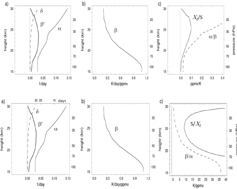
180 Figure 1. Vertical profiles of parameters used in the theoretical model calculations. (a) \alpha , \beta' and \delta , b) \beta and c) (S/X_2/S) and (\beta/\alpha/\beta) . The top axis in (a) shows the associated time scales in days.
