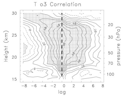
245 Figure 4. Correlation of deseasonalized SHADOZ ozone and temperature time series as a function of height and time lag (in months). Positive lag denotes temperature leading ozone-leading-temperature .
