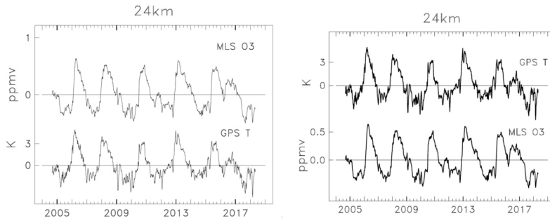
Figure 6. Time series of zonal average GPS temperatures and MLS ozone and GPS temperature at 24 km, for averages over 10° N-S.
