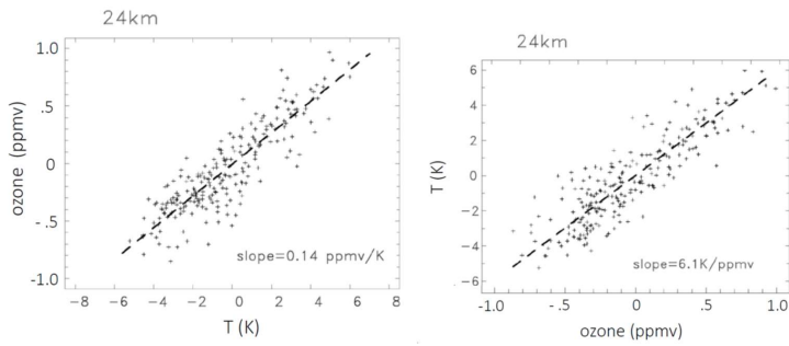
Figure 5. Scatter plot of deseasonalized temperature vs. ozone and-temperature anomalies from SHADOZ data at 24 km (data as in Fig. 3).
