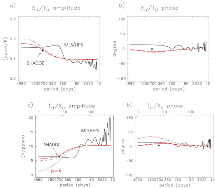
Figure 8. (a) (T_\sigma/X_\sigma/T_\sigma) ratio at 24 km as a function of wave period. Black line shows observational results from MLS/GPS satellite data, and red lines show idealized model calculations (solid red line includes ozone damping, and -dashed red line is for \delta=0 , and dotted red line is for \beta=0 ). The (T_\sigma/X_\sigma/T_\sigma) ratio derived from deseasonalized SHADOZ data at 24 km (Fig. 5) is also shown, which is mainly associated with the QBO (~28 months period). (b) corresponding (T_\sigma/X_\sigma/T_\sigma) phase differences.
