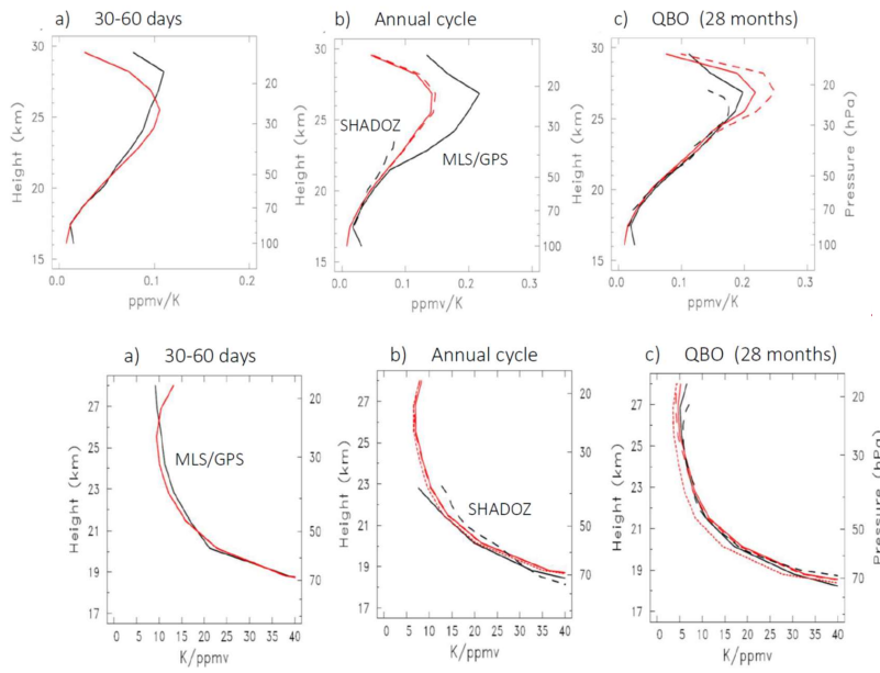
Figure 9. Vertical profiles of (T_{\sigma}/X_{\sigma}/T_{\sigma}) amplitude for selected frequency bands. (a) 30-60 day periods, (b) annual cycle (12 months period), (c) QBO period (~28 months). The solid black lines are results from MLS/GPS satellite data, and red lines show idealized model calculations (solid red line includes ozone damping, and dashed red lines is for \delta=0 , and dotted red lines for \beta=0 ). Additionally, results from SHADOZ ozone and temperature data are included as dashed black lines in (b-c), as described in text. Observations for the annual cycle (b) are only shown over altitudes 19-23 km where the annual cycle is relatively large and distinct. Note the horizontal axes change among the three panels.
